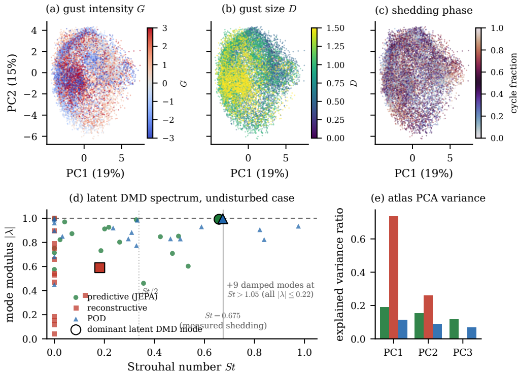
Figure 11. The physics the latent state holds. Top: two-dimensional projections of the predictive coefficient latent coloured by gust strength, core diameter, and shedding phase, showing a parametric manifold that coheres with the release parameters. Bottom: the latent dynamic-mode-decomposition spectrum, modulus against Strouhal number, by family; the predictive and linear latents place a marginally stable mode at the measured shedding frequency while the Fukami-lineage reconstruction is damped and off-frequency.
