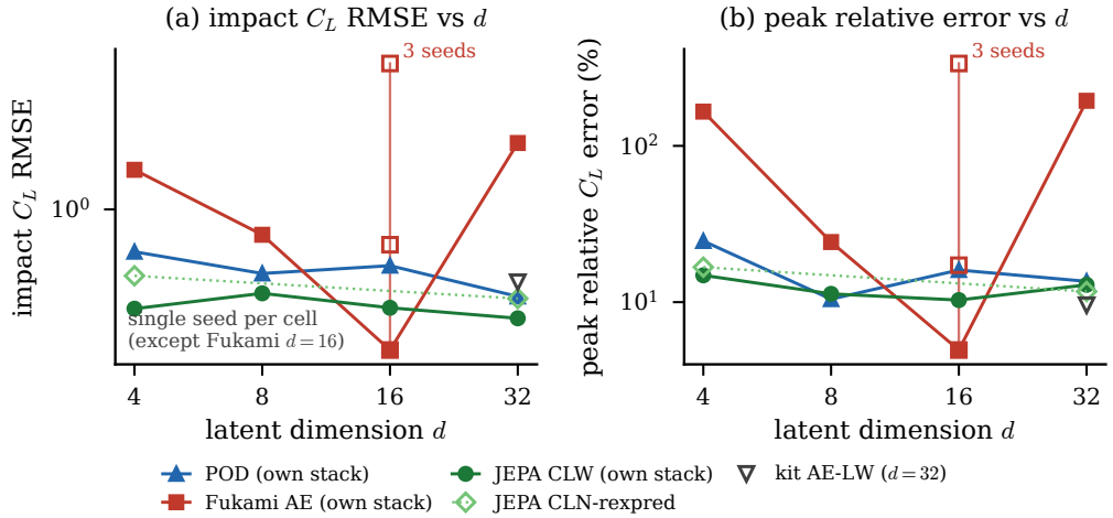
Figure 20. The assimilation-versus-dimension grid (in-distribution test set, per-family end-to-end stacks, K = 8 , every-frame pressure; single seed per cell except the reconstructive d = 16 cell, which carries three): impact error and relative peak error against dimension for the three families. The predictive family is uniform, the linear basis stable, the reconstructive baseline non-monotonic in dimension and irreproducible across seeds.
