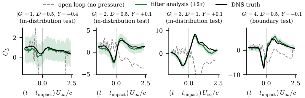
Figure 17. C_L estimation before and after impact across the gust-intensity envelope, on the wake-supervised predictive state ( d = 32 ) under the two-stage filter of §3.3.3: inside the impact window the members are advanced by the direct multi-horizon forecaster’s median forecast with its quantile band as state-dependent process noise (production scale c = 1.77 , validation-calibrated) and corrected by the encoded pressure observation; outside it, by the matched transformer with the tap-space update. Eight wall-pressure taps, N = 64 members; the lift probe that produces the plotted read-out never enters the innovation. Band: \pm 2 ensemble standard deviations; grey, the same stage-scheduled forecast models rolled deterministically without pressure. One representative encounter per |G| stratum (median impact closure on the frozen two-stage filter records; in-distribution test set for |G| \leq 3 , boundary test set at |G| = 4 , where this filter posts no large-error encounter). The analysis tracks the lift through impact and relaxation at every intensity; the open loop loses the transient.
