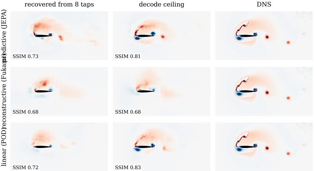
Figure 25. Flow recovered from eight wall-pressure taps on the representative held-out encounter of figure 16, at the impact-side frame, one row per family. Columns: the field decoded from the pressure-recovered coefficient state, the decode ceiling (the same decoder applied to the encoded state, no pressure step), and the simulation; per-panel structural similarity annotated. The comparison is within each row, since the decoders’ ceilings differ (§5.3); the ceiling-to-recovered gap is the cost of the pressure step.
