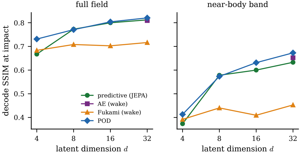
Figure 9. Decode SSIM at the impact instant against latent dimension d (full field and near-body band, in-distribution test set, decode floor). The compact nonlinear states and the linear basis improve with d and saturate together; only the published-recipe lineage plateaus lower. Field decode is not the discriminator at any dimension. Single encoder/decoder seed.
