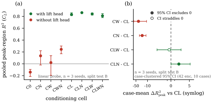
Figure 22. Paired peak-region lift R^2 per conditioning-cube cell (left) and case-mean deltas against the lift-only cell CL (right, symmetric-log axis, 95 % case-clustered bootstrap intervals over the 42 in-distribution test encounters of 10 cases); filled markers mark intervals that exclude zero. The near-body lift-focused predictive state cell (CLN) is the unique positive increment; the no- L cells sit one to two orders of magnitude lower.
