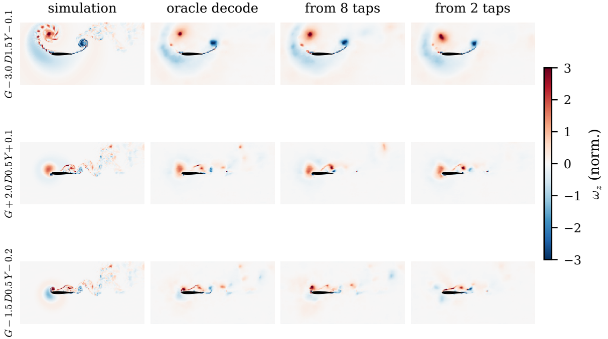
Figure 14: Flow recovered from sparse wall pressure on three held-out encounters (rows, labelled by (G, D, Y) ). Columns: the simulation, the oracle decode (the visualisation decoder applied to the simulation-encoded latent), and the decode of the latent estimated from K = 8 and K = 2 TCSI pressure taps. From eight taps the predictive latent recovers the leading-edge vortex and shear layer close to the oracle; two taps capture the gross impingement. The decoder is blurry by design (§4.6).
