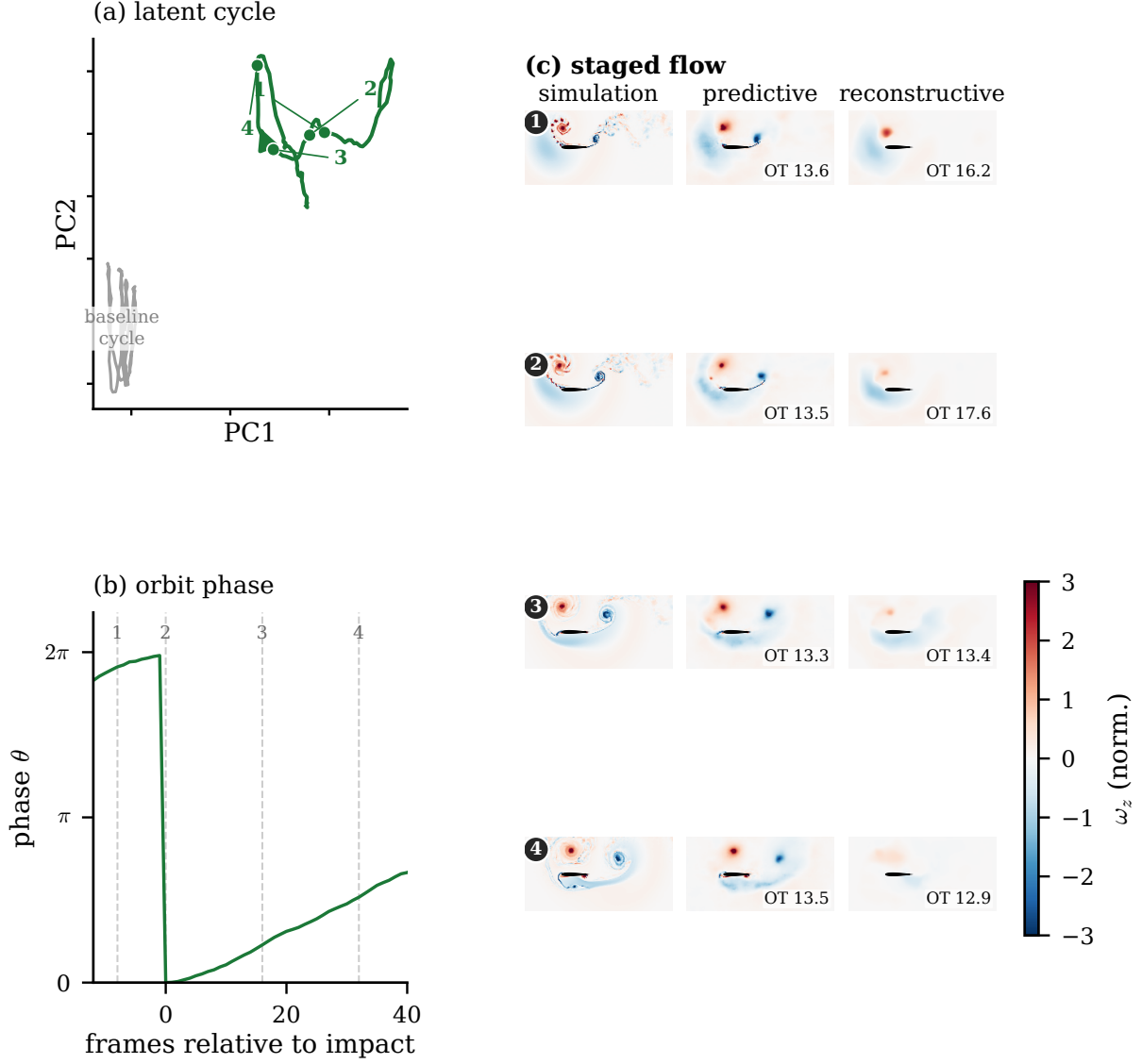
Figure 8: The gust encounter as a single closed cycle in the predictive latent, for a strong negative gust (G, D, Y) = (-3.0, 1.5, -0.1) . (a) The latent trajectory in the leading two baseline principal components departs the no-gust limit cycle (grey), executes the leading-edge-vortex growth and shedding, and returns; numbered glyphs mark the four stages and the arrow gives the direction of travel. (b) The orbit phase relative to the impact frame. (c) Mid-plane vorticity at the four stages (rows) for the simulation, the predictive decode, and the reconstructive decode (columns); the predictive decode localises the impingement while the reconstructive decode collapses, with the optimal-transport field distance between each decode and the simulation annotated at each stage (largest for the reconstructive decode near impact). The stage glyphs are those of Figure 5.
