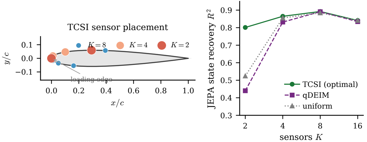
Figure 12: Sparse-sensor placement. (a) The target-conditioned (TCSI) taps for K=2, 4, 8 on the NACA 0012 surface; they cluster near the leading edge on both surfaces. (b) Predictive-state recovery (held-out test_b R^2 ) versus sensor count for TCSI, qDEIM, and uniform placement: optimal placement is decisive at K=2 and the methods converge by K \geq 4 .
