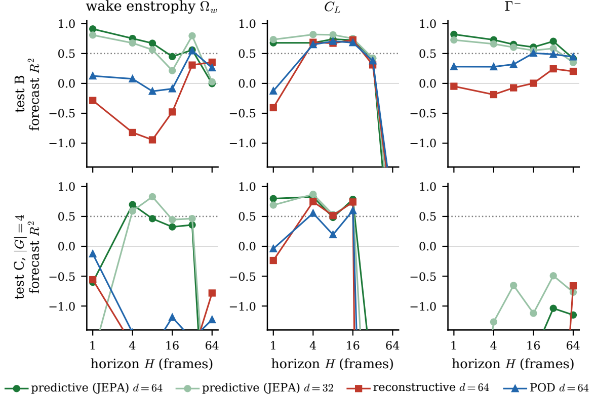
Figure 6: Held-out forecast closure ( R^2 of the Markov rollout) versus horizon H for the wake-entropy, C_L , and negative-circulation observables, on the in-distribution test_b (top) and the |G| = 4 extrapolation test_c (bottom), for the predictive latent at d = 64 and d = 32 , the reconstructive autoencoder, and POD. The dotted line marks R^2 = 0.5 . The predictive latent holds wake-entropy above the floor to H = 16 ; the reconstructive and linear latents are already below it at H = 1 .
