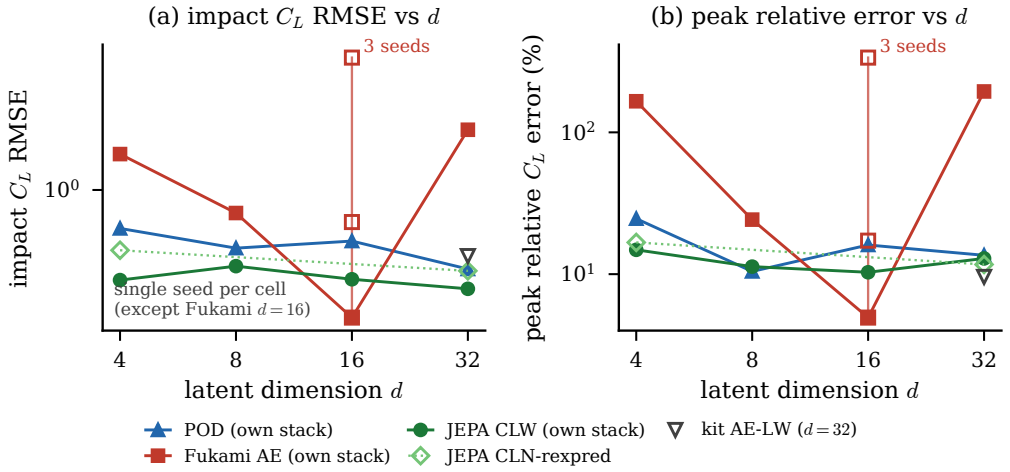
Figure 13. The assimilation-versus-dimension grid (in-distribution test set, per-family end-to-end stacks, K = 8 , every-frame pressure; single seed per cell except the reconstructive d = 16 cell, which carries three): impact error and relative peak error against dimension for the three families. The predictive family is uniform, the linear basis stable, the reconstructive baseline non-monotonic in dimension and irreproducible across seeds.
