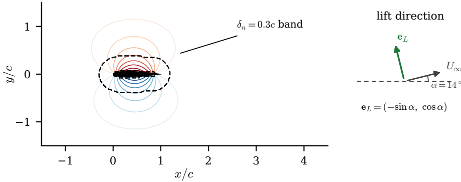
Figure 19. The Chang auxiliary potential \phi_L of equation (3.1) on the cache grid (contours), the feathered \delta_n = 0.3c supervision band (dashed) and the airfoil footprint; the inset shows the lift direction \mathbf{e}_L against the inclined freestream at \alpha = 14^\circ .
