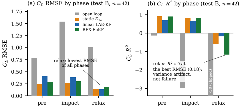
Figure 12. Phase-resolved lift tracking on the in-distribution test set ( n = 42 encounters, K = 8 taps, delay 10, N = 64 members, every-frame pressure). Lift error per phase in physical units (a) and in R^2 (b) at the val-calibrated band: the relaxation R^2 collapse is a variance artifact, the physical error the honest phase metric. The estimator ladder, its noise calibration and the fixed-lag smoother are in appendix C (figure 27).
