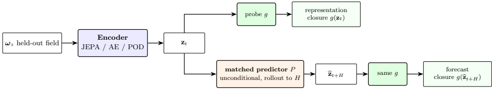
The predictor (unconditional, no gust parameters) and probe family g use the same architecture and protocol, trained separately for each encoder family.
