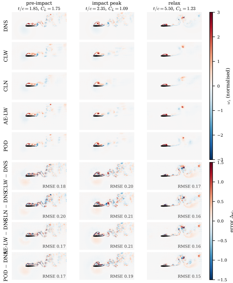
Figure 20. Decode floor on a representative held-out in-distribution test encounter (one decoder seed per model): DNS, the wake-supervised predictive state, the lift-focused predictive state, the wake autoencoder and the linear basis, and the error rows at three phases. Identical-capacity frozen decoders; normalised vorticity at the fixed \pm 3 range. All four states render the field faithfully, including the linear basis: field decode is not where the states separate.
