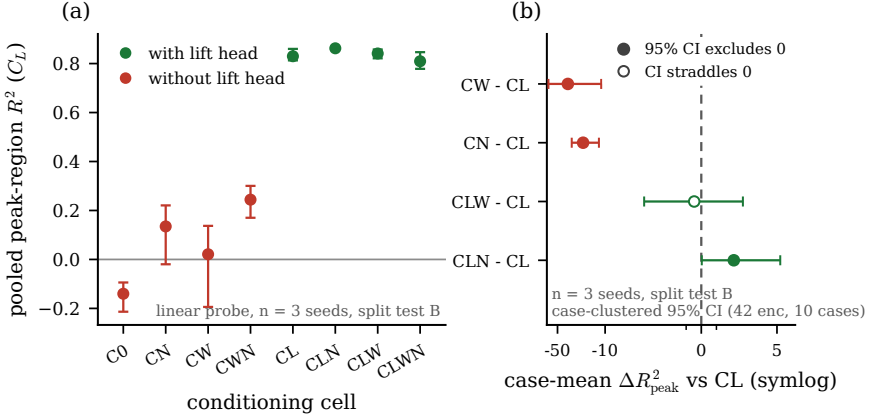
Figure 15. Paired peak-region lift R^2 per conditioning-cube cell (left) and case-mean deltas against the lift-only cell CL (right, symmetric-log axis, 95 % case-clustered bootstrap intervals over the 42 in-distribution test encounters of 10 cases); filled markers mark intervals that exclude zero. The near-body lift-focused predictive state cell (CLN) is the unique positive increment; the no- L cells sit one to two orders of magnitude lower.
