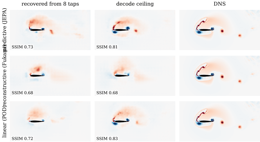
Figure 23. Flow recovered from eight wall-pressure taps on the representative held-out encounter of figure 10, at the impact-side frame, one row per family. Columns: the field decoded from the pressure-recovered coefficient state, the decode ceiling (the same decoder applied to the encoded state, no pressure step), and the simulation; per-panel structural similarity annotated. The comparison is within each row, since the decoders’ ceilings differ (§5.3); the ceiling-to-recovered gap is the cost of the pressure step.
