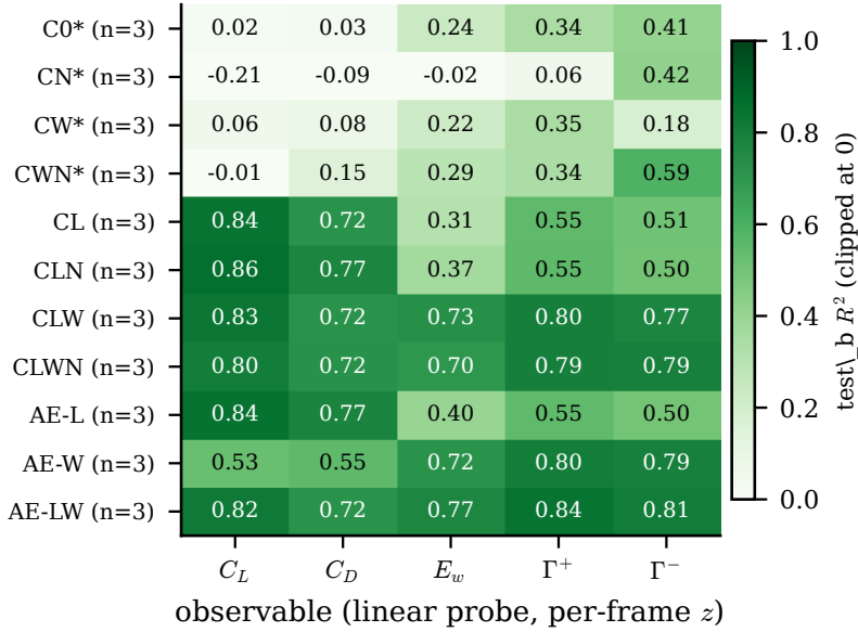
Figure 17. Task-dependent readability (in-distribution test set, linear probes on the per-frame state, seed mean over three encoder seeds per cell): lift and drag follow the L head, the wake block ( E_w , \Gamma^\pm ) follows the W head or the reconstruction objective, and collapsed cells (asterisks) read nothing linearly.
