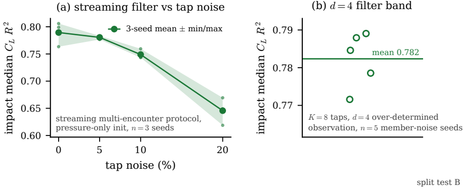
Figure 24. Deployment realism (in-distribution test set): (a) streaming multi-encounter filter against tap noise, three member-noise seeds, validation-selected band (no test-set reference); (b) the d = 4 filter band over five member-noise seeds.
