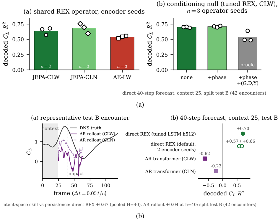
Figure 7. Forecasting the state on the in-distribution test set. (a) Decoded lift R^2 of the shared direct multi-horizon forecaster per family (three operator seeds each, bars at the seed mean) and the conditioning null (three seeds per arm): the (G, D, Y) oracle degrades the forecast, the phase covariate is a wash. (b) Direct versus autoregressive over forty steps through the impact from a 25-frame context: the one-shot forecast stays usable where the rollout compounds.
