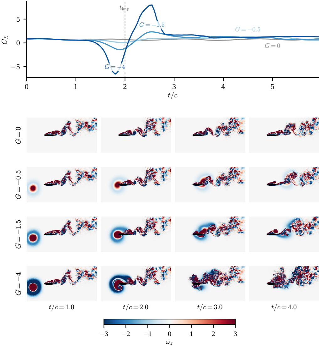
Figure 1. The vortex gust as a wake-reorganisation event: a gust-strength sweep at fixed core diameter D = 0.5 and offset Y = -0.1 (first encounter of each case). (a) Lift coefficient C_L against convective time, with t/c = 0 the release and t_{\text{imp}} (dashed) the leading-edge crossing near t/c = 2 ; the load excursion deepens and widens with |G| , the baseline ( G = 0 ) in grey. (b) Mid-plane spanwise vorticity \omega_z per case (rows G = 0, -0.5, -1.5, -4 ) at four times (columns t/c = 1, 2, 3, 4 ), raw units, colourbar clipped at \pm 3 (intense cores saturate), airfoil filled. The strong gust reorganises the wake through impact while the weak cases barely perturb the shedding; G = -4 is the |G| = 4 extrapolation case, shown only for illustration. The release parameters alone do not fix where the wake sits afterwards, which is why the wake, not only C_L , is the endpoint a reduced state must carry.
