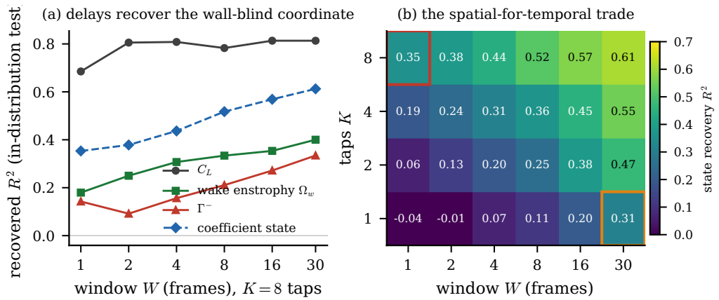
Figure 9. Sensors traded for delays. (a) Recovery of each observable from eight wall-pressure taps against the length of the pressure window (in-distribution test set); the wall-blind wake circulation rises with the window while the force, visible at one instant, does not. (b) Coefficient-state recovery over the tap-count by window-length grid, with the single-tap, thirty-frame cell and the reference eight-tap, single-frame cell outlined: a long window with few taps matches a short window with many.
