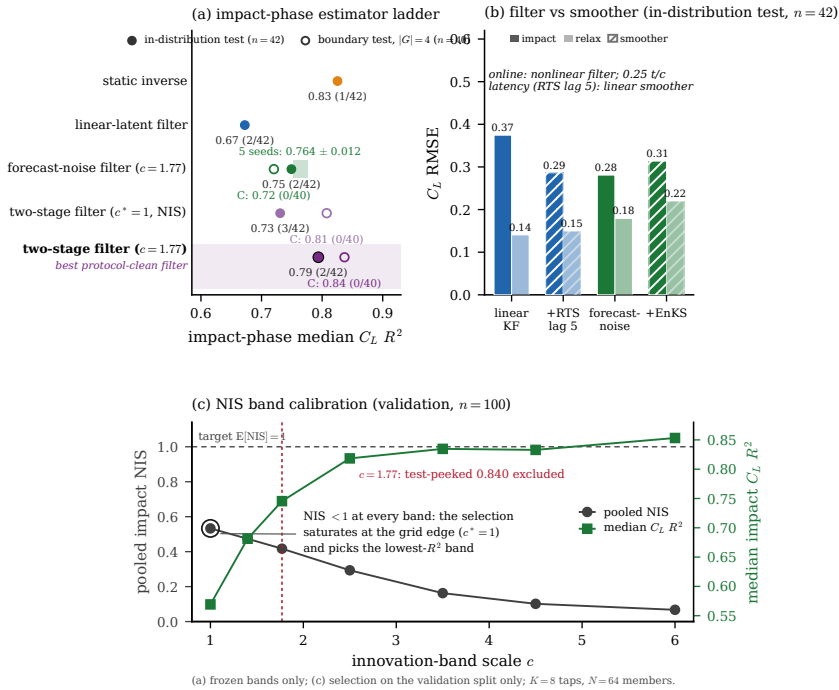
Figure 29. Estimator calibration and selection (in-distribution test, validation and, through the open markers, boundary test sets; parentetical counts on the ladder are large-error encounters, impact-phase R^2 < -1 , per set). (a) The impact-phase estimator ladder with the five-seed member-noise band, open markers the frozen boundary test values; (b) the filter against the fixed-lag smoother; (c) the band-scale calibration on the held-out training encounters, where innovation consistency and tracking disagree and the selection saturates at the grid edge.
