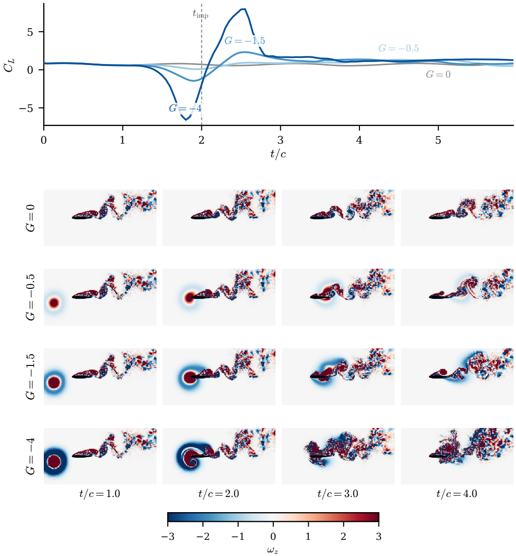
Figure 2. The vortex gust as a wake-reorganisation event: a gust-strength sweep at fixed core diameter D = 0.5 and offset Y = -0.1 (first encounter of each case). Top: lift coefficient C_L against convective time, with t/c = 0 the release and t_{\text{imp}} (dashed) the leading-edge crossing near t/c = 2 ; the load excursion deepens and widens with |G| , the baseline ( G = 0 ) in grey. Bottom: mid-plane spanwise vorticity \omega_z per case (rows G = 0, -0.5, -1.5, -4 ) at four times (columns t/c = 1, 2, 3, 4 ), raw units, colourbar clipped at \pm 3 (intense cores saturate), airfoil filled. The strong gust reorganises the wake through impact while the weak cases barely perturb the shedding; G = -4 is the |G| = 4 extrapolation case, shown only for illustration. The release parameters alone do not fix where the wake sits afterwards, which is why the wake, not only C_L , is the endpoint a reduced state must carry.
