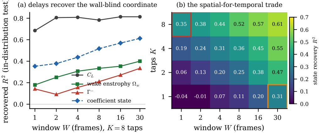
Figure 10. Sensors traded for delays. (a) Recovery of each observable from eight wall-pressure taps against the length of the pressure window (in-distribution test set); the wall-blind wake circulation rises with the window while the force, visible at one instant, does not. (b) Coefficient-state recovery over the tap-count by window-length grid, with the single-tap, thirty-frame cell and the reference eight-tap, single-frame cell outlined: a long window with few taps matches a short window with many.
