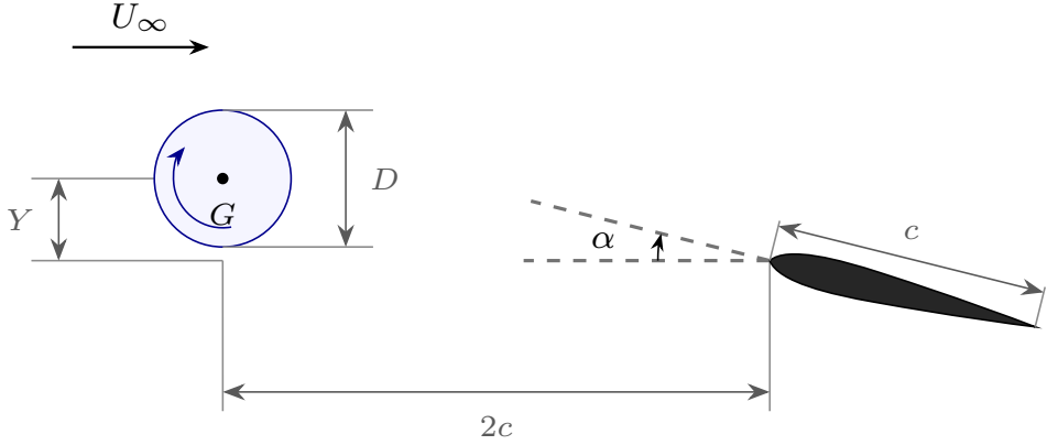
Figure 1. Case geometry (schematic, not to scale), drawn directly in the free-stream-aligned axes in which (G, D, Y) are defined, following Fukami et al. (2025). The vortex core is released a fixed 2c upstream of the leading edge (LE), offset by Y normal to the free stream U_\infty , and convects downstream parallel to it, not along the chord. The chord is pitched by the angle of attack \alpha = 14^\circ relative to these axes, trailing edge (TE) below leading edge. The core has diameter D = 2R/c (core radius R ) and peak azimuthal velocity u_{\theta,\max} setting the signed gust ratio G \equiv u_{\theta,\max}/u_\infty ; the arrow shows the clockwise sense of rotation for G > 0 . Only (G, D, Y) vary across cases.
