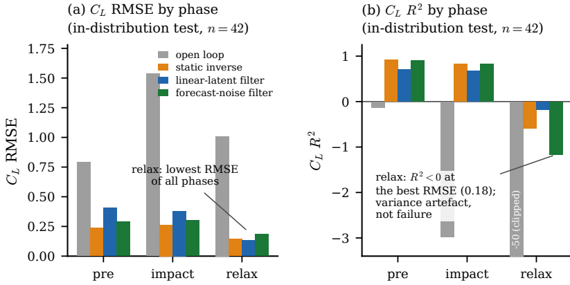
Figure 13. Phase-resolved lift tracking with the forecast-noise filter at the production coverage band on the in-distribution test set ( n = 42 encounters, K = 8 taps, delay 10, N = 64 members, every-frame pressure). Lift error per phase in physical units (a) and in R^2 (b) at the val-calibrated band: the relaxation R^2 collapse is a variance artefact, the physical error the honest phase metric. The estimator ladder, its noise calibration and the fixed-lag smoother are in appendix C (figure 30).
