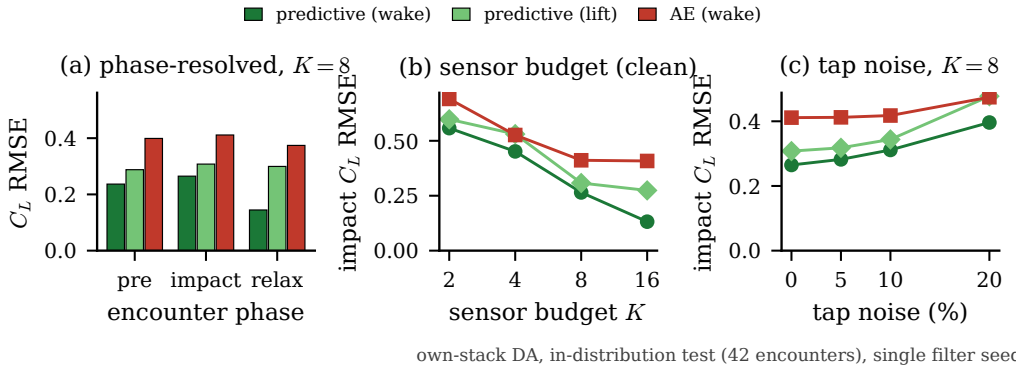
Figure 29. Per-family end-to-end comparison (in-distribution test set, 42 encounters, single filter seed): (a) phase-resolved lift error per family; (b) sensor-budget sweep on each family’s own nested placement; (c) tap-noise sweep at K = 8 .
