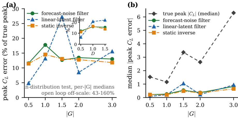
Figure 28. Relative peak error across the gust envelope (in-distribution test set, medians per |G| ): the forecast-derived filter stays near 12 to 14 per cent at all but the |G| = 1 stratum while the linear filter is non-uniform; the absolute peak error (right) grows with the peak itself.
