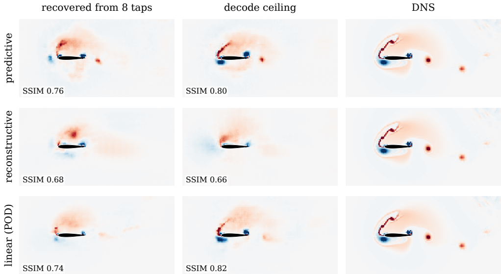
Figure 26. Flow recovered from eight wall-pressure taps on the representative held-out encounter of figure 11, at the impact-side frame, one row per family. Columns: the field decoded from the pressure-recovered coefficient state, the decode ceiling (the same decoder applied to the encoded state, no pressure step), and the simulation; per-panel structural similarity annotated. The comparison is within each row, since the decoders’ ceilings differ (§5.3); the ceiling-to-recovered gap is the cost of the pressure step.
