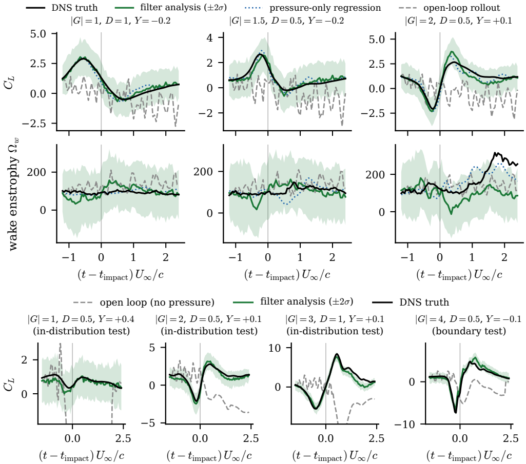
Figure 11. The estimator tracks the encounter from wall pressure alone. Top: representative held-out encounters at |G| = 1, 1.5 and 2 (columns), lift coefficient and wake enstrophy (rows); each panel shows the DNS truth, the filter analysis with its \pm 2\sigma ensemble band, the pressure-only regression, and the open-loop rollout, the vertical line marking impact. The filter follows the load through impact and relaxation where the open-loop forecast loses it and the pressure-only regression goes stale. Bottom: C_L estimation across the gust-intensity envelope on the wake-supervised predictive state ( d = 32 ) under the two-stage filter of §3.3.3 (one representative encounter per |G| stratum, in-distribution test set for |G| \leq 3 and boundary test set at |G| = 4 , where this filter posts no large-error encounter); inside the impact window the members are advanced by the direct multi-horizon forecaster's median with its quantile band as state-dependent process noise (production scale c = 1.77 , validation-calibrated) and corrected by the encoded pressure observation, outside it by the matched transformer with the tap-space update. Eight wall-pressure taps, N = 64 members; the lift probe producing the read-out never enters the innovation; grey is the same forecast run open loop.
