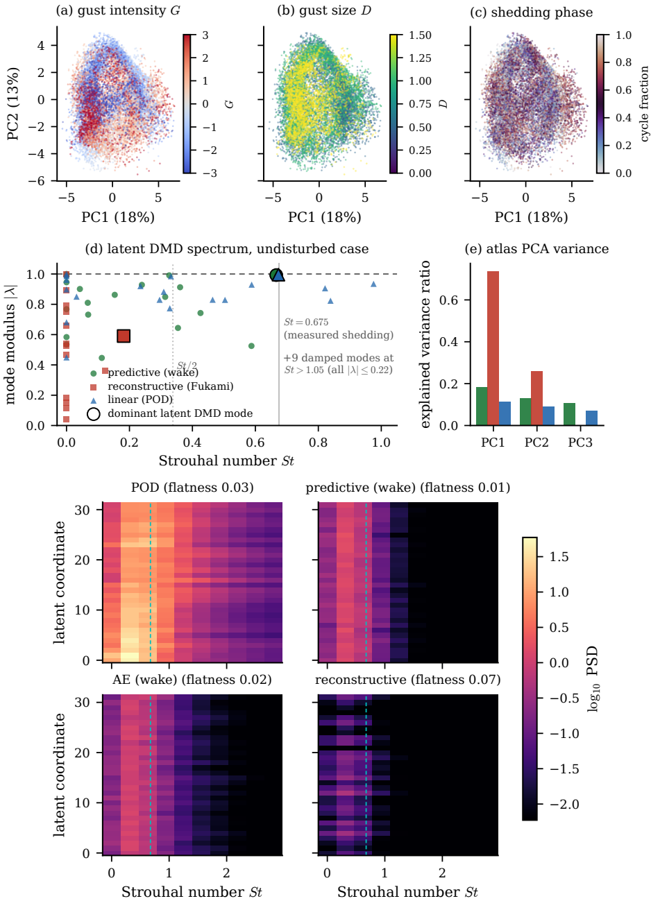
Figure 7. The physics the latent state holds. Top: two-dimensional projections of the predictive coefficient latent coloured by gust strength, core diameter and shedding phase, showing a parametric manifold that coheres with the release parameters, with the latent dynamic-mode-decomposition spectrum (modulus against Strouhal number, by family; the predictive and linear latents place a marginally stable mode at the measured shedding frequency while the Fukami-lineage reconstruction is damped and off-frequency), and the explained-variance ratio of the leading atlas principal components per family (e; colours as in d). Bottom: per-coordinate latent spectra by family (training encounters, d = 32 ; mean Welch power spectral density against Strouhal number, coordinates ordered by peak frequency, dashed line the shedding Strouhal): the predictive coordinates concentrate at the shedding line while the published-recipe reconstruction spreads energy across frequency and the matched-supervision autoencoder does not.
