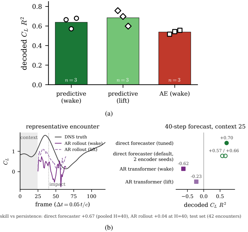
Figure 8. Forecasting the state on the in-distribution test set. (a) Decoded lift R^2 of the shared direct multi-horizon forecaster per family (three operator seeds each, bars at the seed mean): the predictive states forecast the lift best. (b) Direct versus autoregressive over forty steps through the impact from a 25-frame context: the one-shot forecast stays usable where the rollout compounds. The conditioning null, where the (G, D, Y) oracle degrades the forecast and the phase covariate is a wash, is figure 19 in appendix A.
