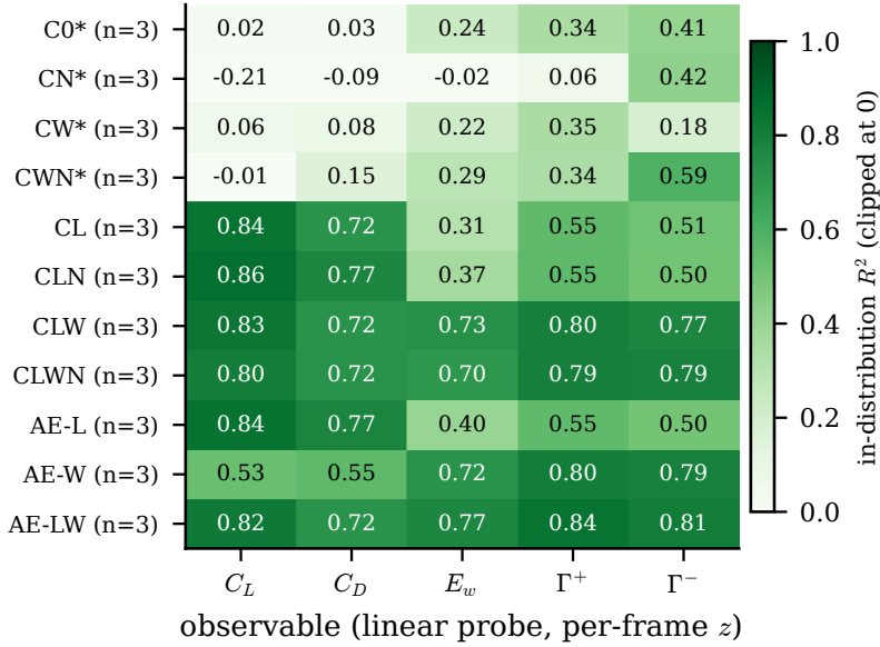
Figure 18. Task-dependent readability (in-distribution test set, linear probes on the per-frame state, seed mean over three encoder seeds per cell): lift and drag follow the L head, the wake block ( E_w , \Gamma^\pm ) follows the W head or the reconstruction objective, and collapsed cells (asterisks) read nothing linearly.
