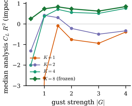
(b) the frozen filter needs its eight taps
