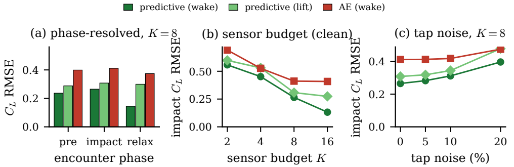
Figure 29. Per-family end-to-end comparison (in-distribution test set, 42 encounters, single filter seed): (a) phase-resolved lift error per family; (b) sensor-budget sweep on each family’s own nested placement; (c) tap-noise sweep at K = 8 .
