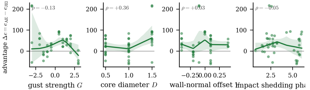
Figure 10. Per-encounter paired improvement \Delta e = e_{\text{AE}} - e_{\text{JEPA}} in held-out wake-entropy error against the gust strength G , core diameter D , wall-normal offset Y , and the baseline shedding phase at impact \phi (test_b, n = 42 ); positive \Delta e means the predictive latent carries the smaller error. Each panel shows the per-encounter values, a locally weighted (LOWESS) trend, and a bootstrap band over encounters. The predictive advantage grows with D (significant) but shows no significant G or Y trend; the shedding-phase axis falls into two clusters because impact is fixed near a single convective instant.
