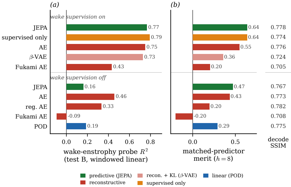
Figure 9. The attribution result of table 6, at a glance. (a) Held-out wake-entrrophy readability and (b) matched-predictor merit, with the models grouped by whether they carry the wake-supervision head; every wake-headed state reads the wake and every bare state collapses, whatever the training objective. The right-hand column lists the decode similarity, which barely separates the families.
