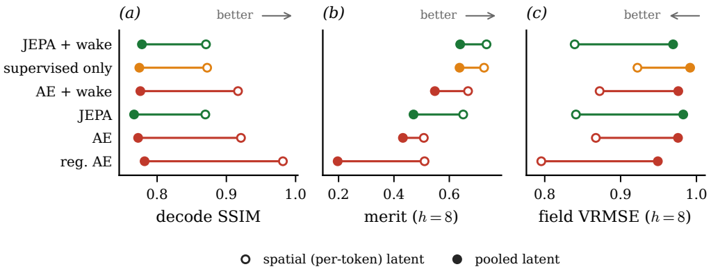
Figure 24. The decodability-versus-estimability trade of §5.3, quantified. Each panel connects the spatially resolved latent (open marker) to its pooled coefficient state (filled marker), per family, for the decode similarity, the matched-predictor merit, and the field forecast error. Pooling costs field fidelity in every family; the coefficient state is the price of a state a wall-pressure filter can track.
