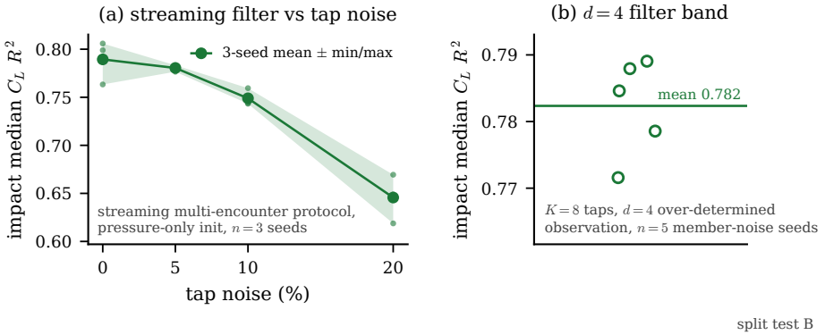
Figure 18. Deployment realism (test_b): (a) streaming multi-encounter filter against tap noise, three member-noise seeds, protocol-clean band; (b) the d=4 filter band over five member-noise seeds.
