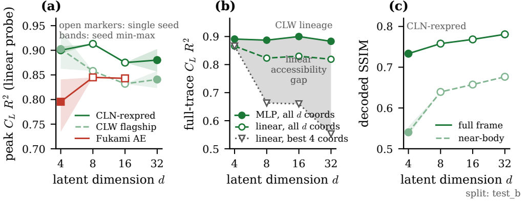
Figure 8. The dimension axis on test_b. (a) Peak-region lift R^2 (linear probe) against latent dimension for the three lineages; shaded bands are three-seed min-max ranges, open markers single seeds. (b) The probe-dilution control: a multilayer probe is flat in d while the best-four-coordinate linear probe falls, so the d = 4 advantage is linear accessibility of a distributed code, not information. (c) Decoded SSIM (Wang convention, §3.5) of the same lineage rises with d : the wake tier is not compressible.
