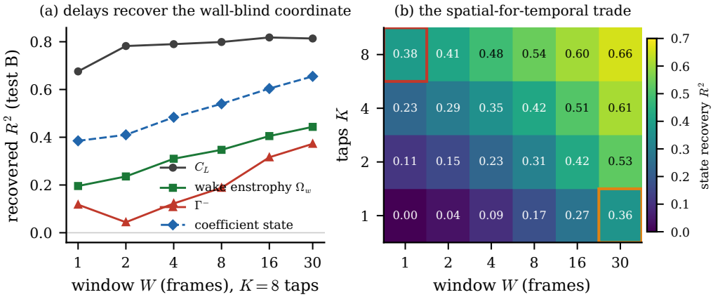
Figure 12. Sensors traded for delays. (a) Recovery of each observable from eight wall-pressure taps against the length of the pressure window (test_b); the wall-blind wake circulation rises with the window while the force, visible at one instant, does not. (b) Coefficient-state recovery over the tap-count by window-length grid, with the single-tap, thirty-frame cell and the reference eight-tap, single-frame cell outlined: a long window with few taps matches a short window with many.
