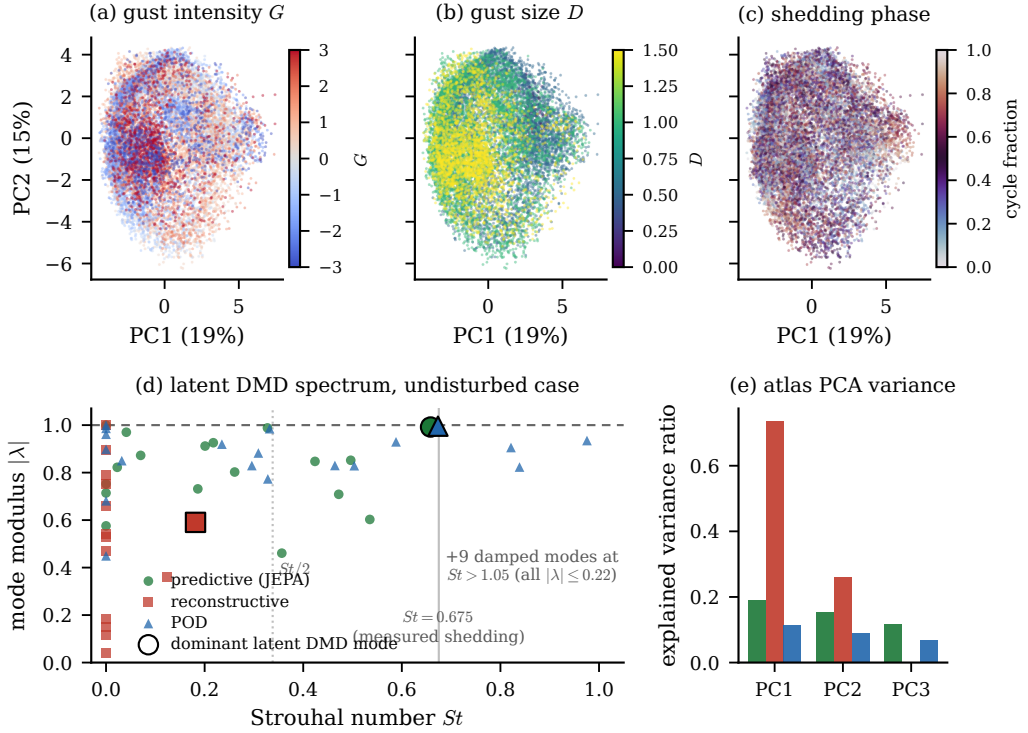
Figure 20. The physics the latent state holds. Top: two-dimensional projections of the predictive coefficient latent coloured by gust strength, core diameter, and shedding phase, showing a parametric manifold that coheres with the release parameters. Bottom: the latent dynamic-mode-decomposition spectrum, modulus against Strouhal number, by family; the predictive and linear latents place a marginally stable mode at the measured shedding frequency while the Fukami-lineage reconstruction is damped and off-frequency.
