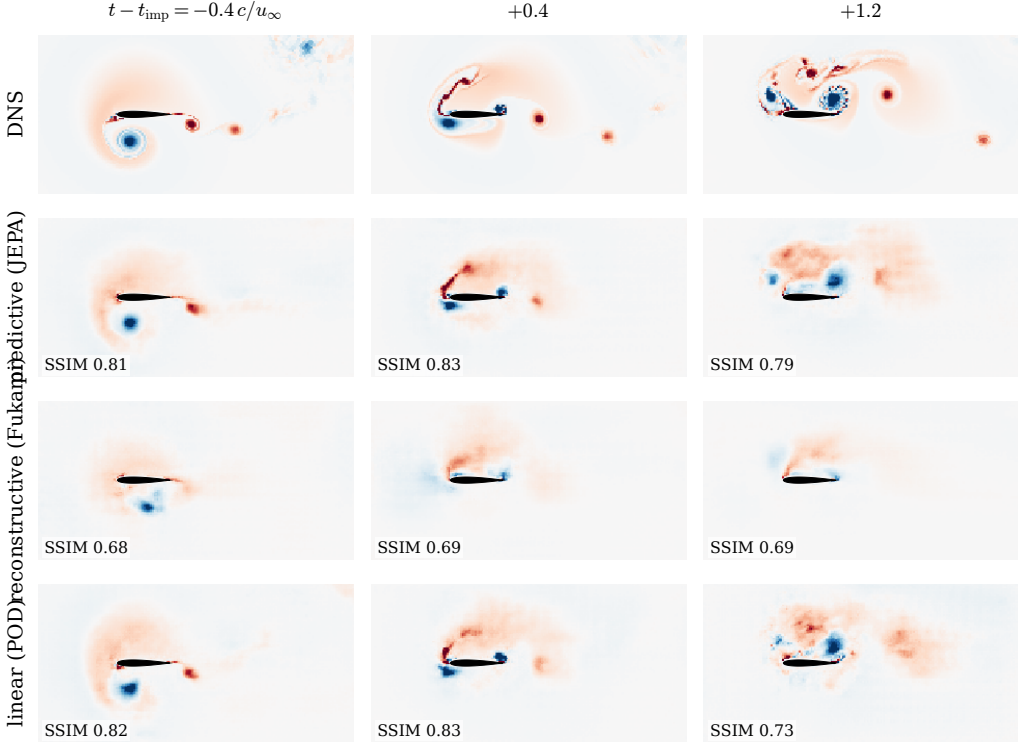
Figure 23. Decoded vorticity through the encounter on the representative held-out test_b case ( |G| = 1.5 , the same encounter as figure 13). Rows: the simulation and the fields decoded from the encoded coefficient state of the predictive, reconstructive, and linear families; columns: a pre-impact, an impact, and a relaxation frame. Each decode is produced by the same diagnostic decoder that defines the decode-floor similarity of table 6, trained on the frozen encoder; the per-panel structural similarity is annotated. The pooled decode is soft by construction (§5.3); the comparison is between rows at matched frames, and no family’s decode is part of any training loss.
