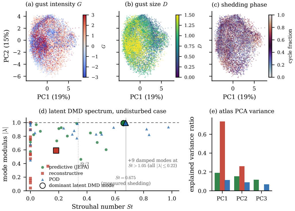
Figure 13. The physics the latent state holds. Top: two-dimensional projections of the predictive coefficient latent coloured by gust strength, core diameter, and shedding phase, showing a parametric manifold that coheres with the release parameters. Bottom: the latent dynamic-mode-decomposition spectrum, modulus against Strouhal number, by family; the predictive and linear latents place a marginally stable mode at the measured shedding frequency while the Fukami-lineage reconstruction is damped and off-frequency.
