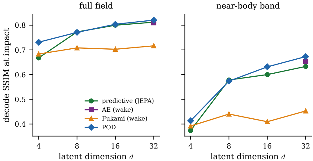
Figure 10. Decode SSIM at the impact instant against latent dimension d (full field and near-body band, in-distribution test set, decode floor). The compact nonlinear states and the linear basis improve with d and saturate together; only the published-recipe lineage plateaus lower. Field decode is not the discriminator at any dimension. Single encoder/decoder seed.
