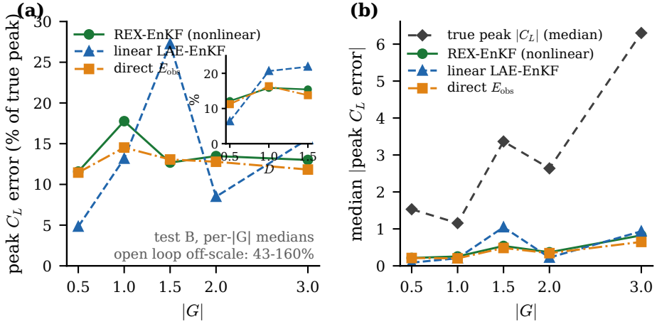
Figure 22. Relative peak error across the gust envelope (in-distribution test set, medians per |G| ): the forecast-derived filter is scale-invariant near 12 to 14 per cent while the linear filter is non-uniform; the absolute peak error (right) grows with the peak itself.
