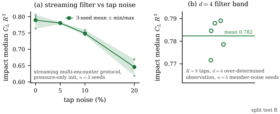
Figure 29. Deployment realism (in-distribution test set): (a) streaming multi-encounter filter against tap noise, three member-noise seeds, validation-selected band (no test-set reference); (b) the d = 4 filter band over five member-noise seeds.
