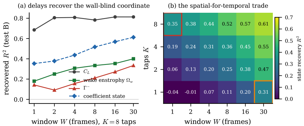
Figure 17. Sensors traded for delays. (a) Recovery of each observable from eight wall-pressure taps against the length of the pressure window (in-distribution test set); the wall-blind wake circulation rises with the window while the force, visible at one instant, does not. (b) Coefficient-state recovery over the tap-count by window-length grid, with the single-tap, thirty-frame cell and the reference eight-tap, single-frame cell outlined: a long window with few taps matches a short window with many.
