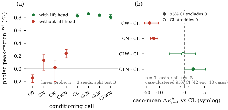
Figure 27. Paired peak-region lift R^2 per conditioning-cube cell (left) and case-mean deltas against the lift-only cell CL (right, symmetric-log axis, 95 % case-clustered bootstrap intervals over the 42 in-distribution test encounters of 10 cases); filled markers mark intervals that exclude zero. The near-body lift-focused predictive state cell (CLN) is the unique positive increment; the no- L cells sit one to two orders of magnitude lower.
