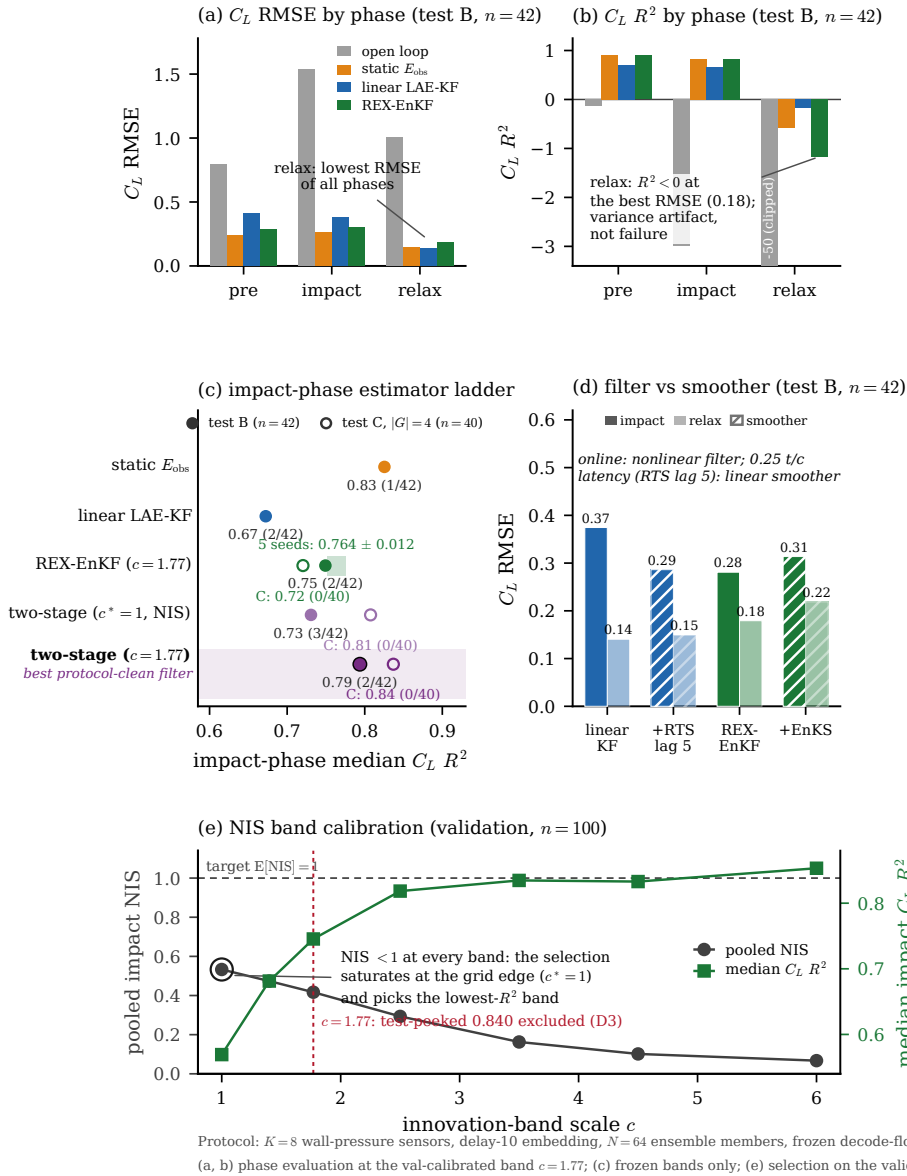
Figure 21. Phase-resolved assimilation on the in-distribution test set ( n = 42 encounters, K = 8 taps, delay 10, N = 64 members, every-frame pressure). (a,b) Lift error per phase in physical units and in R^2 at the val-calibrated band: the relaxation R^2 collapse is a variance artifact. (c) The impact-phase estimator ladder with the five-seed member-noise band; open markers are the frozen boundary test values. (d) Filter against fixed-lag smoother. (e) The band-scale calibration on the held-out training encounters: consistency and tracking disagree, and the selection saturates at the grid edge.
