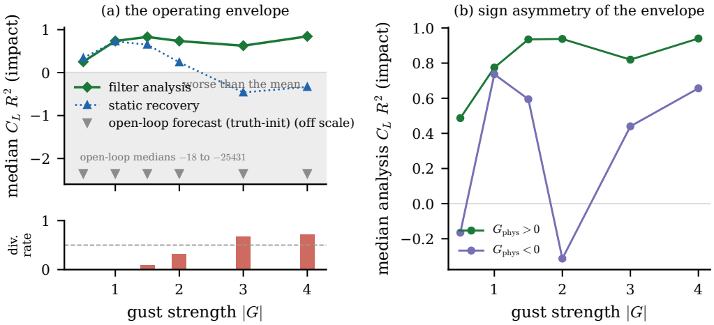
Figure 20. The gust-intensity operating envelope. (a) Median analysis lift closure ( R^2 , impact window) against gust strength for the frozen filter, the static single-frame recovery, and the truth-initialised open-loop forecast, with the filter divergence rate as the strip beneath; the shaded band marks closure worse than predicting the encounter mean, and the open-loop forecast lies off the scale below it. (b) The same filter closure resolved by the physical sign of the gust, showing the wider usable envelope of the positive gusts.
