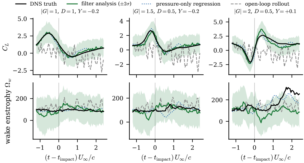
Figure 18. The estimator tracks the encounter from wall pressure alone. Columns are representative held-out encounters at |G| = 1, 1.5 and 2 ; rows are the lift coefficient and the wake enstrophy. Each panel shows the DNS truth, the filter analysis with its \pm 2\sigma ensemble band, the pressure-only regression, and the open-loop rollout; the vertical line marks impact. The filter follows the load through impact and relaxation where the open-loop forecast loses it and the pressure-only regression goes stale.
