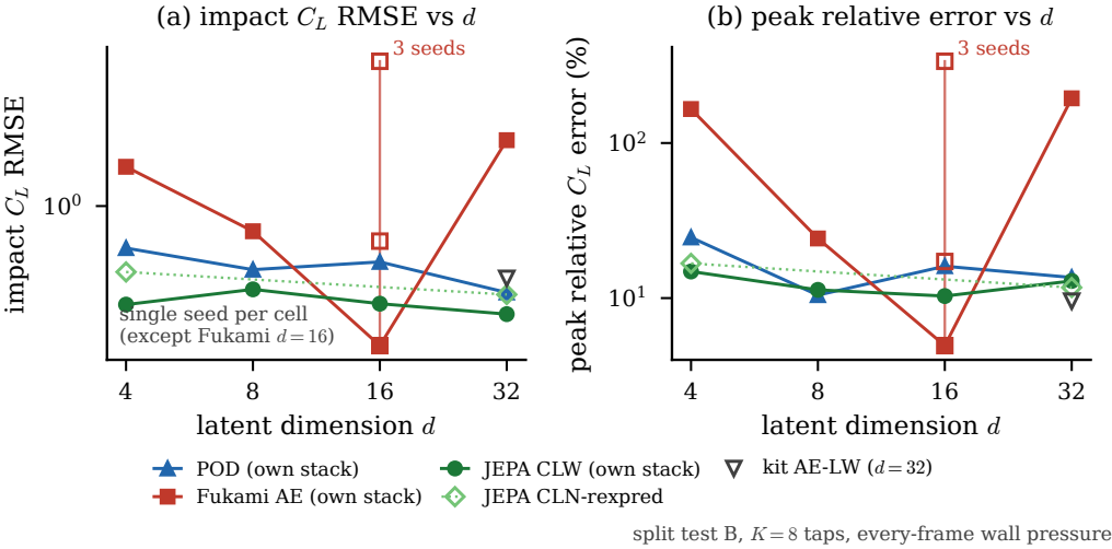
Figure 24. The assimilation-versus-dimension grid (in-distribution test set, per-family end-to-end stacks, K=8 , every-frame pressure; single seed per cell except the reconstructive d=16 cell, which carries three): impact error and relative peak error against dimension for the three families. The predictive family is uniform, the linear basis stable, the reconstructive baseline non-monotonic in dimension and irreproducible across seeds.
