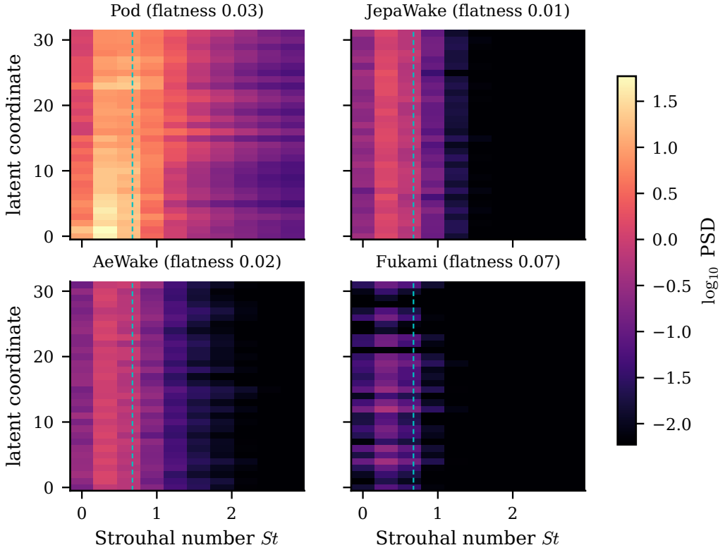
Figure 11. Per-coordinate latent spectra by family (training encounters, d = 32 ; mean Welch power spectral density against Strouhal number, coordinates ordered by peak frequency; the dashed line marks the shedding Strouhal). The predictive coordinates concentrate at the shedding line while the published-recipe reconstruction spreads energy across frequency, and the matched-supervision autoencoder does not.
