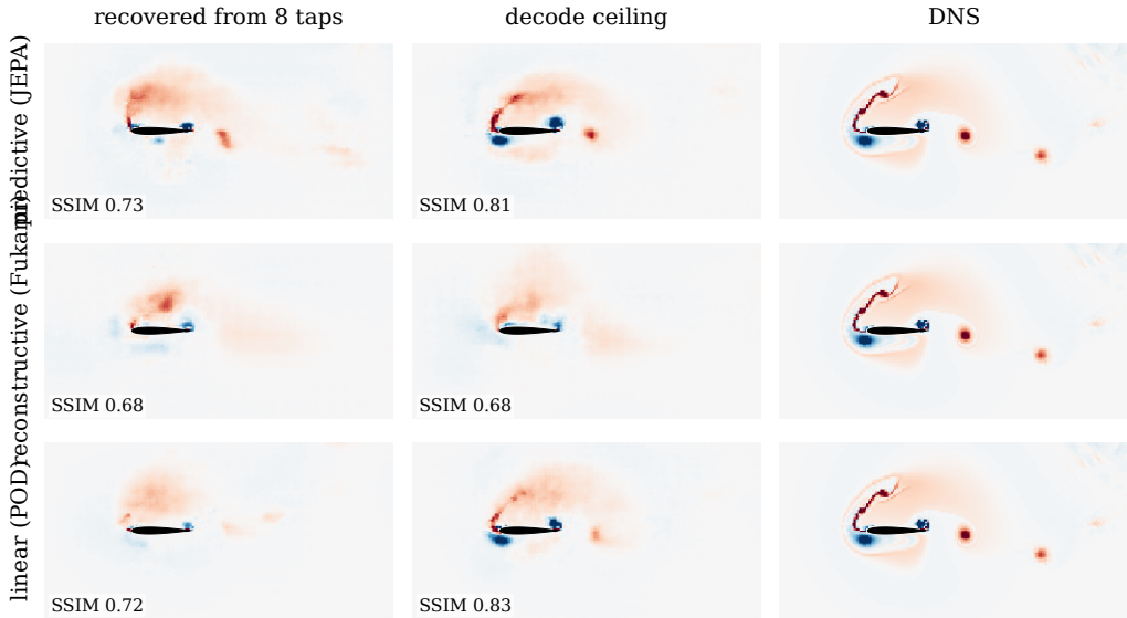
Figure 28. Flow recovered from eight wall-pressure taps on the representative held-out encounter of figure 18, at the impact-side frame, one row per family. Columns: the field decoded from the pressure-recovered coefficient state, the decode ceiling (the same decoder applied to the encoded state, no pressure step), and the simulation; per-panel structural similarity annotated. The comparison is within each row, since the decoders' ceilings differ (§5.3); the ceiling-to-recovered gap is the cost of the pressure step.
