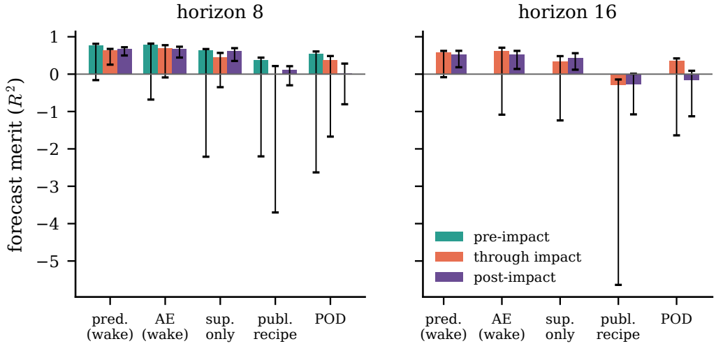
Figure 15. Shared-operator forecast merit split by phase (pre-impact, through-impact, post-impact), per family at horizons eight and sixteen (in-distribution test set, five observables, three operator seeds; bars at the seed mean, case-clustered 95 % intervals). Through-impact merit separates the families: the wake-supervised states hold, the published-recipe reconstruction collapses across the transient, and the linear basis fades into the relaxation.
