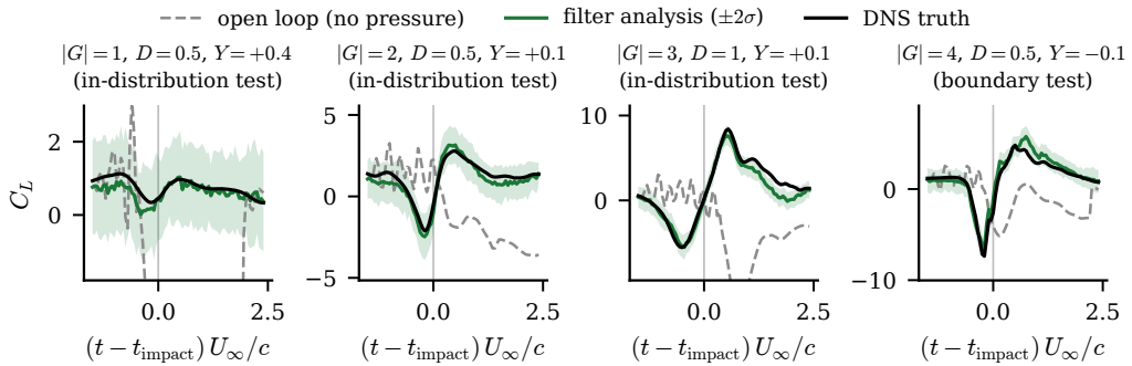
Figure 19. C_L estimation before and after impact across the gust-intensity envelope, on the wake-supervised predictive state ( d = 32 ) under the two-stage filter of §3.3.3: inside the impact window the members are advanced by the direct multi-horizon forecaster’s median forecast with its quantile band as state-dependent process noise (production scale c = 1.77 , validation-calibrated) and corrected by the encoded pressure observation; outside it, by the matched transformer with the tap-space update. Eight wall-pressure taps, N = 64 members; the lift probe that produces the plotted read-out never enters the innovation. Band: \pm 2 ensemble standard deviations; grey, the same stage-scheduled forecast models rolled deterministically without pressure. One representative encounter per |G| stratum (median impact closure on the frozen two-stage filter records; in-distribution test set for |G| \leq 3 , boundary test set at |G| = 4 , where this filter posts no divergent encounter). The analysis tracks the lift through impact and relaxation at every intensity; the open loop loses the transient.
