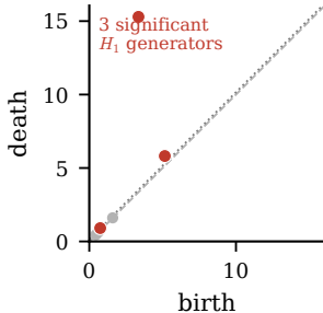
reconstructive encoding
