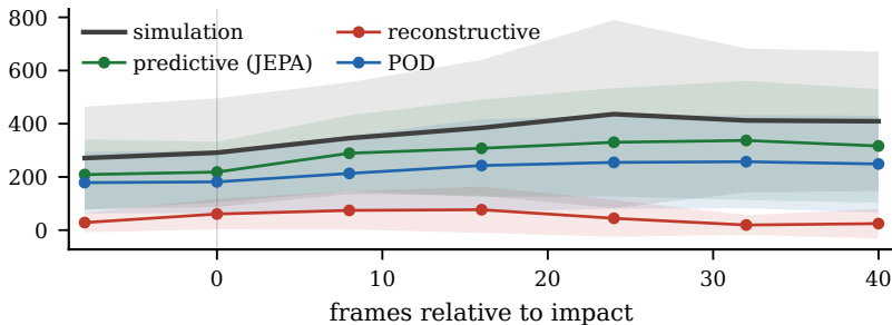
large-scale wake enstrophy
