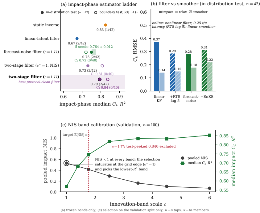
Figure 30. [APC-C1] Estimator calibration and selection (in-distribution test, validation and, through the open markers, boundary test sets; parenthetical counts on the ladder are large-error encounters, impact-phase R^2 < -1 , per set). (a) The impact-phase estimator ladder with the five-seed member-noise band, open markers the frozen boundary test values; (b) the filter against the fixed-lag smoother; (c) the band-scale calibration on the held-out training encounters, where innovation consistency and tracking disagree and the selection saturates at the grid edge.
