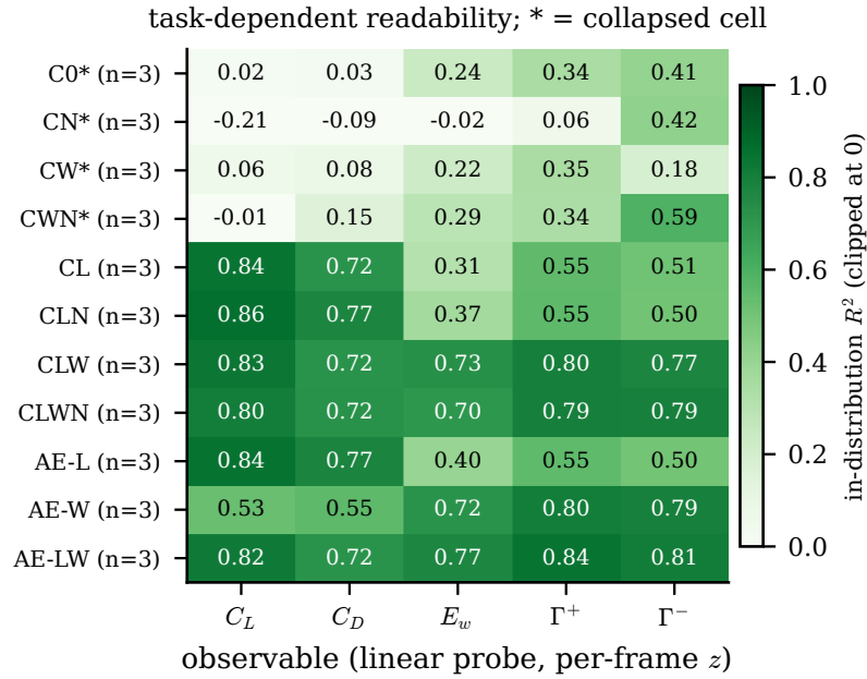
Figure 18. [APA-C6] Task-dependent readability (in-distribution test set, linear probes on the per-frame state, seed mean over three encoder seeds per cell): lift and drag follow the L head, the wake block ( E_w , \Gamma^\pm ) follows the W head or the reconstruction objective, and collapsed cells (asterisks) read nothing linearly.
