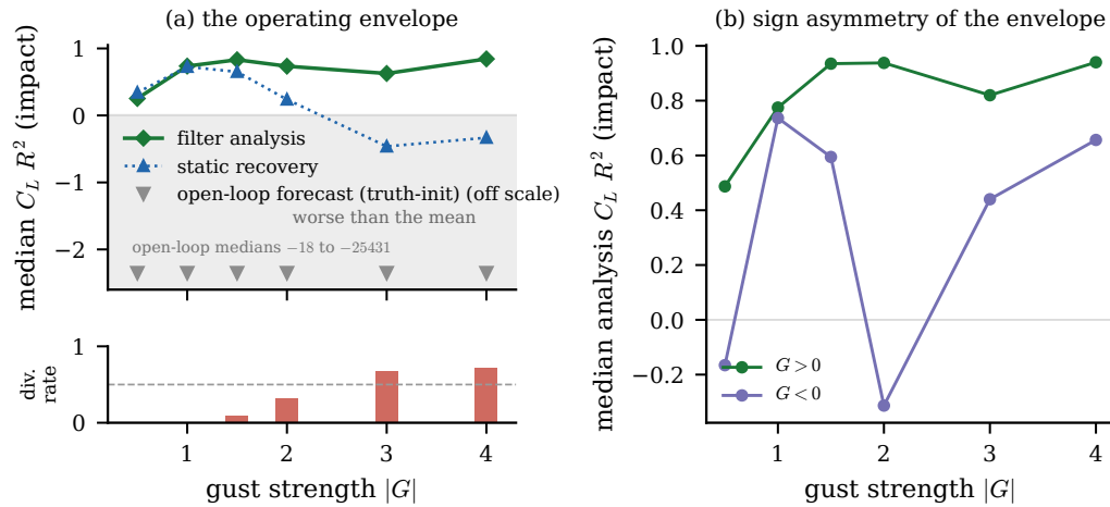
Figure 12. [S4-C5] The gust-intensity operating envelope, diagnosed with the base frozen filter (figure 13 carries the forecast-noise filter's phase-resolved errors). (a) Median analysis lift closure ( R^2 , impact window) against gust strength for the base filter, the static single-frame recovery, and the truth-initialised open-loop forecast, with the filter consistency-failure rate as the strip beneath; the shaded band marks closure worse than predicting the encounter mean, and the open-loop forecast lies off the scale below it. The base filter tracks the median throughout but becomes under-dispersed from a gust ratio of about three, where the consistency-failure rate climbs. (b) The same base-filter closure resolved by the physical sign of the gust, showing the wider usable envelope of the positive gusts.
