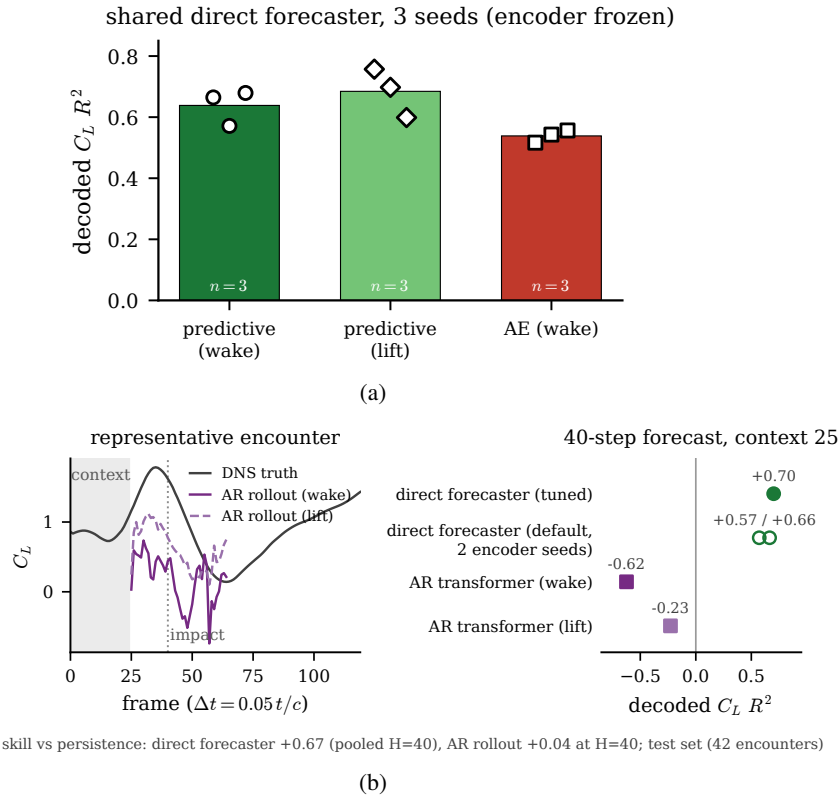
Figure 8. [S4C-C1] Forecasting the state on the in-distribution test set. (a) Decoded lift R^2 of the shared direct multi-horizon forecaster per family (three operator seeds each, the forecaster retrained on a frozen representation, bars at the seed mean): the predictive states forecast the lift best. (b) Direct versus autoregressive over forty steps through the impact from a 25-frame context: the one-shot forecast stays usable where the rollout compounds. The conditioning null, where the (G, D, Y) oracle degrades the forecast and the phase covariate is a wash, is figure 19 in appendix A.
