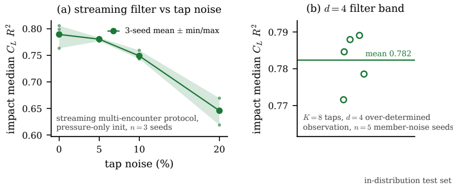
Figure 27. [APB-C2] Deployment realism (in-distribution test set): (a) streaming multi-encounter filter against tap noise, three member-noise seeds, validation-selected band (no test-set reference); (b) the d = 4 filter band over five member-noise seeds.
