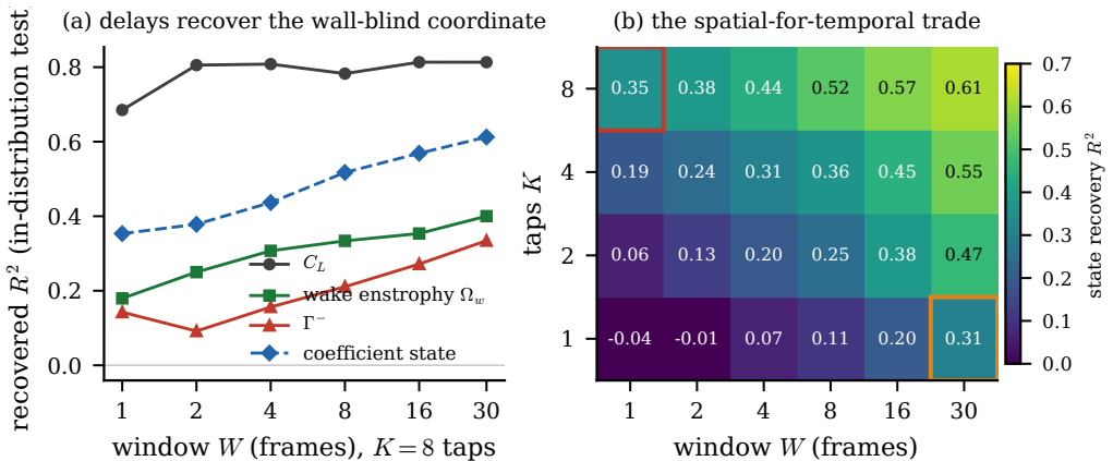
Figure 10. [S4-C3] Sensors traded for delays. (a) Recovery of each observable from eight wall-pressure taps against the length of the pressure window (in-distribution test set); the wall-blind wake circulation rises with the window while the force, visible at one instant, does not. (b) Coefficient-state recovery over the tap-count by window-length grid, with the single-tap, thirty-frame cell and the reference eight-tap, single-frame cell outlined: a long window with few taps matches a short window with many.
