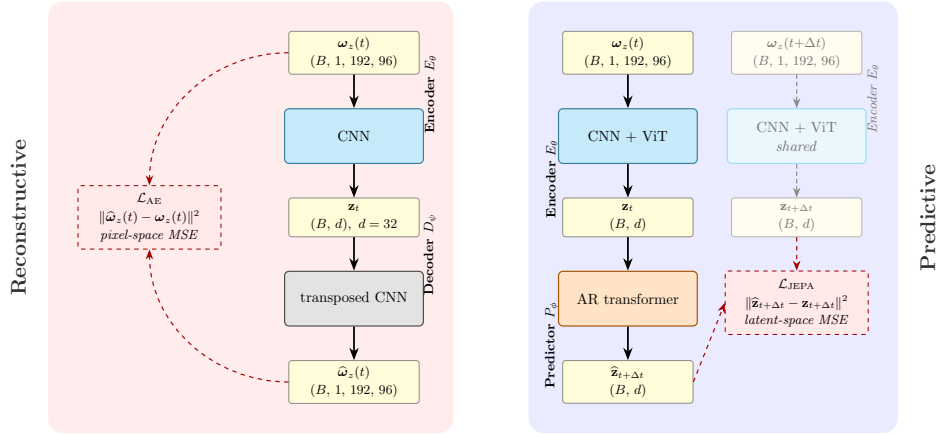
Figure 15. [APA-C1] Predictive versus reconstructive training. Left: the reconstructive autoencoder encodes the field at t , decodes it, and incurs a field-space error. Right: the predictive model encodes the fields at t and t + \Delta t with shared weights and incurs a latent-space error between the predicted and observed target embeddings, with no field-space loss and no decoder during training. This is the contrast the matched-predictor protocol of §3.2 evaluates; the visualisation decoder is trained only afterwards, on the frozen encoder.
