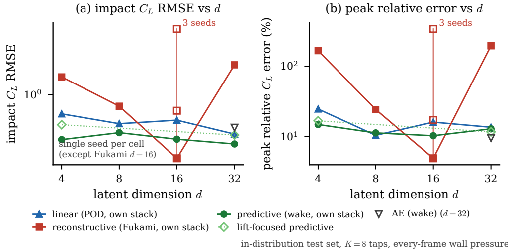
Figure 14. [S4D-C2] The assimilation-versus-dimension grid (in-distribution test set, per-family end-to-end stacks, K = 8 , every-frame pressure; single seed per cell except the reconstructive d = 16 cell, which carries three): impact error and relative peak error against dimension for the three families. The predictive family is uniform, the linear basis stable, the reconstructive baseline non-monotonic in dimension and irreproducible across seeds.
