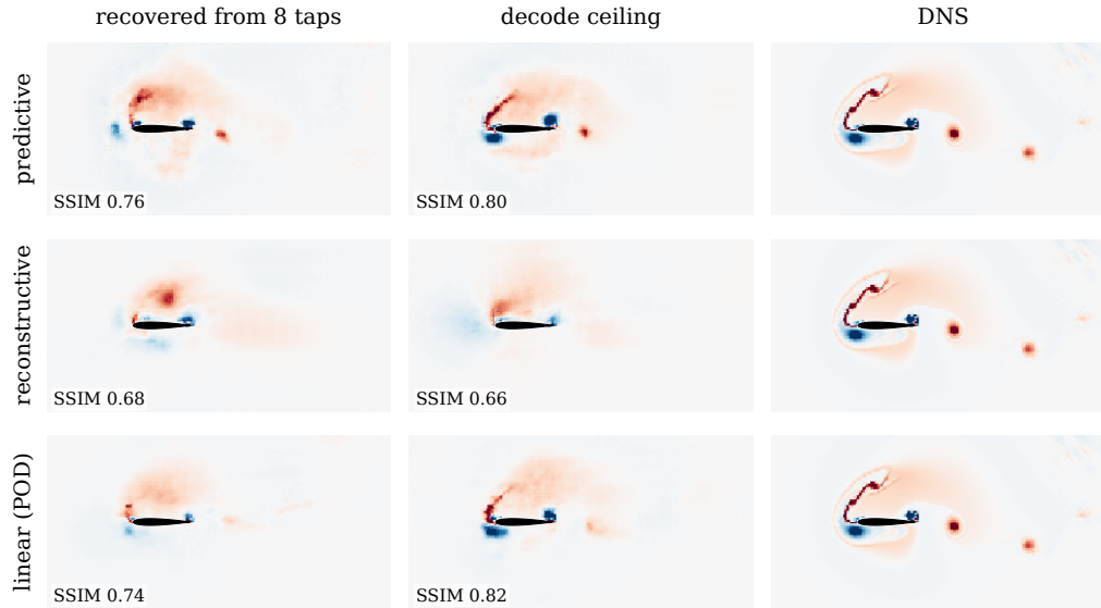
Figure 26. [APB-C1] Flow recovered from eight wall-pressure taps on the representative held-out encounter of figure 11, at the impact-side frame, one row per family. Columns: the field decoded from the pressure-recovered coefficient state, the decode ceiling (the same decoder applied to the encoded state, no pressure step), and the simulation; per-panel structural similarity annotated. The comparison is within each row, since the decoders' ceilings differ (§5.3); the ceiling-to-recovered gap is the cost of the pressure step.
