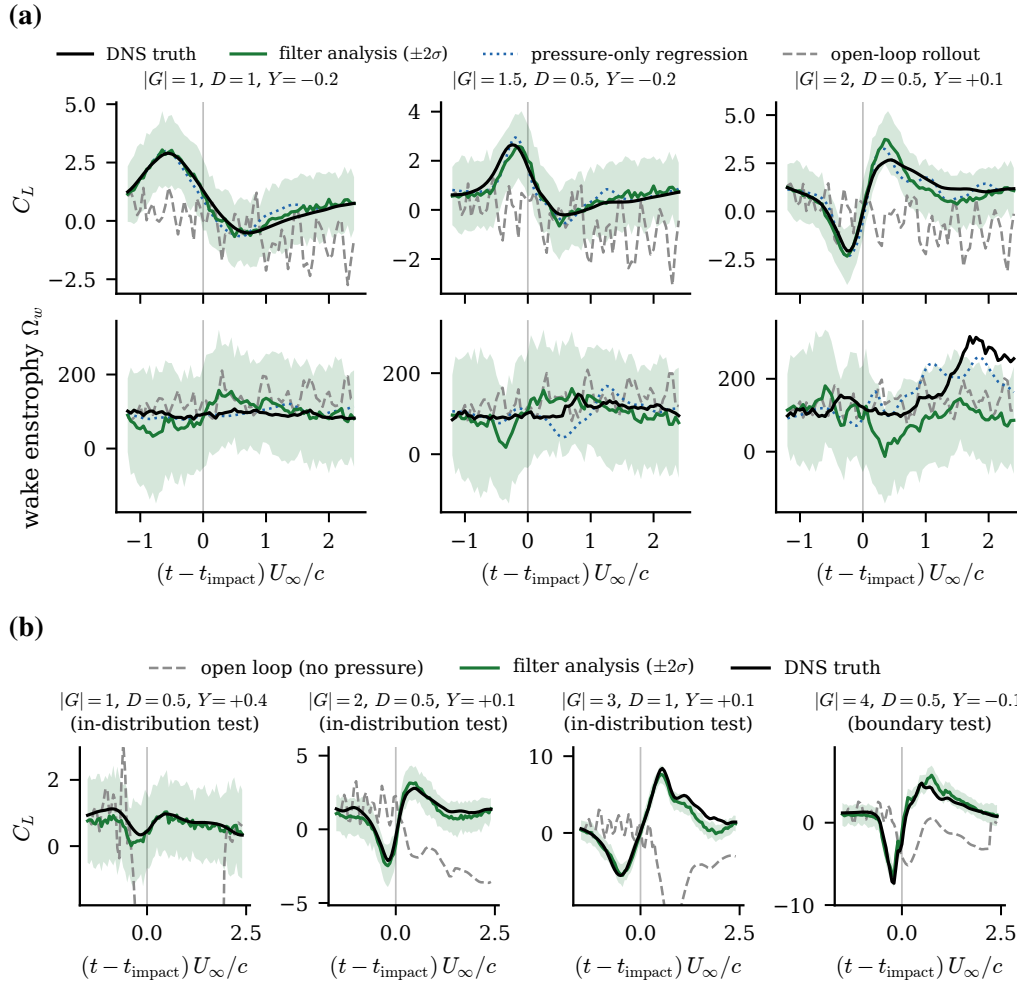
Figure 11. [S4-C4] The estimator tracks the encounter from wall pressure alone. (a) Representative held-out encounters at |G| = 1, 1.5 and 2 (columns), lift coefficient and wake enstrophy (rows); each panel shows the DNS truth, the filter analysis with its \pm 2\sigma ensemble band, the pressure-only regression, and the open-loop rollout, the vertical line marking impact. The filter follows the load through impact and relaxation where the open-loop forecast loses it and the pressure-only regression goes stale. (b) C_L estimation across the gust-intensity envelope on the wake-supervised predictive state ( d = 32 ) under the two-stage filter of §3.3.3 (one representative encounter per |G| stratum, in-distribution test set for |G| \leq 3 and boundary test set at |G| = 4 , where this filter posts no large-error encounter); inside the impact window the members are advanced by the direct multi-horizon forecaster’s median with its quantile band as state-dependent process noise (production scale c = 1.77 , validation-calibrated) and corrected by the encoded pressure observation, outside it by the matched transformer with the tap-space update. Eight wall-pressure taps, N = 64 members; the lift probe producing the read-out never enters the innovation; grey is the same forecast run open loop.
