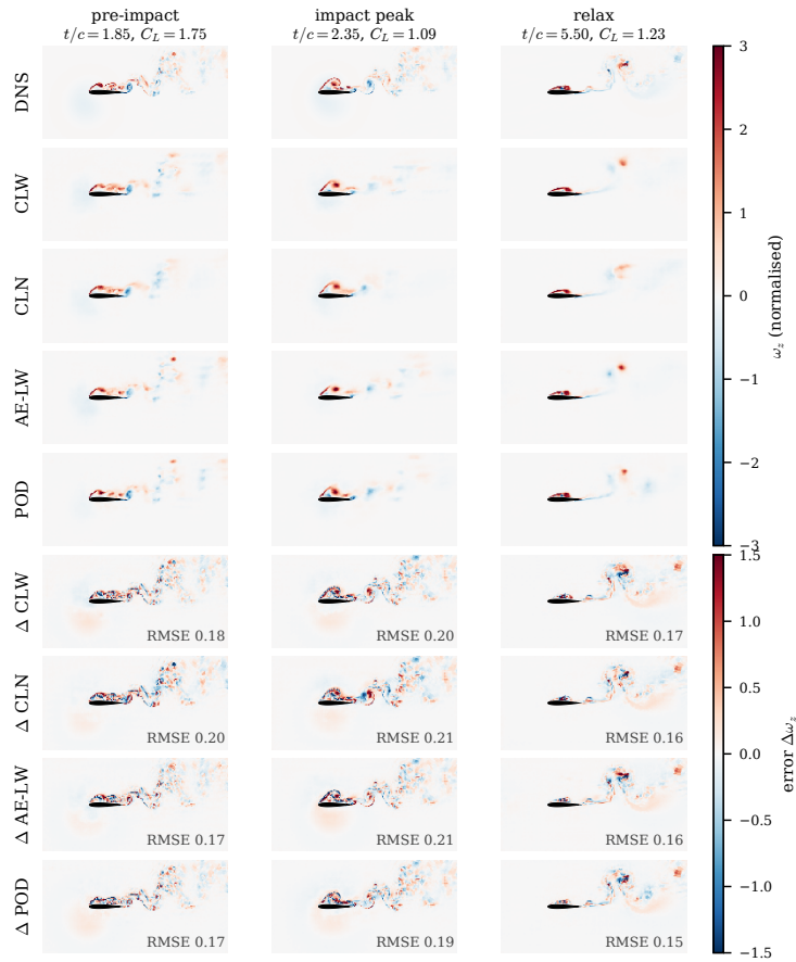
Figure 23. [APA-C11] Decode floor on a representative held-out in-distribution test encounter (one decoder seed per model): DNS, the wake-supervised predictive state, the lift-focused predictive state, the wake autoencoder and the linear basis, and the error rows at three phases. Identical-capacity frozen decoders; normalised vorticity at the fixed \pm 3 range. All four states render the field faithfully, including the linear basis: field decode is not where the states separate.
