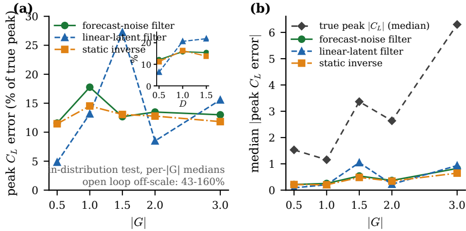
Figure 28. [APB-C3] Relative peak error across the gust envelope (in-distribution test set, medians per |G| ): the forecast-derived filter stays near 12 to 14 per cent at all but the |G| = 1 stratum while the linear filter is non-uniform; the absolute peak error (right) grows with the peak itself.
