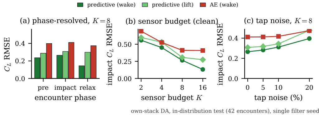
Figure 29. [APB-C4] Per-family end-to-end comparison (in-distribution test set, 42 encounters, single filter seed): (a) phase-resolved lift error per family; (b) sensor-budget sweep on each family's own nested placement; (c) tap-noise sweep at K = 8 .
