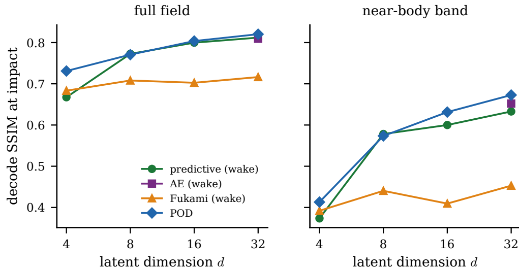
Figure 24. [APA-C12] Decode SSIM at the impact instant against latent dimension d (full field and near-body band, in-distribution test set, decode floor). The compact nonlinear states and the linear basis improve with d and saturate together; only the published-recipe lineage plateaus lower. Field decode is not the discriminator at any dimension. Single encoder/decoder seed.
