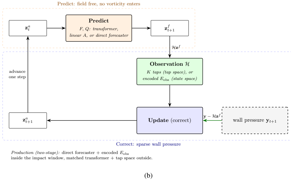
Figure 4. [S3-C1] The framework, from representation to deployment. Each module in (a) carries the stages in which it is active: the encoder is used in training and in the analyses that read \mathbf{z}_t , the three supervision heads are dropped once training ends, the predictor is the only trained module that also runs at deployment, and the visualisation decoder is trained on the frozen encoder and serves analysis alone. (a) The encoder maps the mid-plane vorticity field \omega_z \in \mathbb{R}^{192 \times 96} to a latent \mathbf{z}_t through a CNN stem, a six-layer ViT and a BatchNorm projection, and the predictor advances the latent from its own history in either of its two variants: the six-layer autoregressive transformer with rotary temporal positions of table 11, or the direct multi-horizon forecaster of §3.2.1. No gust parameters enter either network; both are unconditional. The heads read \mathbf{z}_t during training under a smooth- L_1 loss at unit weight, mapping it to the scalar lift C_L(t) ( L ), an 80-dimensional wake observable ( W ) and an 80-dimensional Chang lift-element observable ( N ); none is part of the latent-prediction loss. The decoder D_\psi pairs LapFiLM with a spectral loss. (b) At deployment the pressure-only predict-correct estimator advances an ensemble of 64 members field free through the matched prediction model, then corrects them from 8 span-averaged wall-pressure taps held out from training and placed by the per-model sensor selection. The innovation is the measured minus the predicted observation, in tap space for the base filter of §3.3.1 and in encoded latent space for the filters of §3.3.2 and §3.3.3, and the update is a stochastic ensemble Kalman step at inflation \rho = 1 with calibrated \mathbf{Q} and \mathbf{R} . No vorticity field enters the loop, the state is the same 32-vector at every step, and the lift and wake probes never enter the innovation. The evaluation protocol applied identically to every encoder is figure 21 (appendix A).
