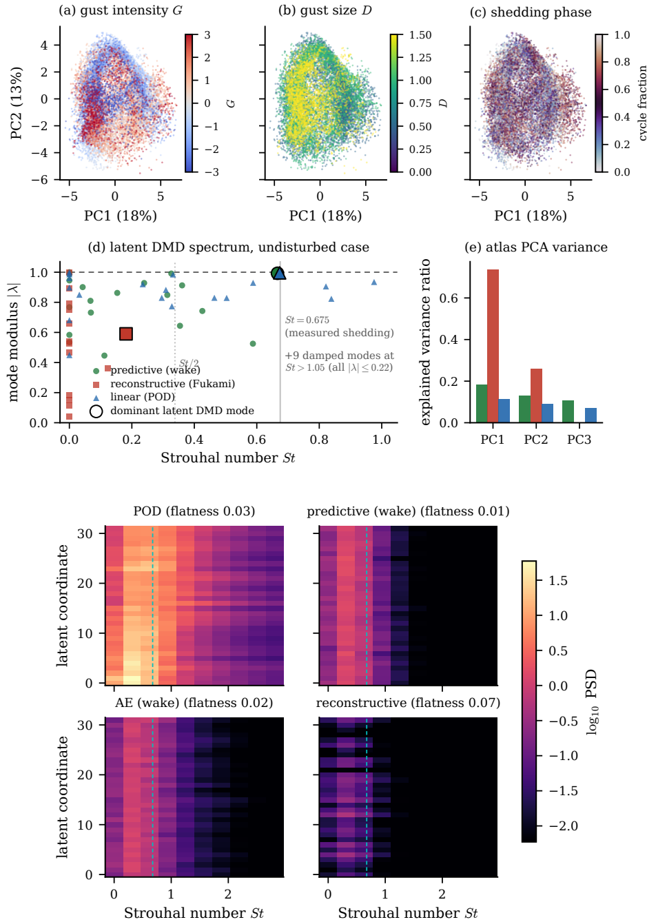
Figure 7. [S4-C1] The physics the latent state holds. (a-e) Two-dimensional projections of the predictive coefficient latent coloured by gust strength, core diameter and shedding phase, showing a parametric manifold that coheres with the release parameters, with the latent dynamic-mode-decomposition spectrum (modulus against Strouhal number, by family; the predictive and linear latents place a marginally stable mode at the measured shedding frequency while the Fukami-lineage reconstruction is damped and off-frequency), and the explained-variance ratio of the leading atlas principal components per family (e; colours as in d). (f) Per-coordinate latent spectra by family (training encounters, d = 32 ; mean Welch power spectral density against Strouhal number, coordinates ordered by peak frequency, dashed line the shedding Strouhal): the predictive coordinates concentrate at the shedding line while the published-recipe reconstruction spreads energy across frequency and the matched-supervision autoencoder does not.
