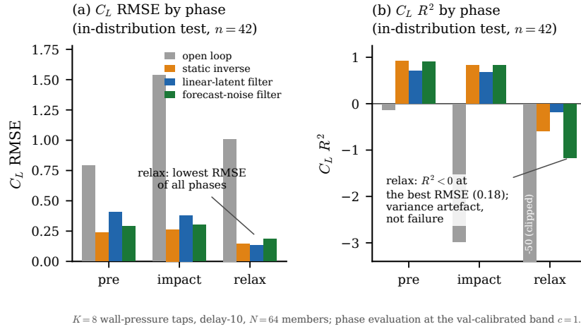
Figure 13. [S4D-C1] Phase-resolved lift tracking with the forecast-noise filter at the production coverage band on the in-distribution test set ( n = 42 encounters, K = 8 taps, delay 10, N = 64 members, every-frame pressure). Lift error per phase in physical units (a) and in R^2 (b) at the val-calibrated band: the relaxation R^2 collapse is a variance artefact, the physical error the honest phase metric. The estimator ladder, its noise calibration and the fixed-lag smoother are in appendix C (figure 30).
