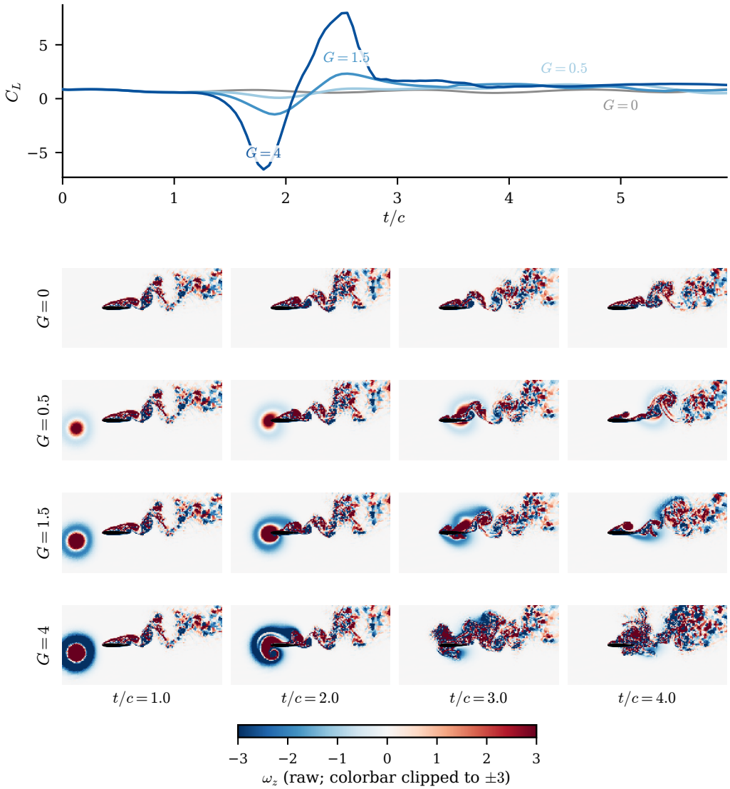
Figure 1. The vortex gust as a wake-reorganisation event, shown as a gust-strength sweep at fixed core diameter D = 0.5 and wall-normal offset Y = -0.1 (the first encounter of each case). (a) The lift coefficient C_L against convective time t/c for the four cases, with t/c = 0 the gust-release instant and impact near t/c = 2 ; the undisturbed baseline ( G = 0 ) is grey, and the load excursion deepens and widens monotonically with the gust strength G . (b) The mid-plane spanwise vorticity \omega_z for each case (rows, G = 0, 0.5, 1.5, 4 ) at four convective times (columns, t/c = 1, 2, 3, 4 ), in raw physical units with the colorbar clipped at \pm 3 (the intense cores saturate; the wake structure away from them lies within the range), and the airfoil drawn as a filled polygon. The strong gust injects a vortex that reorganises the wake through impact, while the weak cases perturb the baseline shedding only slightly; G = 4 is the |G| = 4 extrapolation case, shown here only as a physical illustration. The load spike and the wake reorganisation are the surface and field signatures of the same event, and the release parameters alone do not fix where the wake sits afterwards, which is why the wake, not only C_L , is the endpoint a reduced state must carry.
