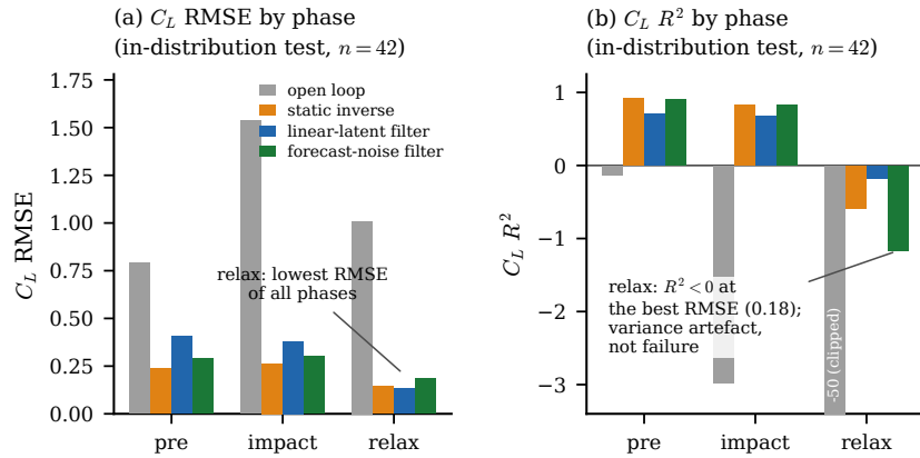
Figure 13. [S4D-C1] Phase-resolved lift tracking with the forecast-noise filter at the production coverage band on the in-distribution test set ( n = 42 encounters, K = 8 taps, delay 10, N = 64 members, every-frame pressure). Lift error per phase in physical units (a) and in R^2 (b) at the val-calibrated band: the relaxation R^2 collapse is a variance artefact, the physical error the honest phase metric. The estimator ladder, its noise calibration and the fixed-lag smoother are in appendix C (figure 30).
