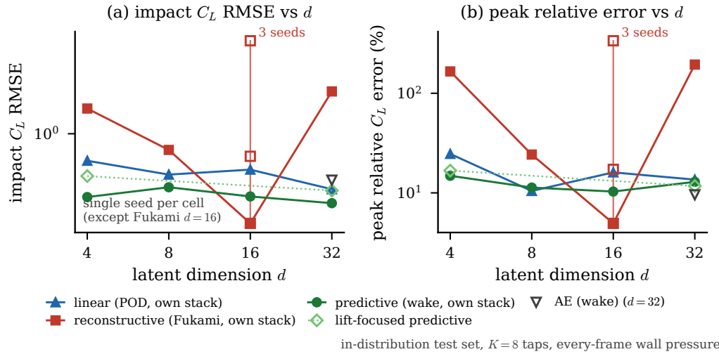
Figure 14. [S4D-C2] The assimilation-versus-dimension grid (in-distribution test set, per-family end-to-end stacks, K=8 , every-frame pressure; single seed per cell except the reconstructive d=16 cell, which carries three): impact error and relative peak error against dimension for the three families. The predictive family is uniform, the linear basis stable, the reconstructive baseline non-monotonic in dimension and irreproducible across seeds.
