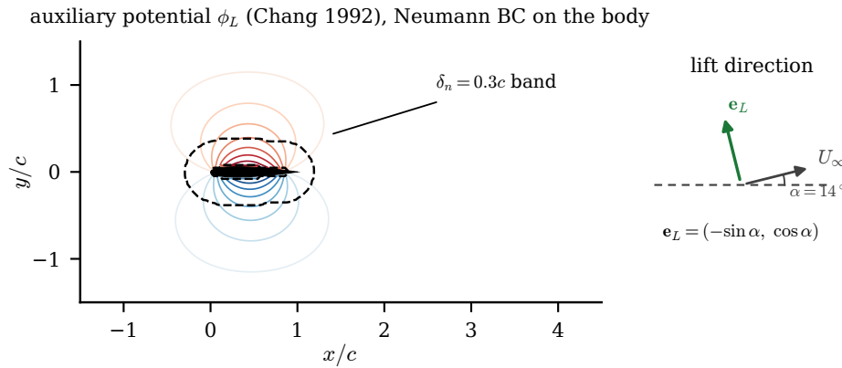
Figure 22. [APA-C10] The Chang auxiliary potential \phi_L of equation (3.2) on the cache grid (contours), the feathered \delta_n = 0.3c supervision band (dashed) and the airfoil footprint; the inset shows the lift direction \mathbf{e}_L against the inclined freestream at \alpha = 14^\circ .
