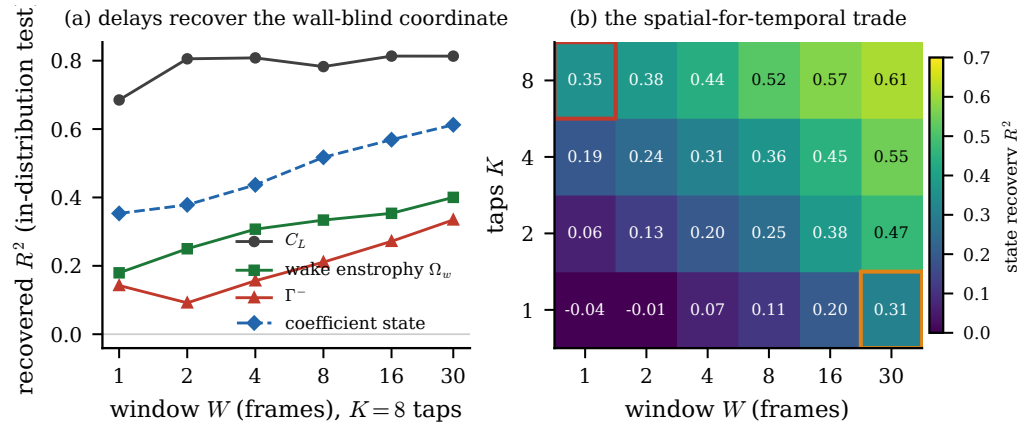
Figure 10. [S4-C3] Sensors traded for delays. (a) Recovery of each observable from eight wall-pressure taps against the length of the pressure window (in-distribution test set); the wall-blind wake circulation rises with the window while the force, visible at one instant, does not. (b) Coefficient-state recovery over the tap-count by window-length grid, with the single-tap, thirty-frame cell and the reference eight-tap, single-frame cell outlined: a long window with few taps matches a short window with many.
