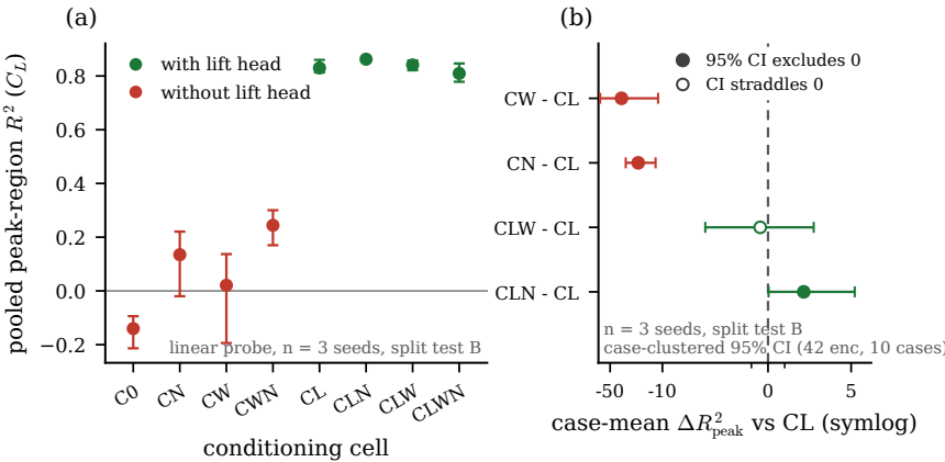
Figure 16. [APA-C4] Paired peak-region lift R^2 per conditioning-cube cell (left) and case-mean deltas against the lift-only cell CL (right, symmetric-log axis, 95 % case-clustered bootstrap intervals over the 42 in-distribution test encounters of 10 cases); filled markers mark intervals that exclude zero. The near-body lift-focused predictive state cell (CLN) is the unique positive increment; the no- L cells sit one to two orders of magnitude lower.
