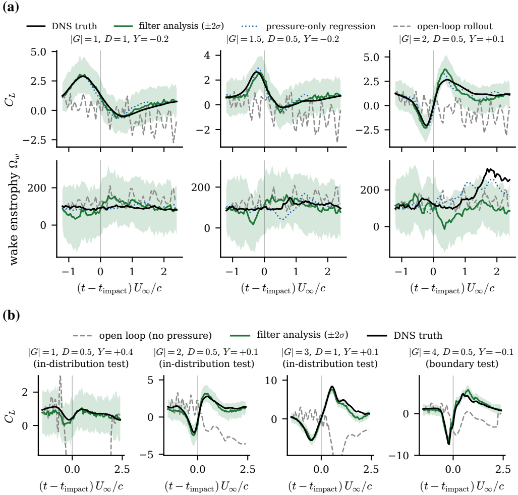
Figure 11. The estimator tracks the encounter from wall pressure alone. (a) Representative held-out encounters at |G| = 1, 1.5 and 2 (columns), lift coefficient and wake enstrophy (rows); each panel shows the DNS truth, the filter analysis with its \pm 2\sigma ensemble band, the pressure-only regression, and the open-loop rollout, the vertical line marking impact. The filter follows the load through impact and relaxation where the open-loop forecast loses it and the pressure-only regression goes stale. (b) C_L estimation across the gust-intensity envelope on the wake-supervised predictive state ( d = 32 ) under the two-stage filter of §3.3.3 (one representative encounter per |G| stratum, in-distribution test set for |G| \leq 3 and boundary test set at |G| = 4 , where this filter posts no large-error encounter); inside the impact window the members are advanced by the direct multi-horizon forecaster's median with its quantile band as state-dependent process noise (production scale c = 1.77 , validation-calibrated) and corrected by the encoded pressure observation, outside it by the matched transformer with the tap-space update. Eight wall-pressure taps, N = 64 members; the lift probe producing the read-out never enters the innovation; grey is the same forecast run open loop.
