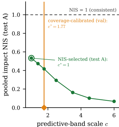
(a) latent-REX: direct multi-horizon quantile forecaster (b) two calibration criteria
