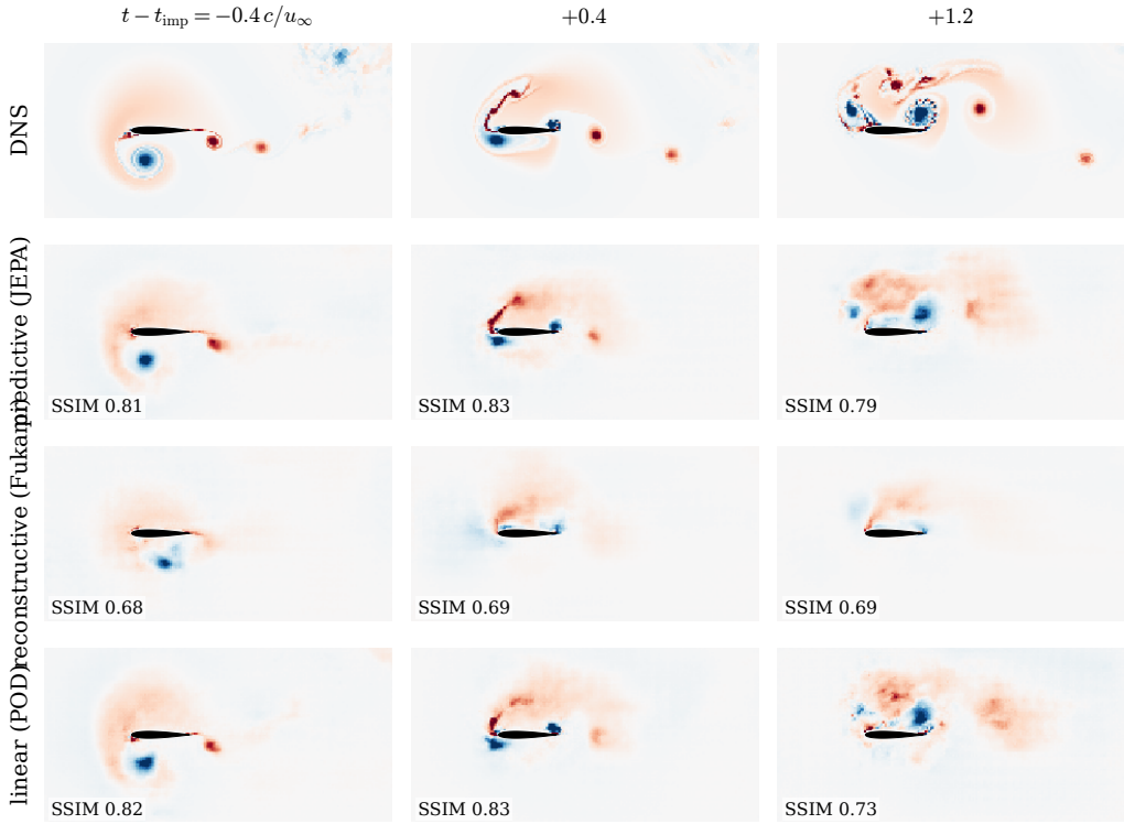
Figure 24. Decoded vorticity through the encounter on the representative held-out in-distribution test case ( |G| = 1.5 , the same encounter as figure 14). Rows: the simulation and the fields decoded from the encoded coefficient state of the predictive, reconstructive, and linear families; columns: a pre-impact, an impact, and a relaxation frame. Each decode is produced by the same diagnostic decoder that defines the decode-floor similarity of table 6, trained on the frozen encoder; the per-panel structural similarity is annotated. The pooled decode is soft by construction (§5.3); the comparison is between rows at matched frames, and no family's decode is part of any training loss.
