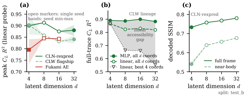
Figure 9. The dimension axis on the in-distribution test set. (a) Peak-region lift R^2 (linear probe) against latent dimension for the three lineages; shaded bands are three-seed min-max ranges, open markers single seeds. (b) The probe-dilution control: a multilayer probe is flat in d while the best-four-coordinate linear probe falls, so the d = 4 advantage is linear accessibility of a distributed code, not information. (c) Decoded SSIM (Wang convention, §3.5) of the same lineage rises with d : the wake tier is not compressible.
