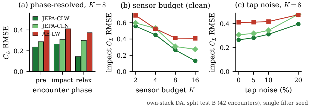
Figure 18. Own-stack family comparison (in-distribution test set, 42 encounters, single filter seed): (a) phase-resolved lift error per family; (b) sensor-budget sweep on each family's own nested placement; (c) tap-noise sweep at K = 8 .
