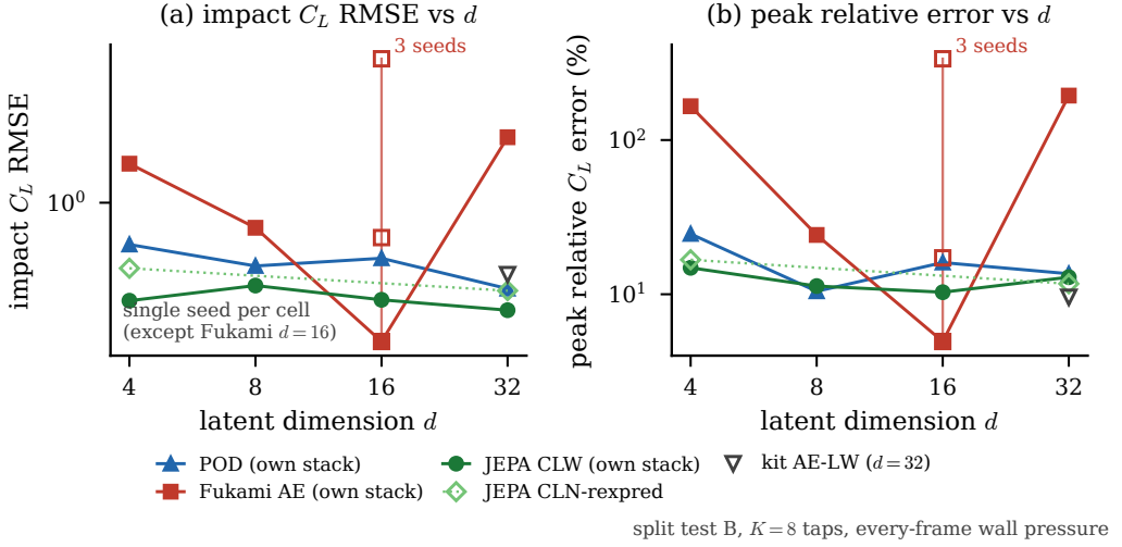
Figure 20. The assimilation-versus-dimension grid (in-distribution test set, own stacks, K=8 , every-frame pressure; single seed per cell except the reconstructive d=16 cell, which carries three): impact error and relative peak error against dimension for the three families. The predictive family is uniform, the linear basis stable, the reconstructive baseline erratic in dimension and in seed.
