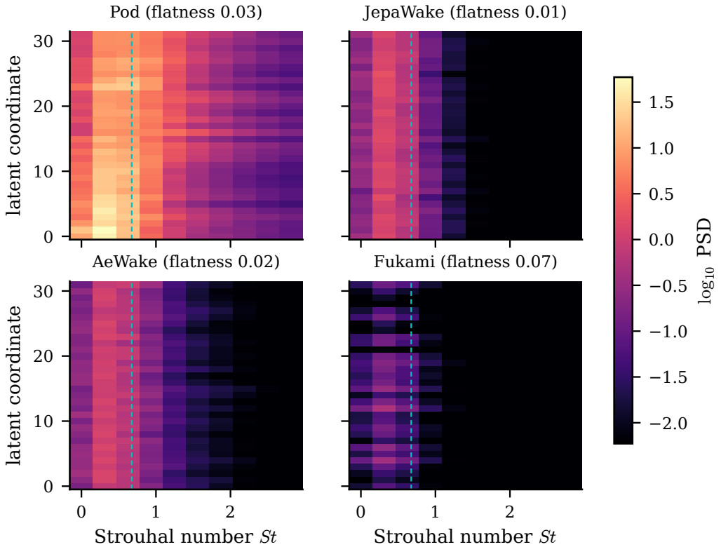
Figure 7. Per-coordinate latent spectra by family (training encounters, d = 32 ; mean Welch power spectral density against Strouhal number, coordinates ordered by peak frequency; the dashed line marks the shedding Strouhal). The predictive coordinates concentrate at the shedding line while the published-recipe reconstruction spreads energy across frequency, and the matched-supervision autoencoder does not.
