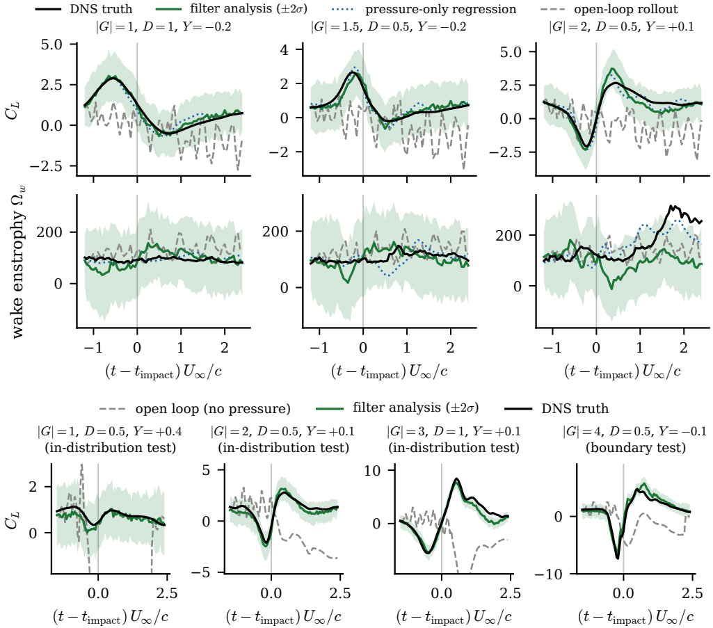
Figure 11. The estimator tracks the encounter from wall pressure alone. Top: representative held-out encounters at |G| = 1, 1.5 and 2 (columns), lift coefficient and wake enstrophy (rows); each panel shows the DNS truth, the filter analysis with its \pm 2\sigma ensemble band, the pressure-only regression, and the open-loop rollout, the vertical line marking impact. The filter follows the load through impact and relaxation where the open-loop forecast loses it and the pressure-only regression goes stale. Bottom: C_L estimation across the gust-intensity envelope on the wake-supervised predictive state ( d = 32 ) under the two-stage filter of §3.3.3 (one representative encounter per |G| stratum, in-distribution test set for |G| \leq 3 and boundary test set at |G| = 4 , where this filter posts no large-error encounter); inside the impact window the members are advanced by the direct multi-horizon forecaster’s median with its quantile band as state-dependent process noise (production scale c = 1.77 , validation-calibrated) and corrected by the encoded pressure observation, outside it by the matched transformer with the tap-space update. Eight wall-pressure taps, N = 64 members; the lift probe producing the read-out never enters the innovation; grey is the same forecast run open loop.
