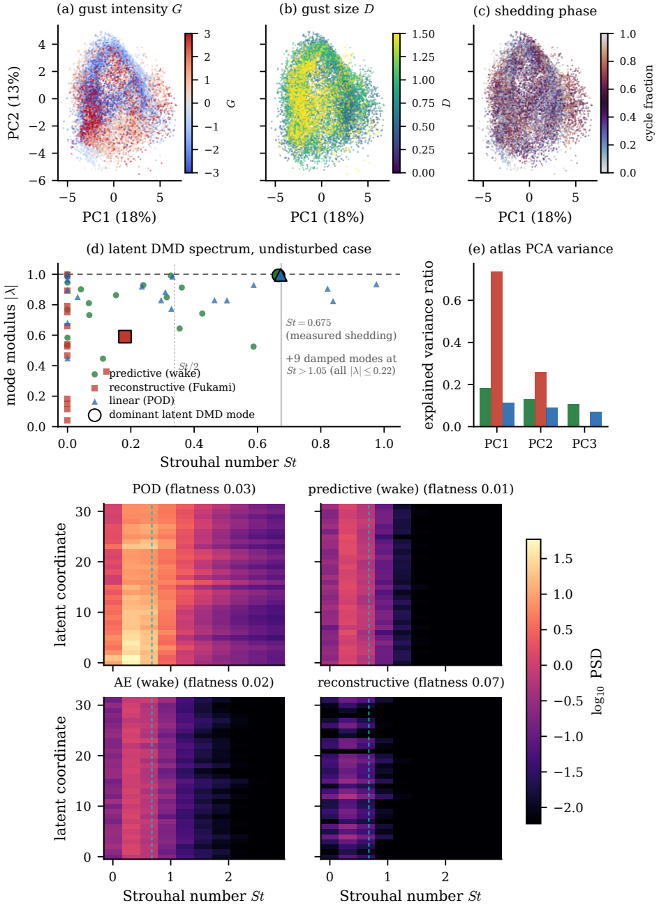
Figure 7. The physics the latent state holds. Top: two-dimensional projections of the predictive coefficient latent coloured by gust strength, core diameter and shedding phase, showing a parametric manifold that coheres with the release parameters, with the latent dynamic-mode-decomposition spectrum (modulus against Strouhal number, by family; the predictive and linear latents place a marginally stable mode at the measured shedding frequency while the Fukami-lineage reconstruction is damped and off-frequency), and the explained-variance ratio of the leading atlas principal components per family (e; colours as in d). Bottom: per-coordinate latent spectra by family (training encounters, d = 32 ; mean Welch power spectral density against Strouhal number, coordinates ordered by peak frequency, dashed line the shedding Strouhal); the predictive coordinates concentrate at the shedding line while the published-recipe reconstruction spreads energy across frequency and the matched-supervision autoencoder does not.
