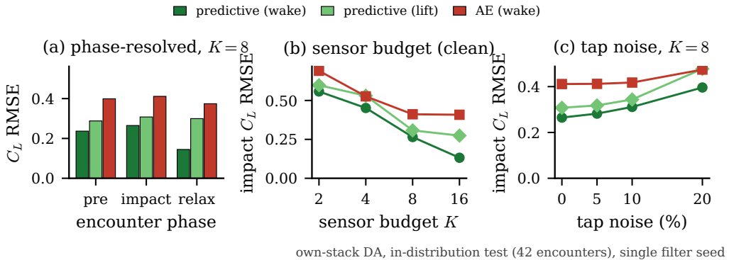
Figure 29. Per-family end-to-end comparison (in-distribution test set, 42 encounters, single filter seed): (a) phase-resolved lift error per family; (b) sensor-budget sweep on each family's own nested placement; (c) tap-noise sweep at K = 8 .
