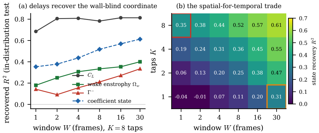
Figure 10. Sensors traded for delays. (a) Recovery of each observable from eight wall-pressure taps against the length of the pressure window (in-distribution test set); the wall-blind wake circulation rises with the window while the force, visible at one instant, does not. (b) Coefficient-state recovery over the tap-count by window-length grid, with the single-tap, thirty-frame cell and the reference eight-tap, single-frame cell outlined: a long window with few taps matches a short window with many.
