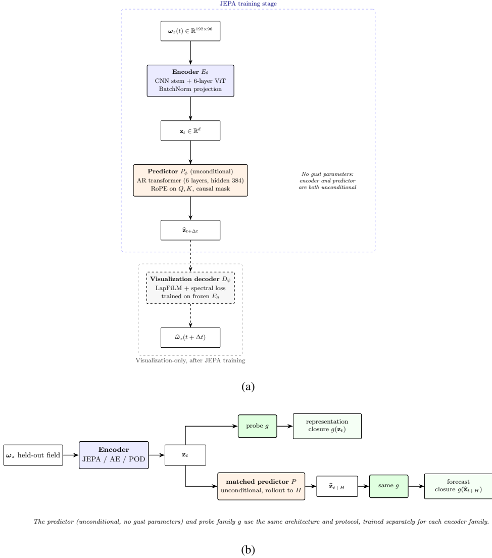
Figure 3. The predictive model and how it is evaluated. (a) The encoder maps the mid-plane vorticity field to a latent \mathbf{z}_t , and the autoregressive predictor advances the latent from its own history; no gust parameters enter the encoder or the predictor. The two auxiliary observable heads (lift and wake) read \mathbf{z}_t during JEPA training with small weights and are not part of the latent-prediction loss; they are omitted from the schematic for clarity. The visualisation decoder is trained only after the encoder is frozen and is used solely for the diagnostic decodes of §4.6, never in the predictive loss. (b) Evaluation applies the same predictor and probe family g to every encoder family: a probe on the simulation-encoded latent measures representational closure, the headline, and the same probe on the rolled-out latent \hat{\mathbf{z}}_{t+H} measures forecast closure, reported as secondary.
