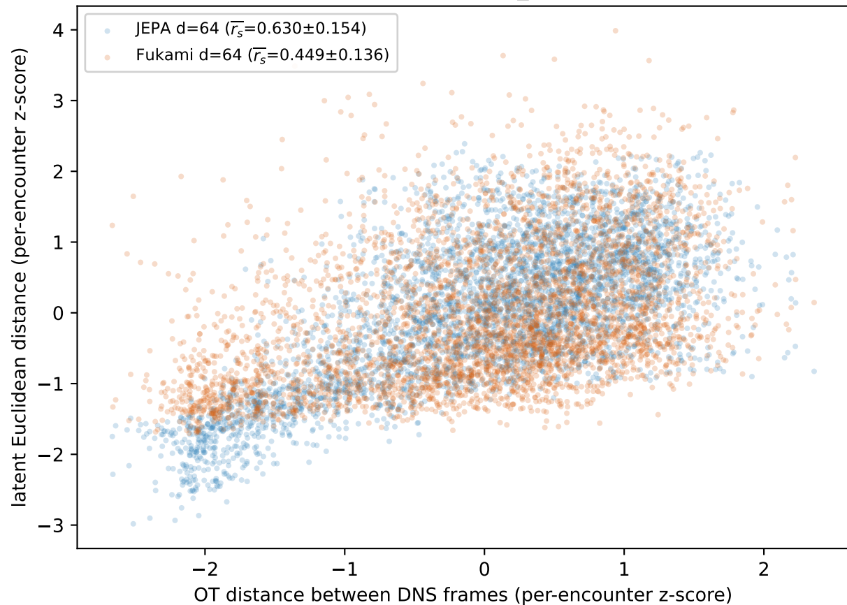
D-ii: OT-vs-latent Shepard (test_b, within-encounter)
