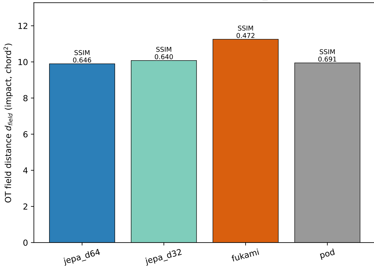
D-i: OT field distance vs SSIM (test_b, impact)
