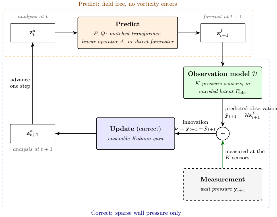
Production configuration (two-stage): direct forecaster with the encoded observation inside the impact window, matched transformer with the pressure sensors outside it.
