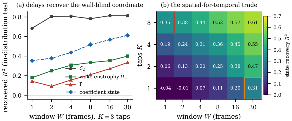
Figure 10. [S4-C3]Sensors traded for delays. (a) Recovery of each observable from eight wall-pressure taps against the length of the pressure window (in-distribution test set); the wall-blind wake circulation rises with the window while the force, visible at one instant, does not. (b) Coefficient-state recovery over the tap-count by window-length grid, with the single-tap, thirty-frame cell and the reference eight-tap, single-frame cell outlined: a long window with few taps matches a short window with many.
