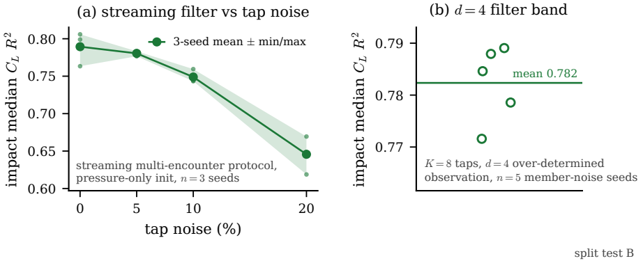
Figure 20. Deployment realism (in-distribution test set): (a) streaming multi-encounter filter against tap noise, three member-noise seeds, validation-selected band (no test-set reference); (b) the d = 4 filter band over five member-noise seeds.
