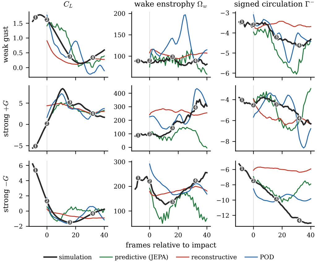
Figure 4. The unconditioned rollout tracks the encounter, shown qualitatively. Predicted observables through representative held-out encounters (rows), for the lift coefficient, the wake enstrophy, and the negative circulation (columns). The simulation is the bold reference; the rollout of the unconditioned predictor, started at the impact frame with no gust input, is the coloured line, and the dashed line is the reconstruction from the encoded latent. The rollout tracks the wake observables through the leading-edge-vortex peak and into recovery before drifting gently at long times. We report this as qualitative tracking, not as a closure R^2 . Numbered glyphs mark the four encounter stages used throughout: baseline, impact, peak load, and recovery.
