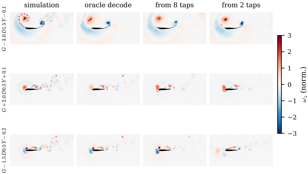
Figure 17. Flow recovered from sparse wall pressure on three held-out encounters (rows, labelled by (G, D, Y) ). Columns: the simulation, the oracle decode (the visualisation decoder applied to the simulation-encoded latent), and the decode of the latent estimated from K = 8 and K = 2 TCSI pressure taps. From eight taps the predictive latent recovers the leading-edge vortex and shear layer close to the oracle; two taps capture the gross impingement. The decoder is blurry by design (§4.4).
