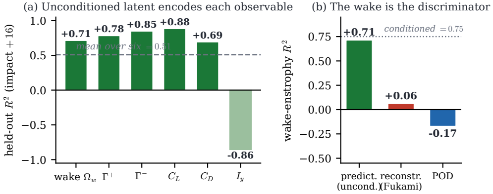
Figure 3. Representational closure of the unconditioned predictive latent at H = 16 after gust impact, the headline result. (a) Held-out R^2 of a fixed linear probe applied to the simulation-encoded latent (no rollout) for each of the six observables, on the in-distribution test set (test_b, n = 42 ); the dashed line marks the mean over the six and the one weak observable, the mid-plane impulse I_y , is shaded light. (b) The wake-entropy R^2 across families: the unconditioned predictive latent (0.71) against the reconstructive autoencoder (0.06) and the linear basis (-0.17), each baseline at its least-bad latent dimension; the dotted line marks the conditioned model's 0.75, which the unconditioned latent essentially matches. The wake is the discriminator, and the predictive latent keeps it with no privileged knowledge of the gust.
