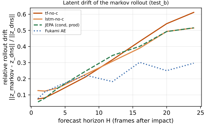
Figure 5. Relative drift of the unconditioned rollout on test_b versus forecast horizon H , measured as the deviation of the rolled latent from the simulation-encoded latent normalised by the encoded-latent scale, \|\hat{\mathbf{z}}_{\text{rollout}} - \mathbf{z}_{\text{DNS}}\| / \|\mathbf{z}_{\text{DNS}}\| . The unconditioned transformer predictor (tf-no-c) and a recurrent unconditioned variant (lstm-no-c) drift gradually and track the conditioned production model closely, so dropping the gust parameters does not destabilise the rollout. This is a deviation diagnostic of the unconditioned model, not a forecast- R^2 headline; the family-separating drift is the Mahalanobis manifold-departure of table 8.
