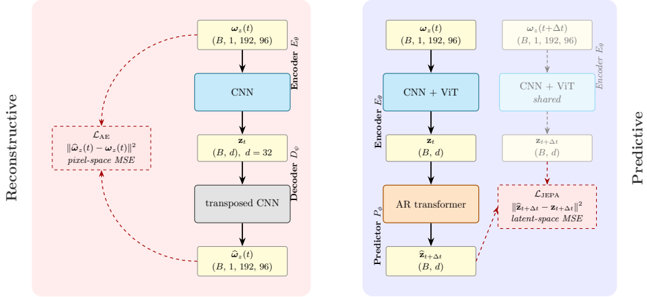
Figure 22. Predictive versus reconstructive training. Left: the reconstructive autoencoder encodes the field at t , decodes it, and incurs a field-space error. Right: the predictive model encodes the fields at t and t + \Delta t with shared weights and incurs a latent-space error between the predicted and observed target embeddings, with no field-space loss and no decoder during training. This is the contrast the matched-predictor protocol of §3.2 evaluates; the visualisation decoder is trained only afterwards, on the frozen encoder.
