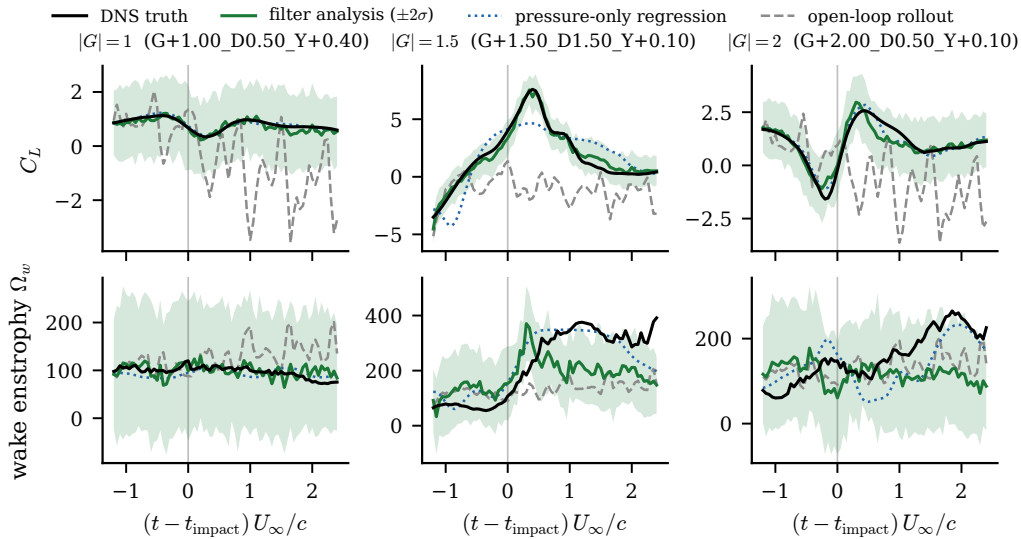
Figure 15. The estimator tracks the encounter from wall pressure alone. Columns are representative held-out encounters at |G| = 1, 1.5 and 2 ; rows are the lift coefficient and the wake enstrophy. Each panel shows the DNS truth, the filter analysis with its \pm 2\sigma ensemble band, the pressure-only regression, and the open-loop rollout; the vertical line marks impact. The filter follows the load through impact and relaxation where the open-loop forecast loses it and the pressure-only regression goes stale.
