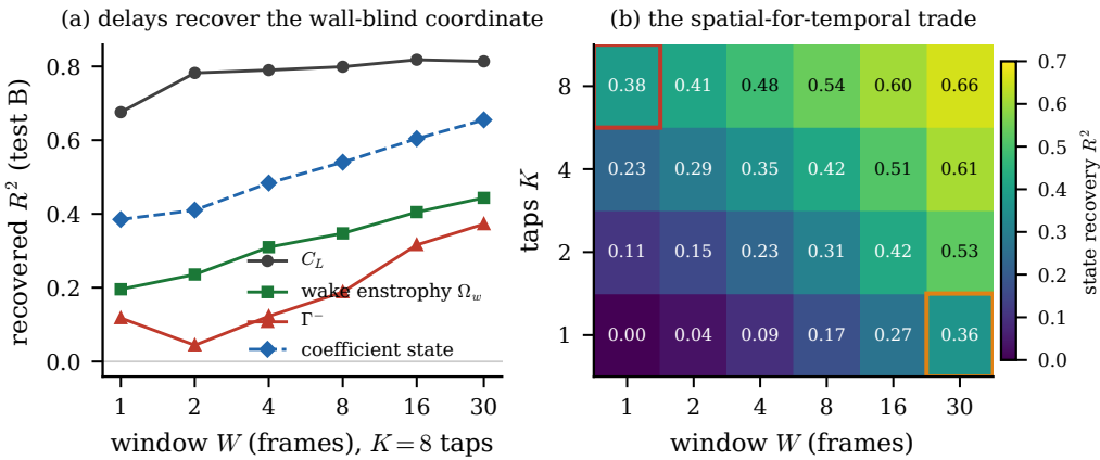
Figure 14. Sensors traded for delays. (a) Recovery of each observable from eight wall-pressure taps against the length of the pressure window (in-distribution test set); the wall-blind wake circulation rises with the window while the force, visible at one instant, does not. (b) Coefficient-state recovery over the tap-count by window-length grid, with the single-tap, thirty-frame cell and the reference eight-tap, single-frame cell outlined: a long window with few taps matches a short window with many.
