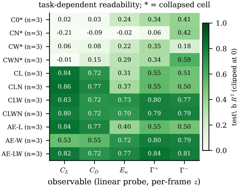
Figure 7. Task-dependent readability (in-distribution test set, linear probes on the per-frame state, seed mean over three encoder seeds per cell): lift and drag follow the L head, the wake block ( E_w , \Gamma^\pm ) follows the W head or the reconstruction objective, and collapsed cells (asterisks) read nothing linearly.
