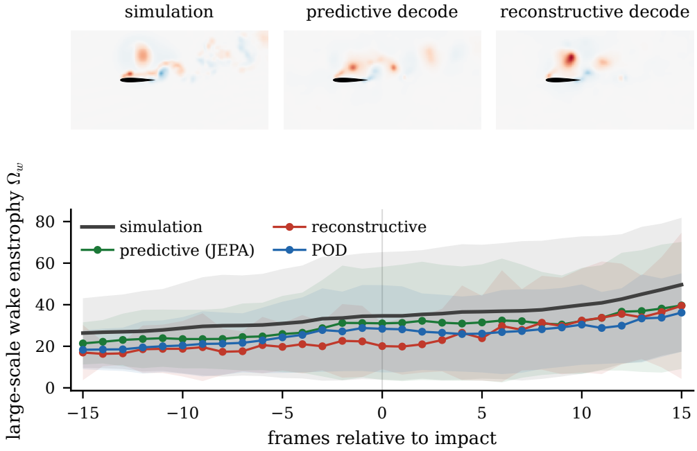
Figure 12. Gaussian scale decomposition ( \sigma/c = 0.05 ) of the held-out reconstructions. Top: large-scale vorticity for the simulation, the predictive decode, and the reconstructive autoencoder at H = 16 ; the predictive latent retains the leading-edge vortex and shear layer the reconstructive one smooths away. Bottom: large-scale wake enstrophy through the staged encounter for the simulation, predictive, and reconstructive fields, on each split.
