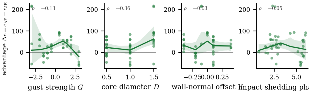
Figure 10. Per-encounter paired improvement \Delta e = e_{\text{AE}} - e_{\text{JEPA}} in held-out wake-entropy error against the gust strength G , core diameter D , wall-normal offset Y , and the baseline shedding phase at impact \phi (test_b, n = 42 ); positive \Delta e means the predictive latent carries the smaller error. Each panel shows the per-encounter values, a locally weighted (LOWESS) trend, and a bootstrap band over encounters. The predictive advantage grows with D (significant) but shows no significant G or Y trend; the shedding-phase axis falls into two clusters because impact is fixed near a single convective instant.
