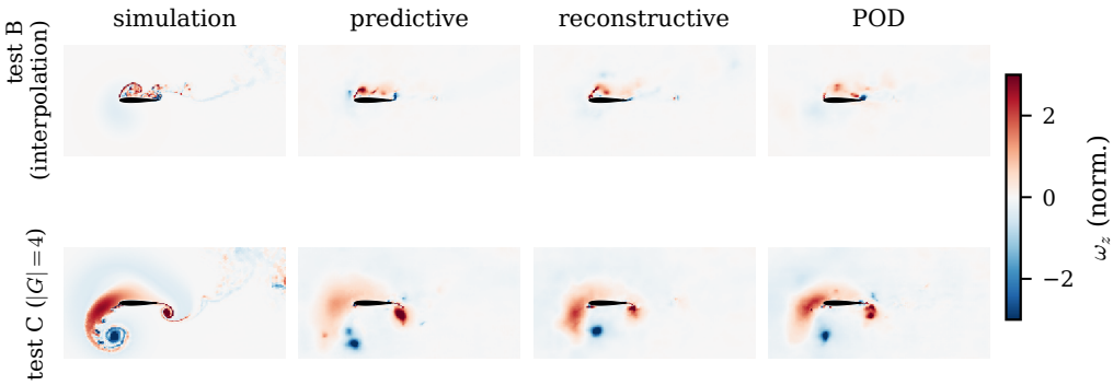
Figure 11. Decoded vorticity at the impact frame on held-out encounters (rows: an interpolation test_b encounter and a |G| = 4 test_c encounter) for the simulation and the predictive, reconstructive, and POD decodes (columns). The predictive decoder is blurry by design but localises the impingement; the reconstructive autoencoder collapses toward a near-uniform field on the held-out interpolation condition, while the linear basis is amplitude-accurate. All families degrade in the |G| = 4 regime, reported as the observability boundary of §2.1 rather than as a generalisation claim. Field-space similarity is read only as a labelled decode ceiling (§4.6).
