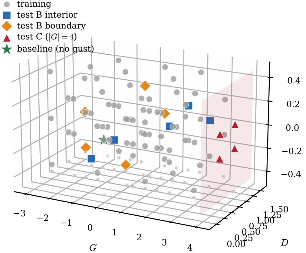
Figure 1. Parameter-space sampling of the 85 cases in the (G, D, Y) gust envelope, shown as one isometric view and coloured by split: training (229 encounters), the stratified in-distribution test set (test_b, 42 encounters, split into interior and boundary tiers), and the out-of-distribution extrapolation set (test_c, 24 encounters). The translucent plane marks the |G| = 4 extrapolation boundary and the grey points on the floor are the projection of every case, which shows that training mass concentrates near Y/c = 0 , the reason the wall-normal offset is the least well resolved parameter (§4.6).
