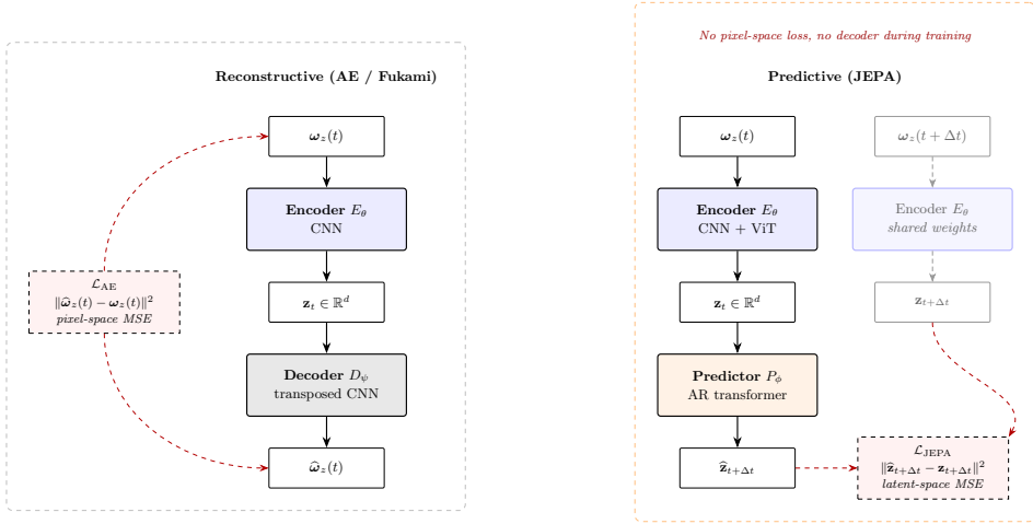
Figure 15. Predictive versus reconstructive training. Left: the reconstructive autoencoder encodes the field at t , decodes it, and incurs a field-space error. Right: the predictive model encodes the fields at t and t + \Delta t with shared weights and incurs a latent-space error between the predicted and observed target embeddings, with no field-space loss and no decoder during training. This is the contrast the matched-predictor protocol of §3.2 evaluates; the visualisation decoder is trained only afterwards, on the frozen encoder.
