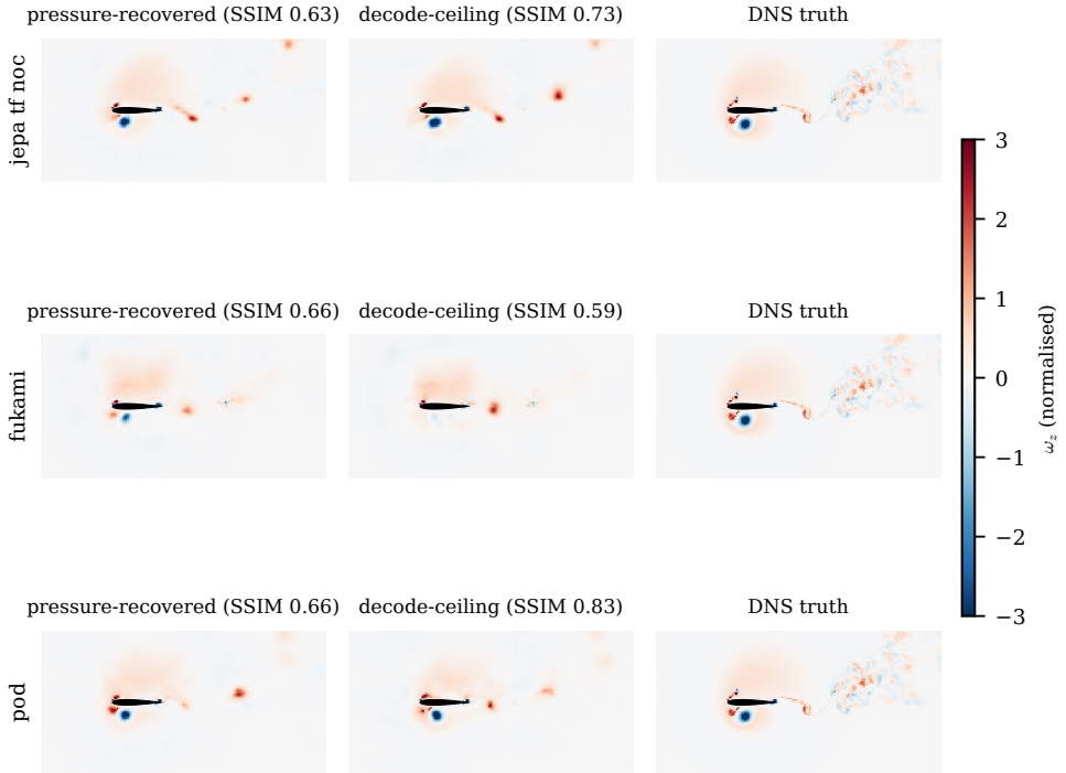
Figure 17. Flow recovered from K = 8 target-blind (qDEIM) wall-pressure taps on a representative held-out encounter (the typical-difficulty case G = +1.50 , D = 1.50 , Y = +0.10 ), one row per family. Columns: the field decoded from the pressure-estimated latent, the decode ceiling (the same decoder applied to the true encoded latent, with no pressure step), and the simulation. The per-panel similarity makes the appendix point visible: the linear basis reaches field parity through the highest decode ceiling, not through better pressure-to-state recovery, where the predictive latent has the smallest ceiling gap. The decoder is blurry by design (§4.6); the comparison is between the columns of the same row.
