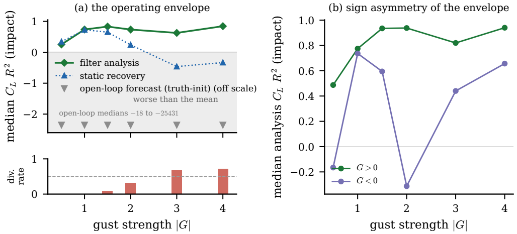
Figure 11. The gust-intensity operating envelope, diagnosed with the base frozen filter (the production estimator remains the two-stage filter of §4.6.3; figure 12 carries the forecast-noise filter’s phase-resolved errors). (a) Median analysis lift closure ( R^2 , impact window) against gust strength for the base filter, the static single-frame recovery, and the truth-initialised open-loop forecast, with the filter consistency-failure rate as the strip beneath; the shaded band marks closure worse than predicting the encounter mean, and the open-loop forecast lies off the scale below it. The base filter tracks the median throughout but becomes under-dispersed from a gust ratio of about three, where the consistency-failure rate climbs. (b) The same base-filter closure resolved by the physical sign of the gust, showing the wider usable envelope of the positive gusts.
