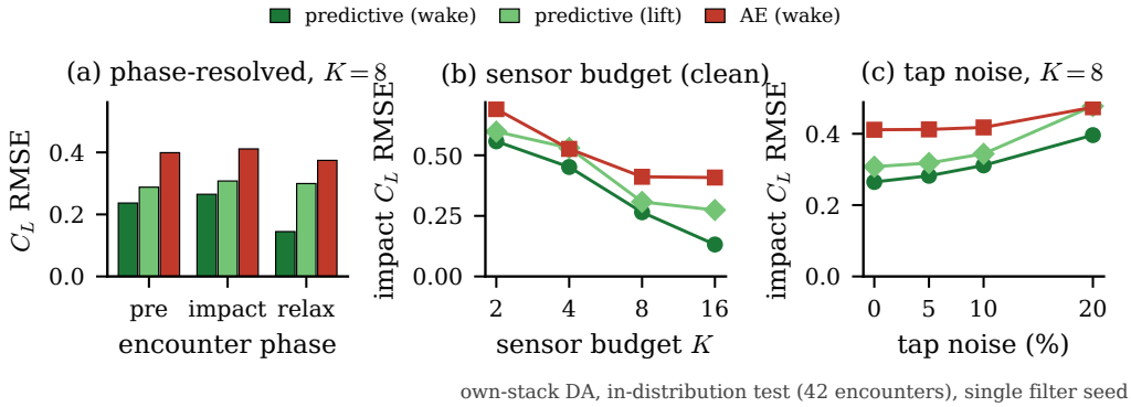
Figure 28. Per-family end-to-end comparison (in-distribution test set, 42 encounters, single filter seed): (a) phase-resolved lift error per family; (b) sensor-budget sweep on each family’s own nested placement; (c) tap-noise sweep at K = 8 .
