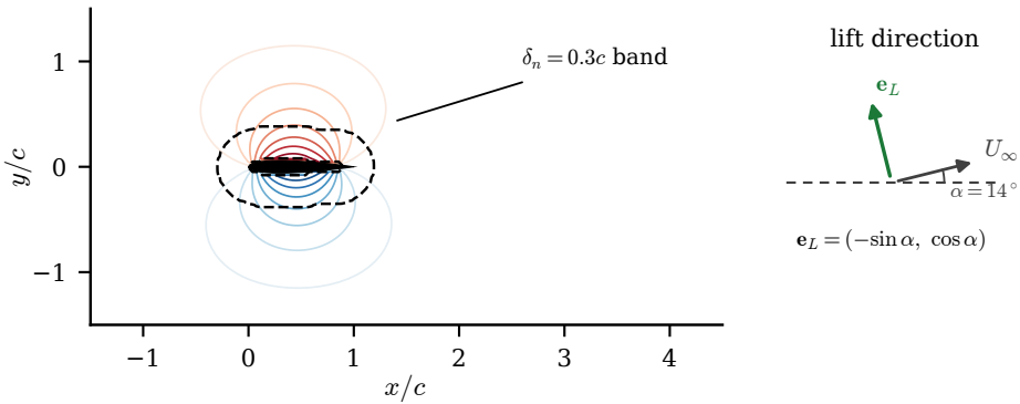
Figure 21. The Chang auxiliary potential \phi_L of equation (3.1) on the cache grid (contours), the feathered \delta_n = 0.3c supervision band (dashed) and the airfoil footprint; the inset shows the lift direction \mathbf{e}_L against the inclined freestream at \alpha = 14^\circ .
