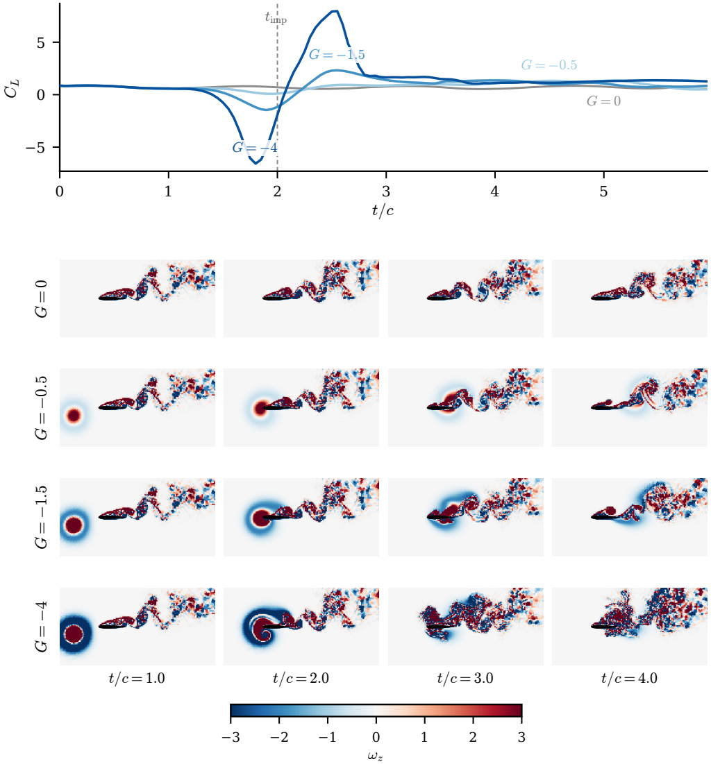
Figure 1. The vortex gust as a wake-reorganisation event: a gust-strength sweep at fixed core diameter D = 0.5 and offset Y = -0.1 (first encounter of each case). Top: lift coefficient C_L against convective time, with t/c = 0 the release and t_{\text{imp}} (dashed) the leading-edge crossing near t/c = 2 ; the load excursion deepens and widens with |G| , the baseline ( G = 0 ) in grey. Bottom: mid-plane spanwise vorticity \omega_z per case (rows G = 0, -0.5, -1.5, -4 ) at four times (columns t/c = 1, 2, 3, 4 ), raw units, colourbar clipped at \pm 3 (intense cores saturate), airfoil filled. The strong gust reorganises the wake through impact while the weak cases barely perturb the shedding; G = -4 is the |G| = 4 extrapolation case, shown only for illustration. The release parameters alone do not fix where the wake sits afterwards, which is why the wake, not only C_L , is the endpoint a reduced state must carry.
