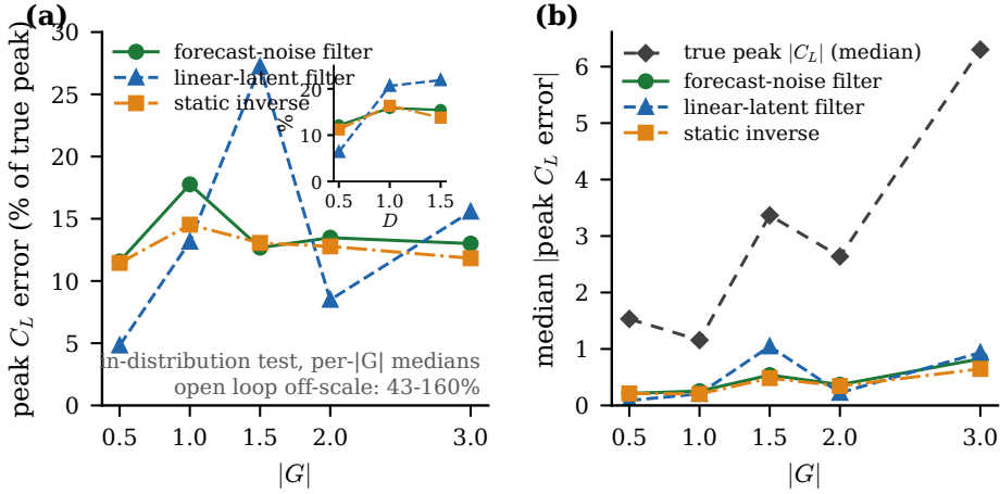
Figure 27. Relative peak error across the gust envelope (in-distribution test set, medians per |G| ): the forecast-derived filter stays near 12 to 14 per cent at all but the |G| = 1 stratum while the linear filter is non-uniform; the absolute peak error (right) grows with the peak itself.
