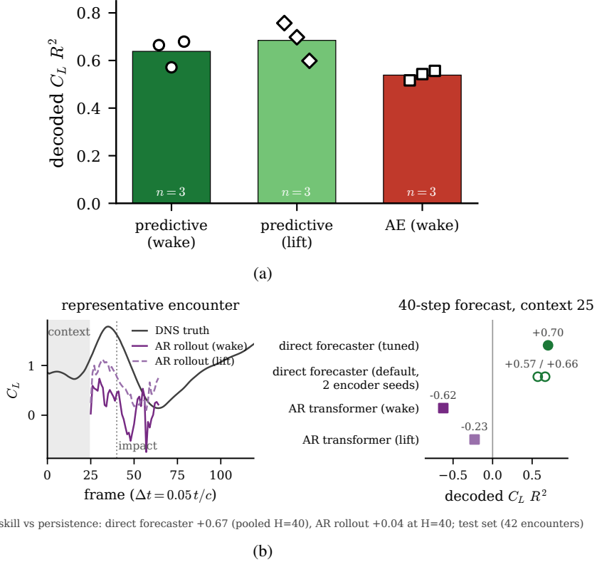
Figure 7. Forecasting the state on the in-distribution test set. (a) Decoded lift R^2 of the shared direct multi-horizon forecaster per family (three operator seeds each, bars at the seed mean): the predictive states forecast the lift best. (b) Direct versus autoregressive over forty steps through the impact from a 25-frame context: the one-shot forecast stays usable where the rollout compounds. The conditioning null, where the (G, D, Y) oracle degrades the forecast and the phase covariate is a wash, is figure 18 in appendix A.
