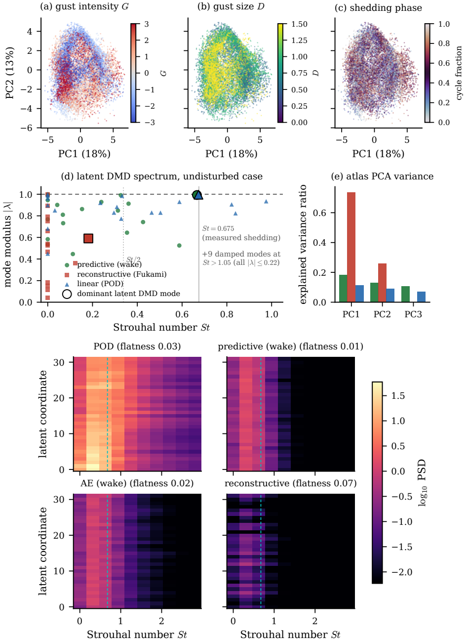
Figure 6. The physics the latent state holds. Top: two-dimensional projections of the predictive coefficient latent coloured by gust strength, core diameter and shedding phase, showing a parametric manifold that coheres with the release parameters, with the latent dynamic-mode-decomposition spectrum (modulus against Strouhal number, by family; the predictive and linear latents place a marginally stable mode at the measured shedding frequency while the Fukami-lineage reconstruction is damped and off-frequency), and the explained-variance ratio of the leading atlas principal components per family (e; colours as in d). Bottom: per-coordinate latent spectra by family (training encounters, d = 32 ; mean Welch power spectral density against Strouhal number, coordinates ordered by peak frequency, dashed line the shedding Strouhal); the predictive coordinates concentrate at the shedding line while the published-recipe reconstruction spreads energy across frequency and the matched-supervision autoencoder does not.
