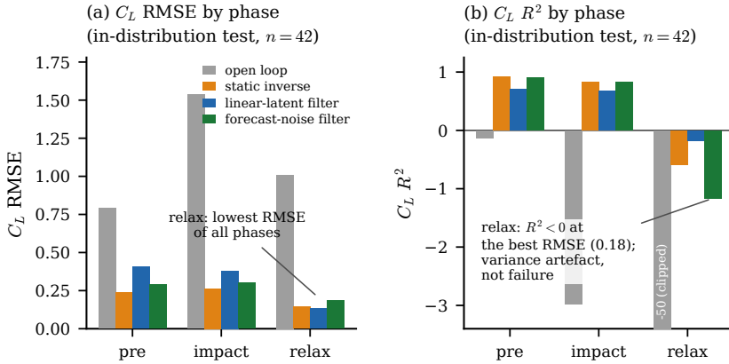
Figure 12. Phase-resolved lift tracking with the forecast-noise filter at the production coverage band on the in-distribution test set ( n = 42 encounters, K = 8 taps, delay 10, N = 64 members, every-frame pressure). Lift error per phase in physical units (a) and in R^2 (b) at the val-calibrated band: the relaxation R^2 collapse is a variance artefact, the physical error the honest phase metric. The estimator ladder, its noise calibration and the fixed-lag smoother are in appendix C (figure 29).
