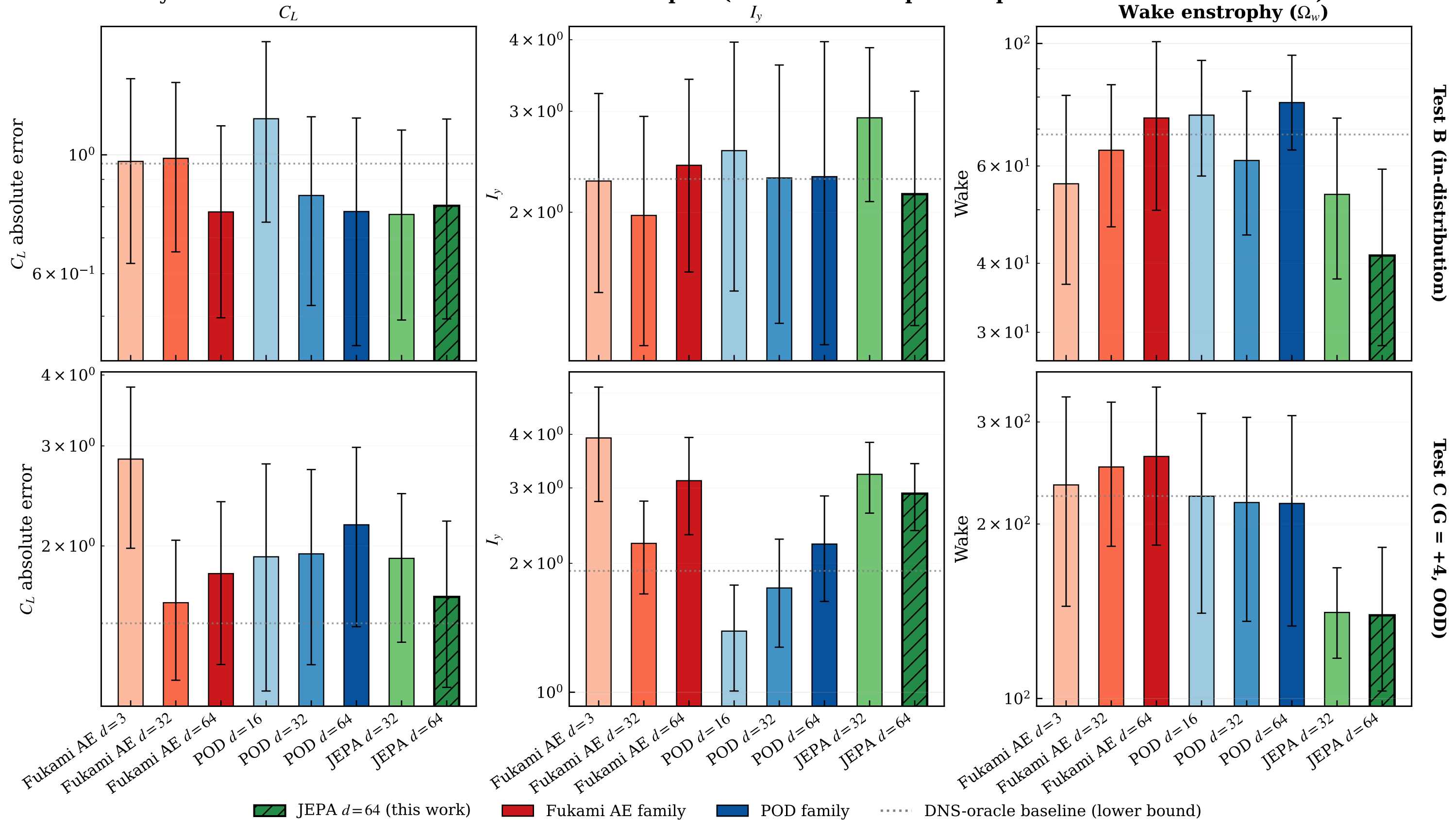
Physical Markov closure at H=16 frames after impact (unified –no–output–BN predictor across all baselines)
