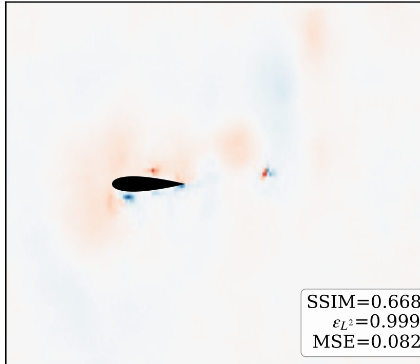
JEPA rollout
