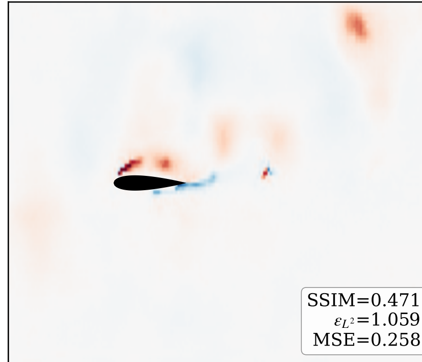
JEPA rollout
