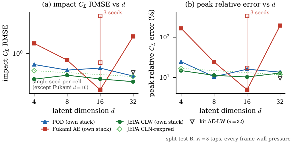
Figure 20. The assimilation-versus-dimension grid (in-distribution test set, own stacks, K = 8 , every-frame pressure; single seed per cell except the reconstructive d = 16 cell, which carries three): impact error and relative peak error against dimension for the three families. The predictive family is uniform, the linear basis stable, the reconstructive baseline erratic in dimension and in seed.
