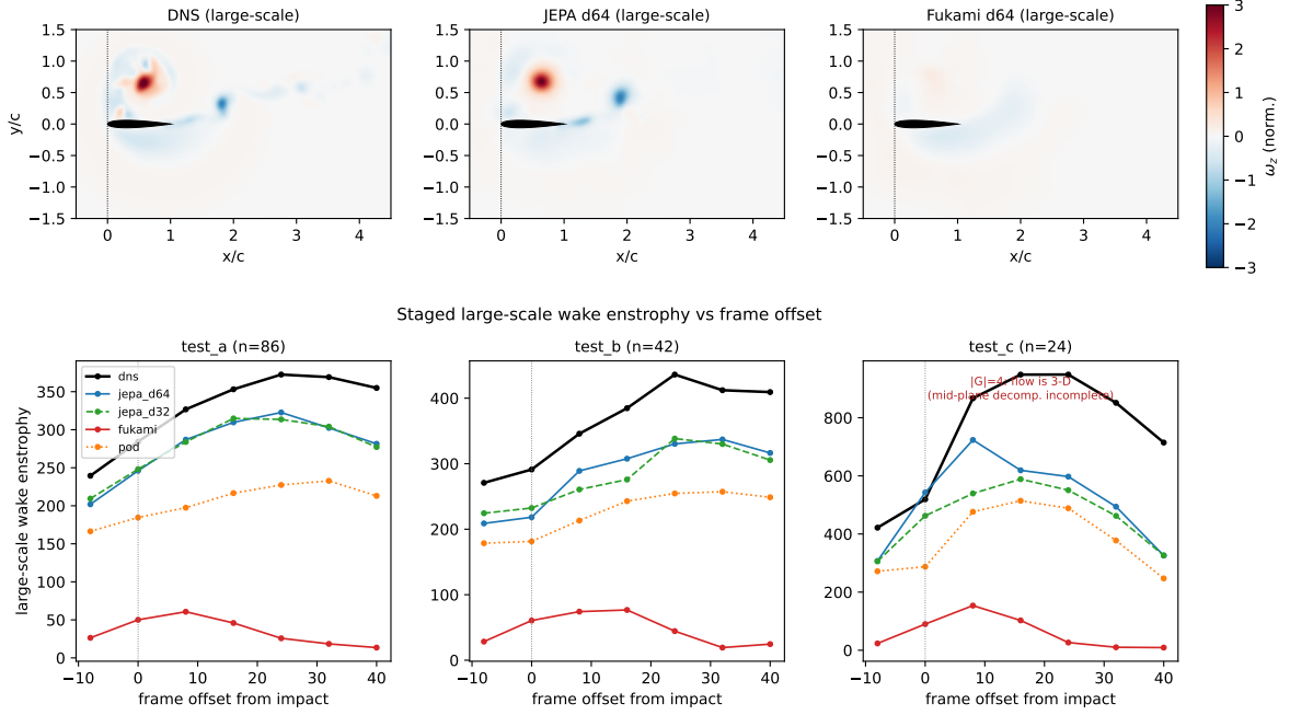
Figure 9: Gaussian scale decomposition ( \sigma/c = 0.05 ) of the held-out reconstructions. Top: large-scale vorticity for the simulation, the predictive decode, and the reconstructive autoencoder at H = 16 ; the predictive latent retains the leading-edge vortex and shear layer the reconstructive one smooths away. Bottom: large-scale wake enstrophy through the staged encounter for the simulation, predictive, and reconstructive fields, on each split.
