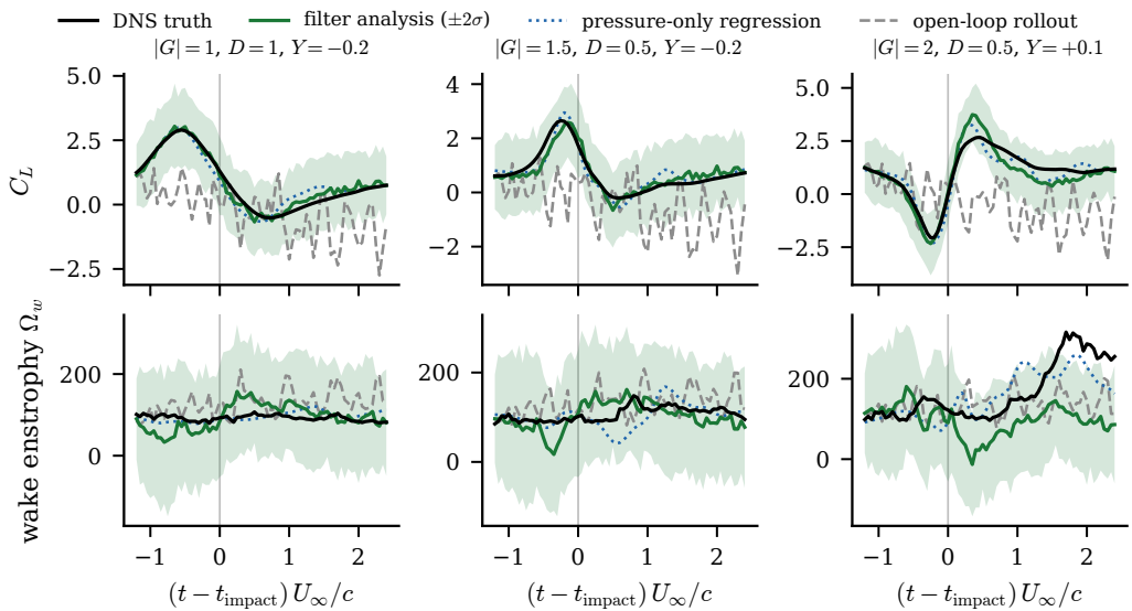
Figure 12. The estimator tracks the encounter from wall pressure alone. Columns are representative held-out encounters at |G| = 1, 1.5 and 2 ; rows are the lift coefficient and the wake enstrophy. Each panel shows the DNS truth, the filter analysis with its \pm 2\sigma ensemble band, the pressure-only regression, and the open-loop rollout; the vertical line marks impact. The filter follows the load through impact and relaxation where the open-loop forecast loses it and the pressure-only regression goes stale.
