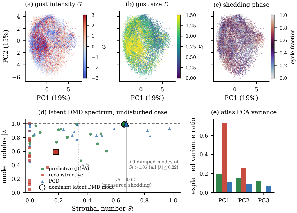
Figure 8. The physics the latent state holds. Top: two-dimensional projections of the predictive coefficient latent coloured by gust strength, core diameter, and shedding phase, showing a parametric manifold that coheres with the release parameters. Bottom: the latent dynamic-mode-decomposition spectrum, modulus against Strouhal number, by family; the predictive and linear latents place a marginally stable mode at the measured shedding frequency while the Fukami-lineage reconstruction is damped and off-frequency.
