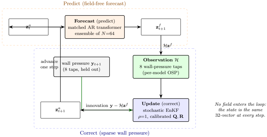
Figure 4. The pressure-only predict-correct estimator in the latent space. An ensemble of 64 members is advanced field free (predict), then corrected from 8 span-averaged wall-pressure taps (correct); the innovation is the difference between the measured observation and the observation predicted from the forecast state, in tap space for the base filter of §3.3.1 and in encoded latent space for the filters of §3.3.2 and §3.3.3. No vorticity field enters the loop and the lift and wake probes never enter the innovation. The state is the same 32-vector at every step.
