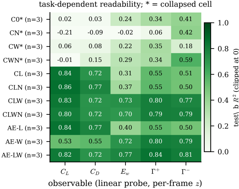
Figure 20. Task-dependent readability (in-distribution test set, linear probes on the per-frame state, seed mean over three encoder seeds per cell): lift and drag follow the L head, the wake block ( E_w , \Gamma^\pm ) follows the W head or the reconstruction objective, and collapsed cells (asterisks) read nothing linearly.
