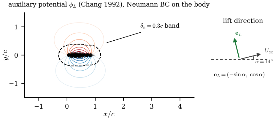
Figure 21. The Chang auxiliary potential \phi_L of equation (3.1) on the cache grid (contours), the feathered \delta_n = 0.3c supervision band (dashed) and the airfoil footprint; the inset shows the lift direction \mathbf{e}_L against the inclined freestream at \alpha = 14^\circ .
