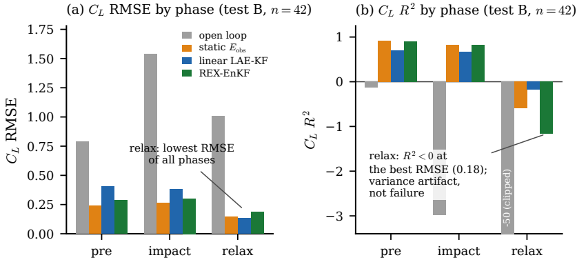
Figure 15. Phase-resolved lift tracking on the in-distribution test set ( n = 42 encounters, K = 8 taps, delay 10, N = 64 members, every-frame pressure). Lift error per phase in physical units (a) and in R^2 (b) at the val-calibrated band: the relaxation R^2 collapse is a variance artifact, the physical error the honest phase metric. The estimator ladder, its noise calibration and the fixed-lag smoother are in appendix C (figure 29).
