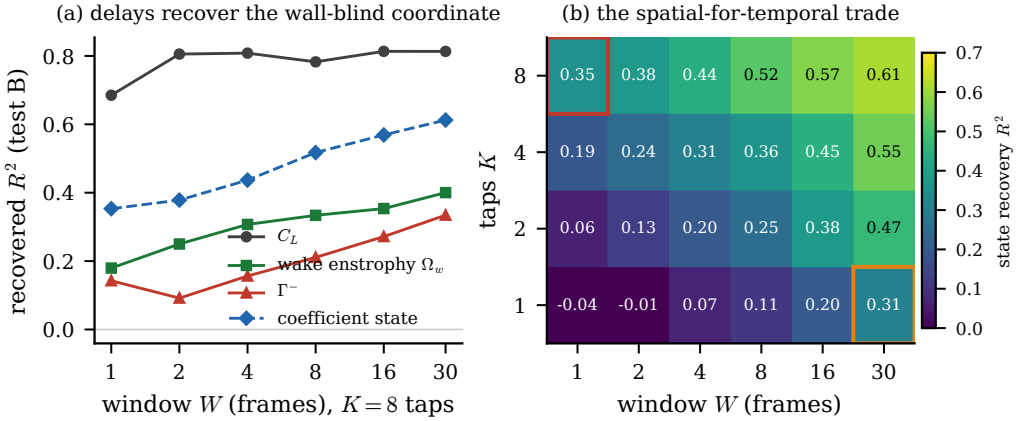
Figure 11. Sensors traded for delays. (a) Recovery of each observable from eight wall-pressure taps against the length of the pressure window (in-distribution test set); the wall-blind wake circulation rises with the window while the force, visible at one instant, does not. (b) Coefficient-state recovery over the tap-count by window-length grid, with the single-tap, thirty-frame cell and the reference eight-tap, single-frame cell outlined: a long window with few taps matches a short window with many.
