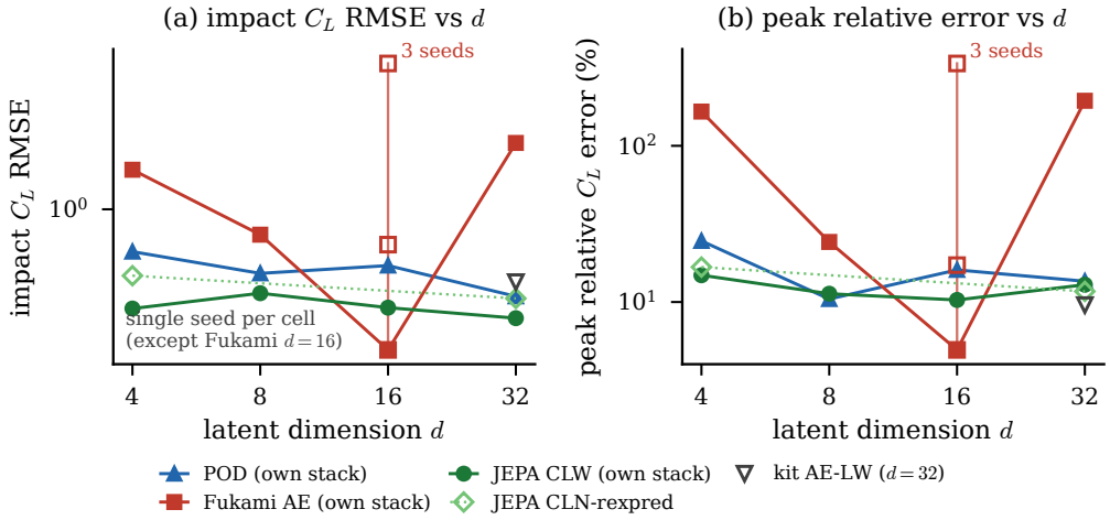
Figure 16. The assimilation-versus-dimension grid (in-distribution test set, per-family end-to-end stacks, K = 8 , every-frame pressure; single seed per cell except the reconstructive d = 16 cell, which carries three): impact error and relative peak error against dimension for the three families. The predictive family is uniform, the linear basis stable, the reconstructive baseline non-monotonic in dimension and irreproducible across seeds.
