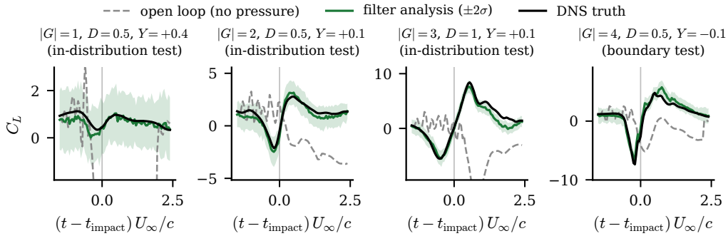
Figure 13. C_L estimation before and after impact across the gust-intensity envelope, on the wake-supervised predictive state ( d = 32 ) under the two-stage filter of §3.3.3: inside the impact window the members are advanced by the direct multi-horizon forecaster’s median forecast with its quantile band as state-dependent process noise (production scale c = 1.77 , validation-calibrated) and corrected by the encoded pressure observation; outside it, by the matched transformer with the tap-space update. Eight wall-pressure taps, N = 64 members; the lift probe that produces the plotted read-out never enters the innovation. Band: \pm 2 ensemble standard deviations; grey, the same stage-scheduled forecast models rolled deterministically without pressure. One representative encounter per |G| stratum (median impact closure on the frozen two-stage filter records; in-distribution test set for |G| \leq 3 , boundary test set at |G| = 4 , where this filter posts no large-error encounter). The analysis tracks the lift through impact and relaxation at every intensity; the open loop loses the transient.
