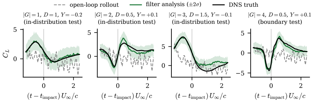
Figure 15. C_L estimation before and after impact across the gust-intensity envelope. DNS truth, frozen-filter analysis (band: \pm 2 ensemble standard deviations) and open-loop rollout for one representative encounter per |G| stratum (median-rule pick on the frozen envelope records; in-distribution test set for |G| \leq 3 , boundary test set at |G| = 4 ; the full per-stratum statistics are in table 10). The analysis tracks the lift through impact and relaxation at every intensity while the open loop reverts to the shedding cycle.
