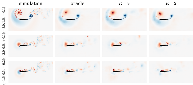
(b) flow recovery from sparse wall pressure
