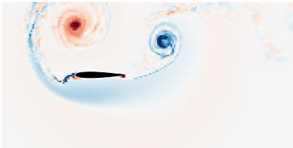
simulation
