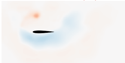
reconstructive (AE)
