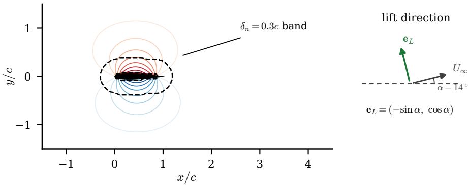
Figure 22. The Chang auxiliary potential \phi_L of equation (3.2) on the cache grid (contours), the feathered \delta_n = 0.3c supervision band (dashed) and the airfoil footprint; the inset shows the lift direction \mathbf{e}_L against the inclined freestream at \alpha = 14^\circ .
