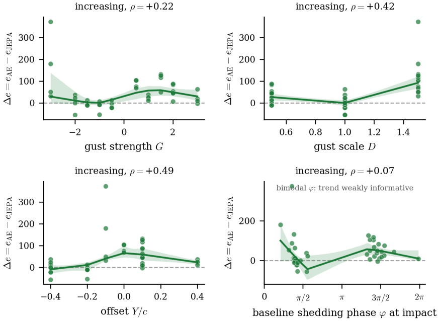
Figure 8. Per-encounter paired improvement \Delta e = e_{AE} - e_{JEPA} in held-out wake-entropy error against the gust strength G , core diameter D , wall-normal offset Y , and the baseline shedding phase at impact \phi (test_b, n = 42 ); positive \Delta e means the predictive latent carries the smaller error. Each panel shows the per-encounter values, a locally weighted (LOWESS) trend, and a bootstrap band over encounters. The predictive advantage grows with D and toward off-midplane Y ; the shedding-phase axis falls into two clusters because impact is fixed near a single convective instant.
