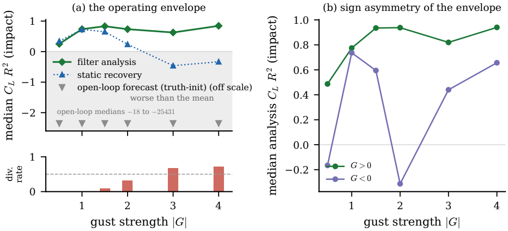
Figure 12. The gust-intensity operating envelope, diagnosed with the base frozen filter (figure 13 carries the forecast-noise filter’s phase-resolved errors). (a) Median analysis lift closure ( R^2 , impact window) against gust strength for the base filter, the static single-frame recovery, and the truth-initialised open-loop forecast, with the filter consistency-failure rate as the strip beneath; the shaded band marks closure worse than predicting the encounter mean, and the open-loop forecast lies off the scale below it. The base filter tracks the median throughout but becomes under-dispersed from a gust ratio of about three, where the consistency-failure rate climbs. (b) The same base-filter closure resolved by the physical sign of the gust, showing the wider usable envelope of the positive gusts.
