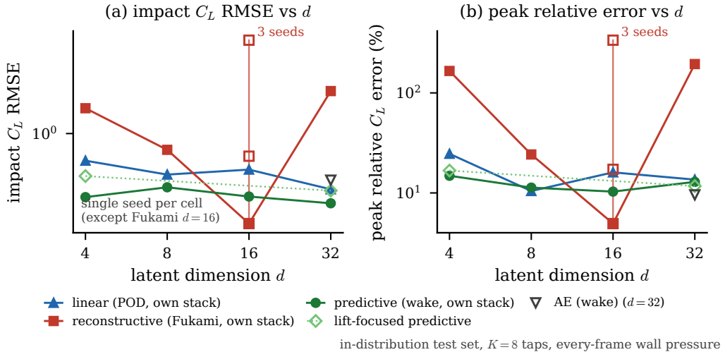
Figure 14. The assimilation-versus-dimension grid (in-distribution test set, per-family end-to-end stacks, K = 8 , every-frame pressure; single seed per cell except the reconstructive d = 16 cell, which carries three): impact error and relative peak error against dimension for the three families. The predictive family is uniform, the linear basis stable, the reconstructive baseline non-monotonic in dimension and irreproducible across seeds.
