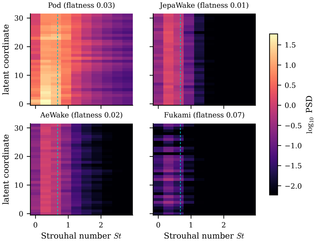
Figure 10. Per-coordinate latent spectra by family (training encounters, d = 32 ; mean Welch power spectral density against Strouhal number, coordinates ordered by peak frequency; the dashed line marks the shedding Strouhal). The predictive coordinates concentrate at the shedding line while the published-recipe reconstruction spreads energy across frequency, and the matched-supervision autoencoder does not.
