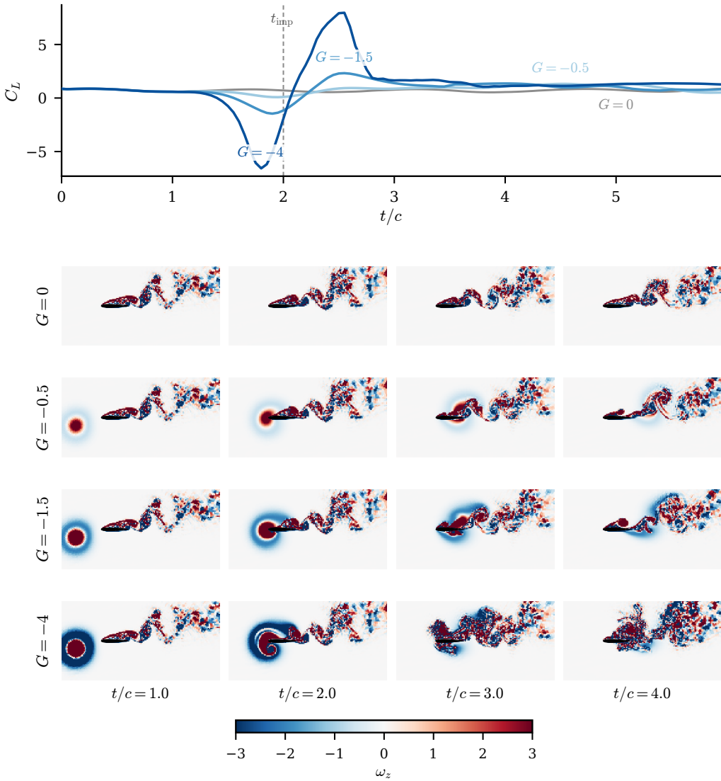
Figure 2. The vortex gust as a wake-reorganisation event: a gust-strength sweep at fixed core diameter D = 0.5 and offset Y = -0.1 (first encounter of each case). Top: lift coefficient C_L against convective time, with t/c = 0 the release and t_{\text{imp}} (dashed) the leading-edge crossing near t/c = 2 ; the load excursion deepens and widens with |G| , the baseline ( G = 0 ) in grey. Bottom: mid-plane spanwise vorticity \omega_z per case (rows G = 0, -0.5, -1.5, -4 ) at four times (columns t/c = 1, 2, 3, 4 ), raw units, colourbar clipped at \pm 3 (intense cores saturate), airfoil filled. The strong gust reorganises the wake through impact while the weak cases barely perturb the shedding; G = -4 is the |G| = 4 extrapolation case, shown only for illustration. The release parameters alone do not fix where the wake sits afterwards, which is why the wake, not only C_L , is the endpoint a reduced state must carry.
