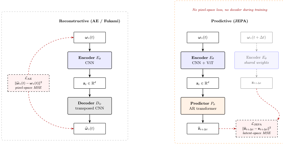
Figure 12. Predictive versus reconstructive training. Left: the reconstructive autoencoder encodes the field at t , decodes it, and incurs a field-space error. Right: the predictive model encodes the fields at t and t + \Delta t with shared weights and incurs a latent-space error between the predicted and observed target embeddings, with no field-space loss and no decoder during training. This is the contrast the matched-predictor protocol of §3.2 evaluates; the visualisation decoder is trained only afterwards, on the frozen encoder.
