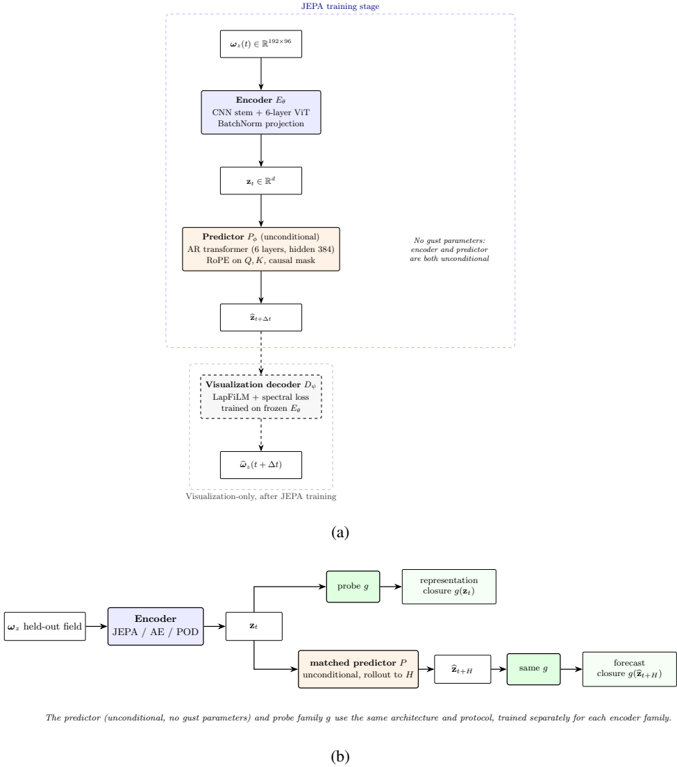
Figure 2. The predictive model and how it is evaluated. (a) The encoder maps the mid-plane vorticity field to a latent \mathbf{z}_t , and the autoregressive predictor advances the latent from its own history; no gust parameters enter the encoder or the predictor. The two auxiliary observable heads (lift and wake) read \mathbf{z}_t during JEPa training with small weights and are not part of the latent-prediction loss; they are omitted from the schematic for clarity. The visualisation decoder is trained only after the encoder is frozen and is used solely for the diagnostic decodes of §4.6, never in the predictive loss. (b) Evaluation applies the same predictor and probe family g to every encoder family: a probe on the simulation-encoded latent measures representational closure, the headline, and the same probe on the rolled-out latent \hat{\mathbf{z}}_{t+H} measures forecast closure, reported as secondary.
