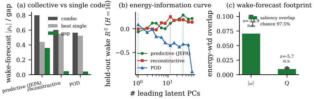
Figure 11. The wake is a distributed latent code, on test_b. Left: the gap between the held-out wake readability of the full latent and that of its single most informative coordinate, by family; the predictive (JEPA) latent shows a large gap (0.36) where the reconstructive (Fukami, 0.05) and linear (POD, 0.04) latents do not, so no single predictive coordinate carries the wake. Centre: the held-out wake skill versus the number of leading principal components, which knees at about 32 components for the predictive latent against 12 and 1 for the baselines. Right: the gradient-saliency footprint of the wake-forecast direction overlaps the high-vorticity cores and Q-criterion vortices below the permutation chance band, so the distributed code is not spatially localised. Observational probes on the frozen encoders.
