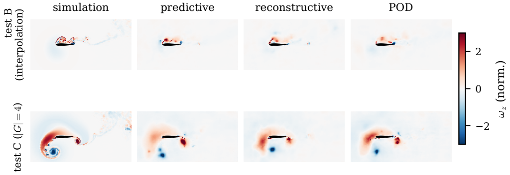
Figure 18. Decoded vorticity at the impact frame on held-out encounters (rows: an interpolation test_b encounter and a |G| = 4 test_c encounter) for the simulation and the predictive, reconstructive, and POD decodes (columns). The predictive decoder is blurry by design but localises the impingement; the reconstructive autoencoder collapses toward a near-uniform field on the held-out interpolation condition, while the linear basis is amplitude-accurate. All families degrade in the |G| = 4 regime, reported as the observability boundary of §2.1 rather than as a generalisation claim. Field-space similarity is read only as a labelled decode ceiling (§4.6).
