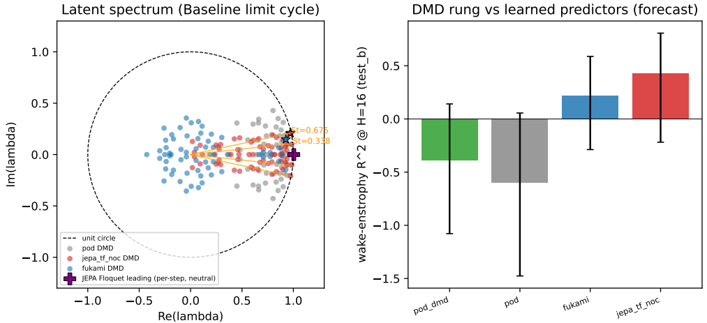
Figure 8. The latent dynamics carry the shedding spectrum but are not a linear operator. Left: dynamic-mode-decomposition eigenvalues of the encoded limit-cycle trajectory in the complex plane, by family, against the unit circle and the measured shedding-frequency ray; the predictive (JEPA) and linear (POD) latents place a marginally stable oscillatory pair at the shedding Strouhal number (0.66 and 0.68, moduli 0.991 and 0.996) while the reconstructive (Fukami) pair is damped and off-frequency (0.50). Right: the wake-entropy forecast skill of a best-fit linear operator on the linear basis (dynamic mode decomposition as a forecaster, -0.39 ) against the learned predictor (0.43), a margin of 0.82.
