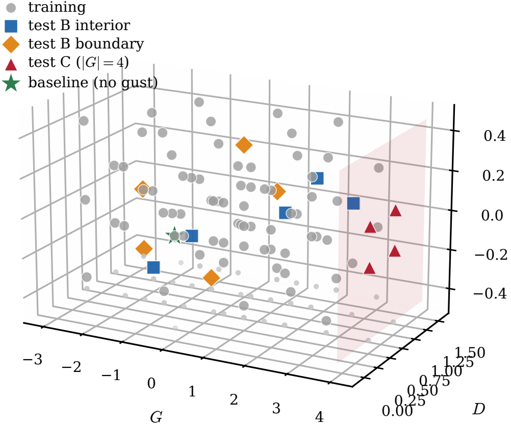
Figure 2. Parameter-space sampling of the 85 cases in the (G, D, Y) gust envelope, shown as one isometric view and coloured by split: training (229 encounters), the stratified in-distribution test set (test_b, 42 encounters, split into interior and boundary tiers), and the out-of-distribution extrapolation set (test_c, 24 encounters). The translucent plane marks the |G| = 4 extrapolation boundary and the grey points on the floor are the projection of every case, which shows that training mass concentrates near Y/c = 0 , the reason the wall-normal offset is the least well resolved parameter (§4.6).
