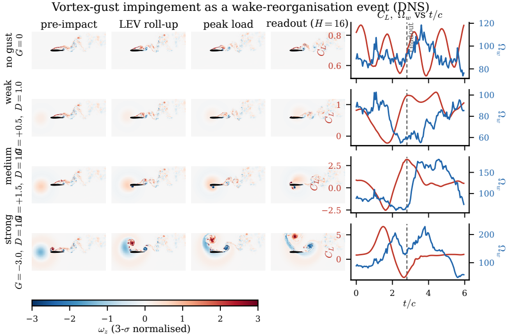
Figure 1. The vortex gust as a wake-reorganisation event, shown on four representative encounters (rows) from the no-gust limit cycle to a strong gust. The first four columns are the mid-plane spanwise vorticity \omega_z at four stages of the encounter, fixed on a common frame timeline so the columns read as one shared clock: pre-impact, leading-edge-vortex roll-up, peak load, and the readout instant H = 16 frames after impact at which every representation is later probed. The field is shown on the 3- \sigma normalised scale with the airfoil as a filled polygon. The right column overlays the lift coefficient C_L and the mid-plane wake enstrophy \Omega_w against convective time t/c , with the dashed line at the readout instant; the load spike and the wake-enstrophy excursion are the surface and field signatures of the same roll-up and shedding event, and the release parameters alone do not fix where the wake sits at readout. The cases are typical interior encounters chosen for clarity, not the largest excursions in the set.
