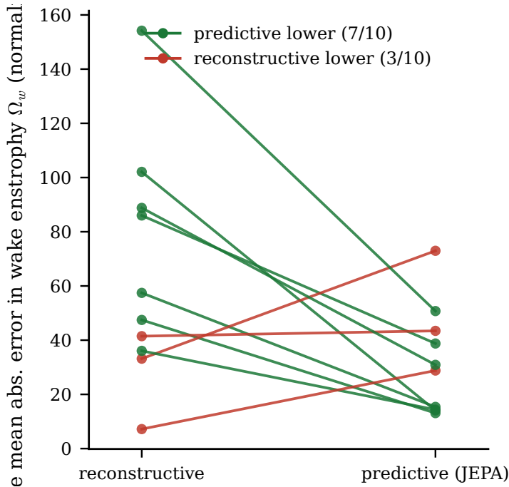
Figure 5. Per-case wake-entropy closure, the honest case-level view of the headline result. Each line is one held-out test_b case (ten in all), connecting the reconstructive autoencoder’s per-case mean absolute error (left) to the predictive latent’s (right) at H = 16 ; a downward line favours the predictive latent. The predictive latent gives the lower error on seven of the ten cases (median per-case improvement positive, case-level signed-rank significant), with three cases favouring the reconstructive baseline: the advantage is real at the case level but not uniform, which is why the case-level multiplicity correction is not passed and the claim is stated at encounter level with this spread shown.
