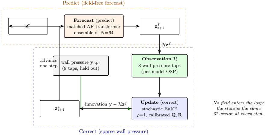
Figure 5. The leakage-free predict-correct estimator in the latent space. An ensemble of 64 members is advanced field free (predict), then corrected from 8 span-averaged wall-pressure taps (correct); the innovation is the difference between the measured observation and the observation predicted from the forecast state, in tap space for the base filter of §3.3.1 and in encoded latent space for the filters of §3.3.2 and §3.3.3. No vorticity field enters the loop and the lift and wake probes never enter the innovation. The state is the same 32-vector at every step.
