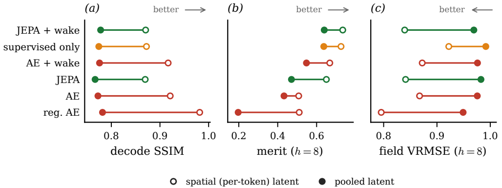
Figure 25. The decodability-versus-estimability trade of §5.3, quantified. Each panel connects the spatially resolved latent (open marker) to its pooled coefficient state (filled marker), per family, for the decode similarity, the matched-predictor merit, and the field forecast error. Pooling costs field fidelity in every family; the coefficient state is the price of a state a wall-pressure filter can track.
