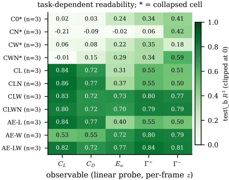
Figure 7. Task-dependent readability (test_b, linear probes on the per-frame state, seed mean over three encoder seeds per cell): lift and drag follow the L head, the wake block ( E_w , \Gamma^\pm ) follows the W head or the reconstruction objective, and collapsed cells (asterisks) read nothing linearly.
