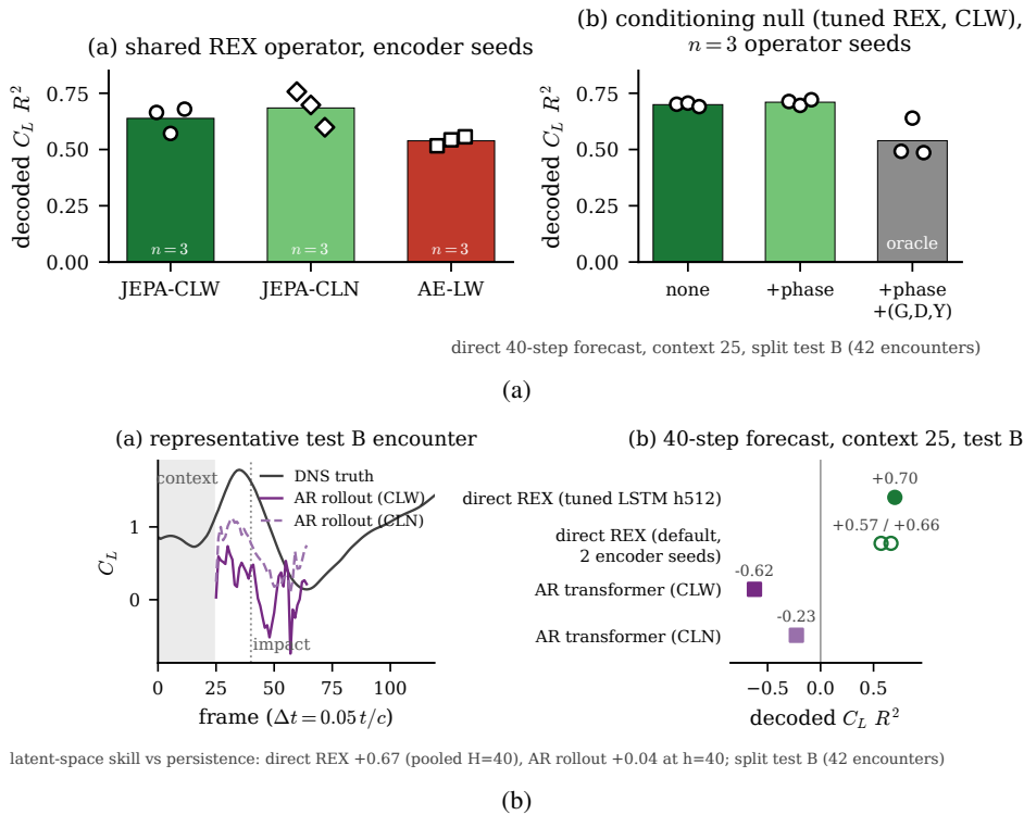
Figure 11. Forecasting the state on test_b. (a) Decoded lift R^2 of the shared direct forecaster per family (three operator seeds each, bars at the seed mean) and the conditioning null (three seeds per arm): the (G, D, Y) oracle degrades the forecast, the phase covariate is a wash. (b) Direct versus autoregressive over forty steps through the impact from a 25-frame context: the one-shot forecast stays usable where the rollout compounds.
