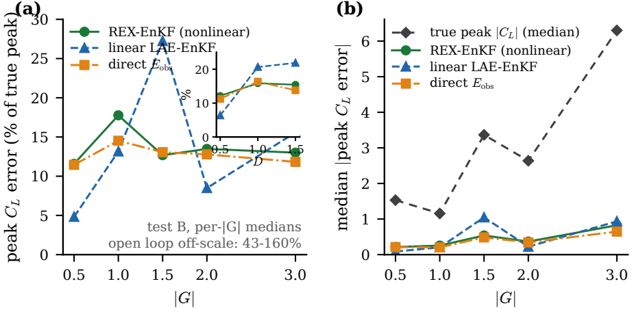
Figure 17. Relative peak error across the gust envelope (test_b, medians per |G| ): the forecast-derived filter is scale-invariant near 12 to 14 per cent while the linear filter is non-uniform; the absolute peak error (right) grows with the peak itself.
