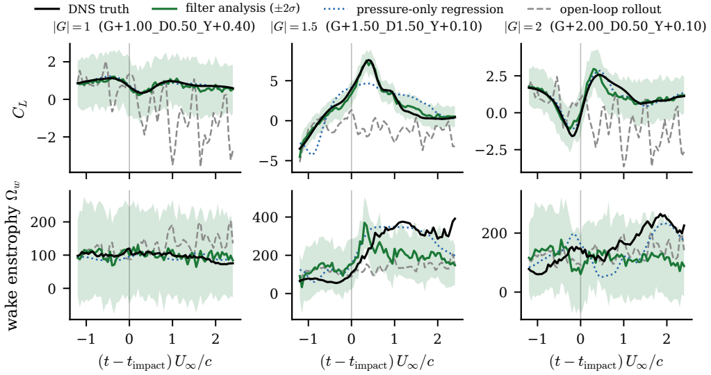
Figure 14. The estimator tracks the encounter from wall pressure alone. Columns are representative held-out encounters at |G| = 1, 1.5 and 2 ; rows are the lift coefficient and the wake enstrophy. Each panel shows the DNS truth, the filter analysis with its \pm 2\sigma ensemble band, the pressure-only regression, and the open-loop rollout; the vertical line marks impact. The filter follows the load through impact and relaxation where the open-loop forecast loses it and the pressure-only regression goes stale.
