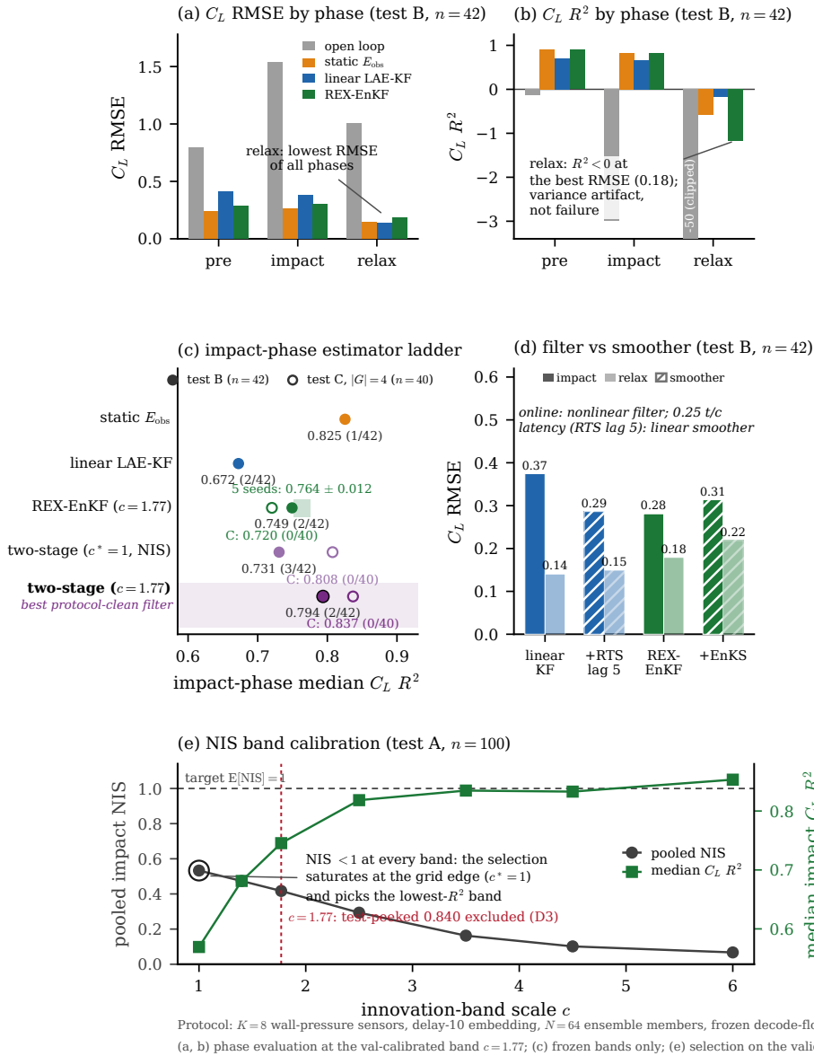
Figure 16. Phase-resolved assimilation on test_b ( n = 42 encounters, K = 8 taps, delay 10, N = 64 members, every-frame pressure). (a,b) Lift error per phase in physical units and in R^2 at the val-calibrated band: the relaxation R^2 collapse is a variance artifact. (c) The impact-phase estimator ladder with the five-seed member-noise band; open markers are the frozen test_c values. (d) Filter against fixed-lag smoother. (e) The band-scale calibration on the held-out training encounters: consistency and tracking disagree, and the selection saturates at the grid edge.
