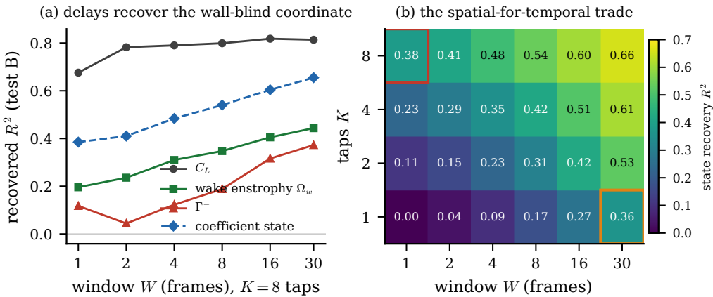
Figure 13. Sensors traded for delays. (a) Recovery of each observable from eight wall-pressure taps against the length of the pressure window (test_b); the wall-blind wake circulation rises with the window while the force, visible at one instant, does not. (b) Coefficient-state recovery over the tap-count by window-length grid, with the single-tap, thirty-frame cell and the reference eight-tap, single-frame cell outlined: a long window with few taps matches a short window with many.
