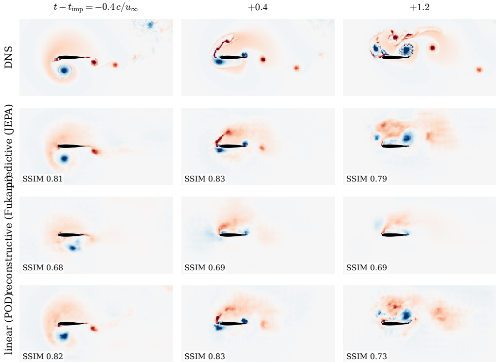
Figure 24. Decoded vorticity through the encounter on the representative held-out test_b case ( |G| = 1.5 , the same encounter as figure 14). Rows: the simulation and the fields decoded from the encoded coefficient state of the predictive, reconstructive, and linear families; columns: a pre-impact, an impact, and a relaxation frame. Each decode is produced by the same diagnostic decoder that defines the decode-floor similarity of table 6, trained on the frozen encoder; the per-panel structural similarity is annotated. The pooled decode is soft by construction (§5.3); the comparison is between rows at matched frames, and no family's decode is part of any training loss.
