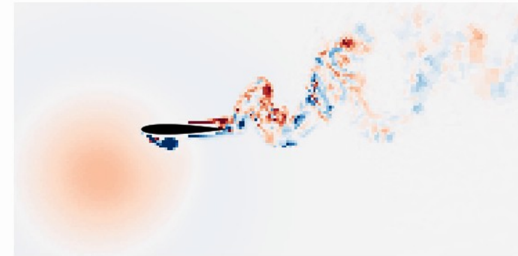
Gust encounter ( G=+2.0 , D=1.5 , Y=-0.4 ): t/c = -0.60
