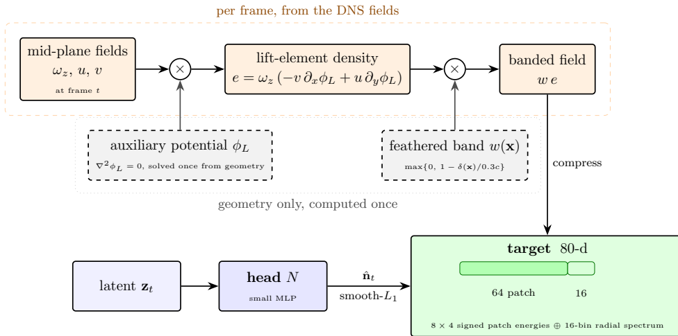
Figure 5. [S31-C1] The near-body supervision head. Along the top, the per-frame path that builds the target from the DNS fields: the mid-plane vorticity and velocity are weighted by the auxiliary potential \phi_L to give the lift-element density e , which is restricted to the feathered near-body band w and compressed to 80 dimensions. The potential and the band, drawn on the lower branch, depend on the geometry alone and are computed once; neither carries time or flow state. Below, the trained part: the head reads the latent \mathbf{z}_t and is fit to that target under a smooth- L_1 loss. The encoder never sees e itself, and this loss is not part of the latent-prediction objective. The 64 + 16 split of the target, 8 \times 4 signed patch energies followed by a 16-bin radial spectrum, is the identical construction used for the wake target of §3.1, which is what makes the two field observables byte-matched in capacity.
