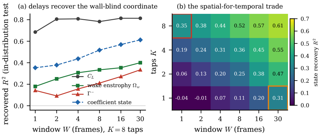
Figure 12. [S4-C3] Sensors traded for delays. (a) Recovery of each observable from eight wall-pressure taps against the length of the pressure window (in-distribution test set); the wall-blind wake circulation rises with the window while the force, visible at one instant, does not. (b) Coefficient-state recovery over the tap-count by window-length grid, with the single-tap, thirty-frame cell and the reference eight-tap, single-frame cell outlined: a long window with few taps matches a short window with many.
