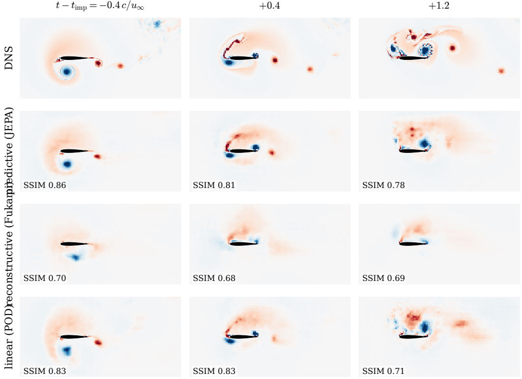
Figure S1. Decoded vorticity through the encounter on the representative held-out in-distribution test case ( |G| = 1.5 , the same encounter as figure 16). Rows: the simulation and the fields decoded from the encoded coefficient state of the predictive, reconstructive, and linear families; columns: a pre-impact, an impact, and a relaxation frame. Each decode is produced by the same diagnostic decoder that defines the decode-floor similarity of table 6, trained on the frozen encoder; the per-panel structural similarity is annotated. The pooled decode is soft by construction (§5.3); the comparison is between rows at matched frames, and no family's decode is part of any training loss.
