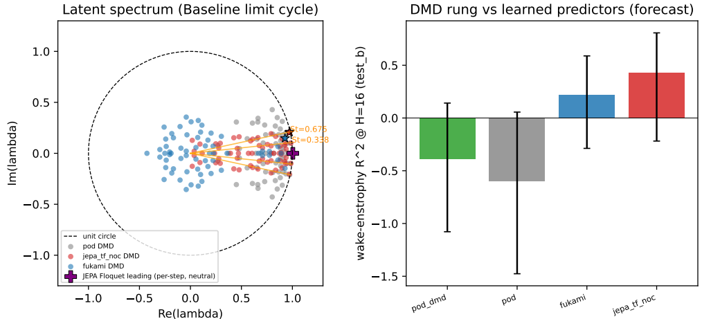
Figure 7. The latent dynamics carry the shedding spectrum but are not a linear operator. Left: dynamic-mode-decomposition eigenvalues of the encoded limit-cycle trajectory in the complex plane, by family, against the unit circle and the measured shedding-frequency ray; the predictive (JEPA) and linear (POD) latents place a marginally stable oscillatory pair at the shedding Strouhal number (0.66 and 0.68, moduli 0.991 and 0.996) while the reconstructive (Fukami) pair is damped and off-frequency (0.50). Right: the wake-entropy forecast skill of a best-fit linear operator on the linear basis (dynamic mode decomposition as a forecaster, -0.39 ) against the learned predictor (0.43), a margin of 0.82.
